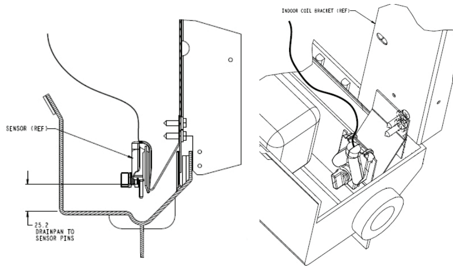
REFERENCE VIEWS
