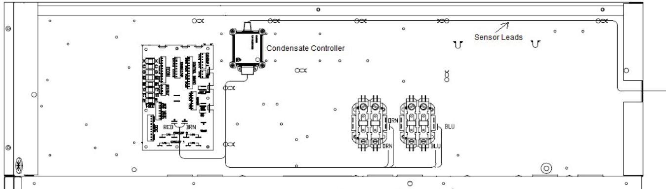
Fig. 1 — Control Box
