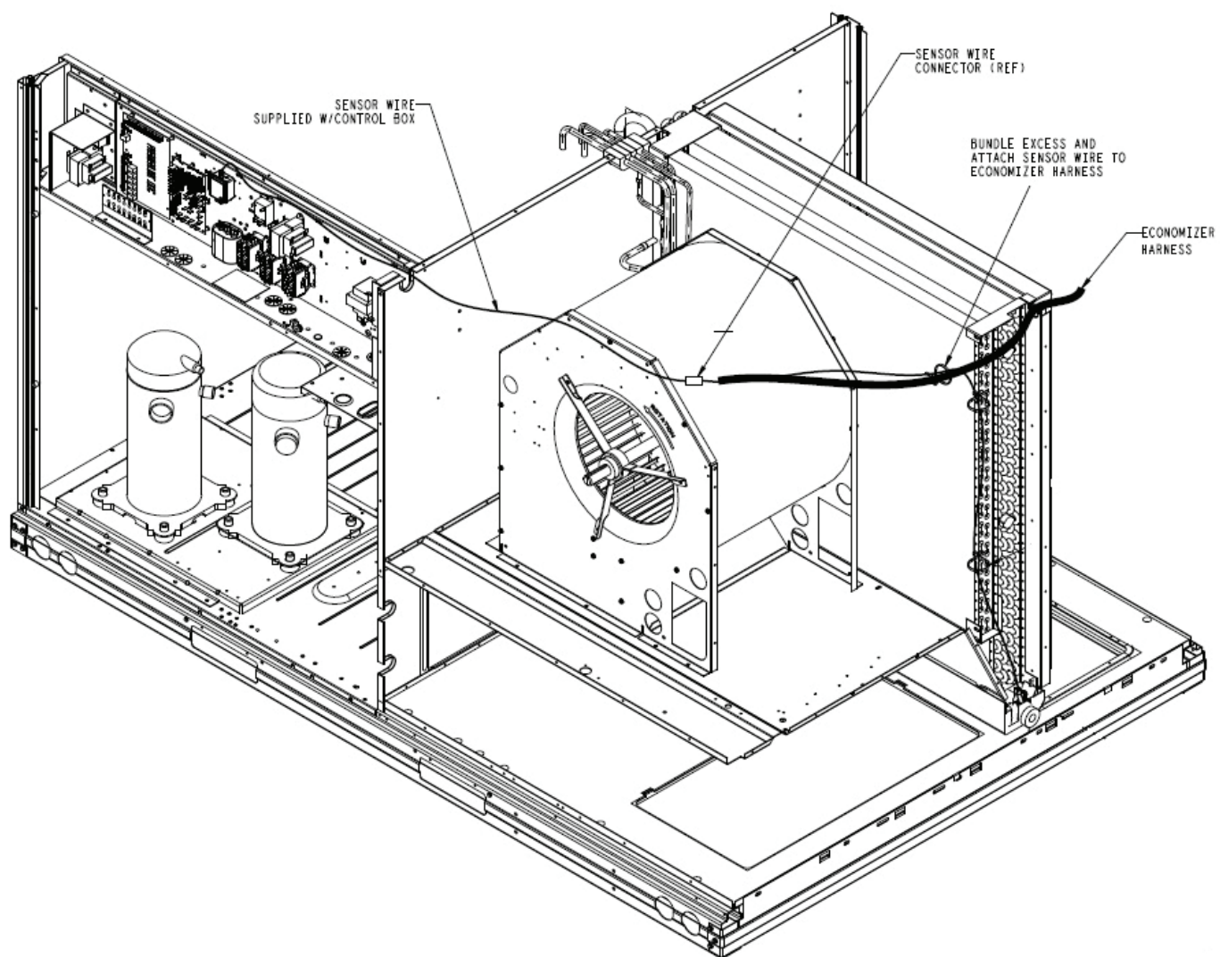
Fig. 5 — Sensor Wire Connection
