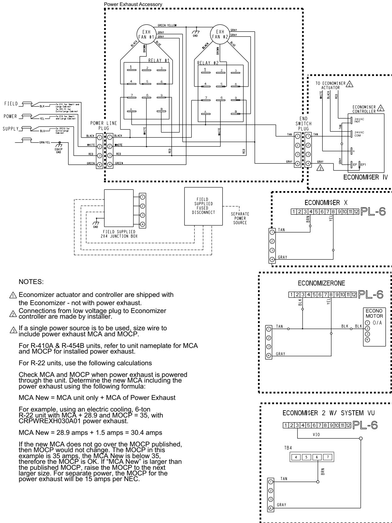
Fig. 7 — Dual Fan Power Exhaust Wiring for EconoMi$er IV, EconoMi$er X, EconomizerONE, and EconoMi$er 2 with SystemVu - 460 V Units
