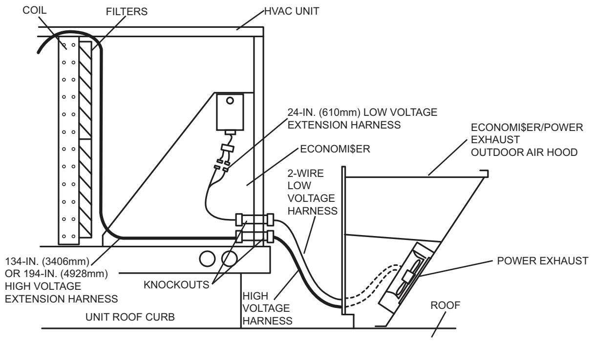
Fig. 5 — Power Exhaust Harness Installation for EconoMiSer X with W7220 Controller and EconomizerONE with POL 224 Controller
