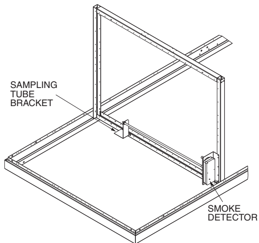
Fig. 5 — Smoke Detector for 48/50P030-050 Units (No Economizer or Power Exhaust)
