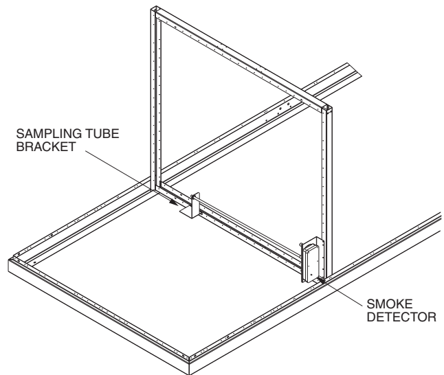
Fig. 8 — Smoke Detector for 48/50P055-100 Units (No Economizer or Power Exhaust)
