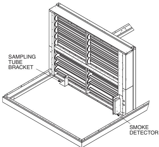
Fig. 6 — Smoke Detector for 48/50P030-050 Units (Economizer Only)
