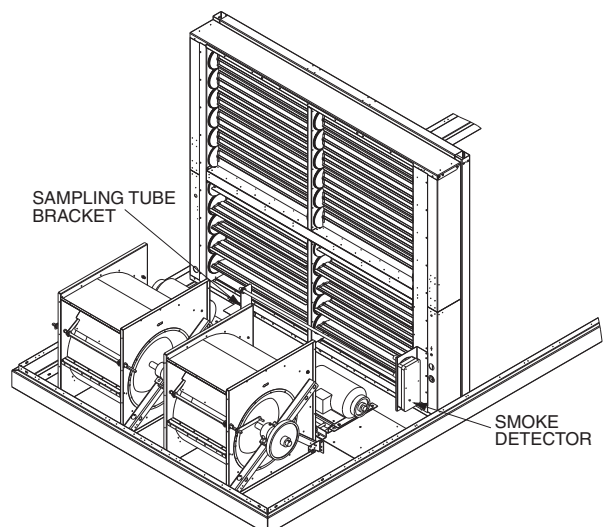
Fig. 10 — Smoke Detector for 48/50P055-100 Units (Economizer with Power Exhaust)
