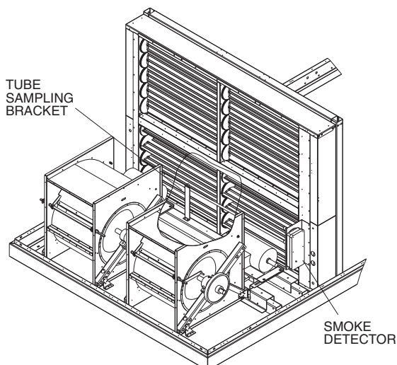
Fig. 7 — Smoke Detector for 48/50P030-050 Units (Economizer with Power Exhaust)
