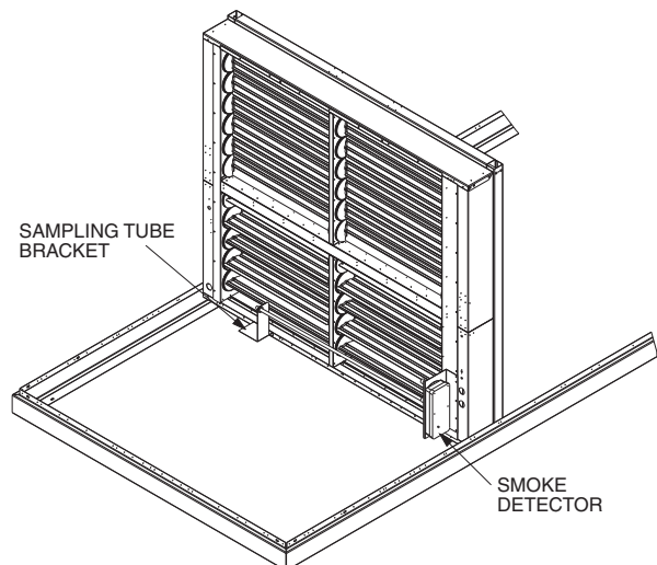
Fig. 9 — Smoke Detector for 48/50P055-100 Units (Economizer Only)
