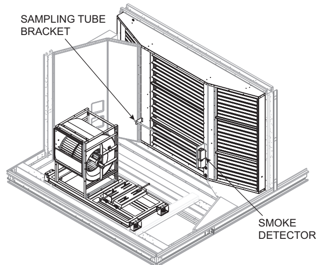
Fig. 11 — Smoke Detector for 48/50N Units
