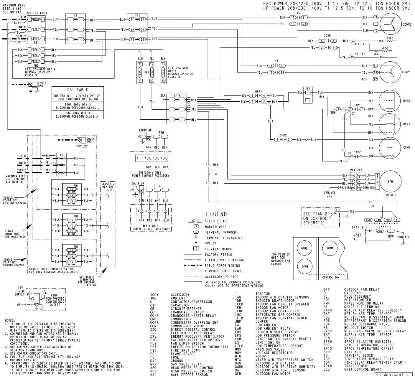
Fig. W — 50GC-*14 Power Wiring Diagram — 208/230, 460-3-60 Unit with SystemVu™ Control — High SCCR
