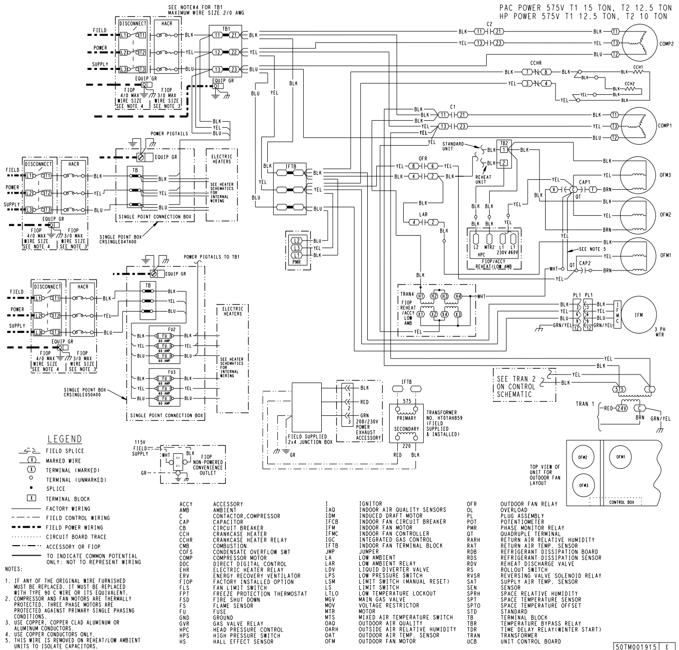
Fig. M — 50GC-14 Power Wiring Diagram — 575-3-60 Unit Electromechanical with POL224 Controller — Standard/Medium SCCR
