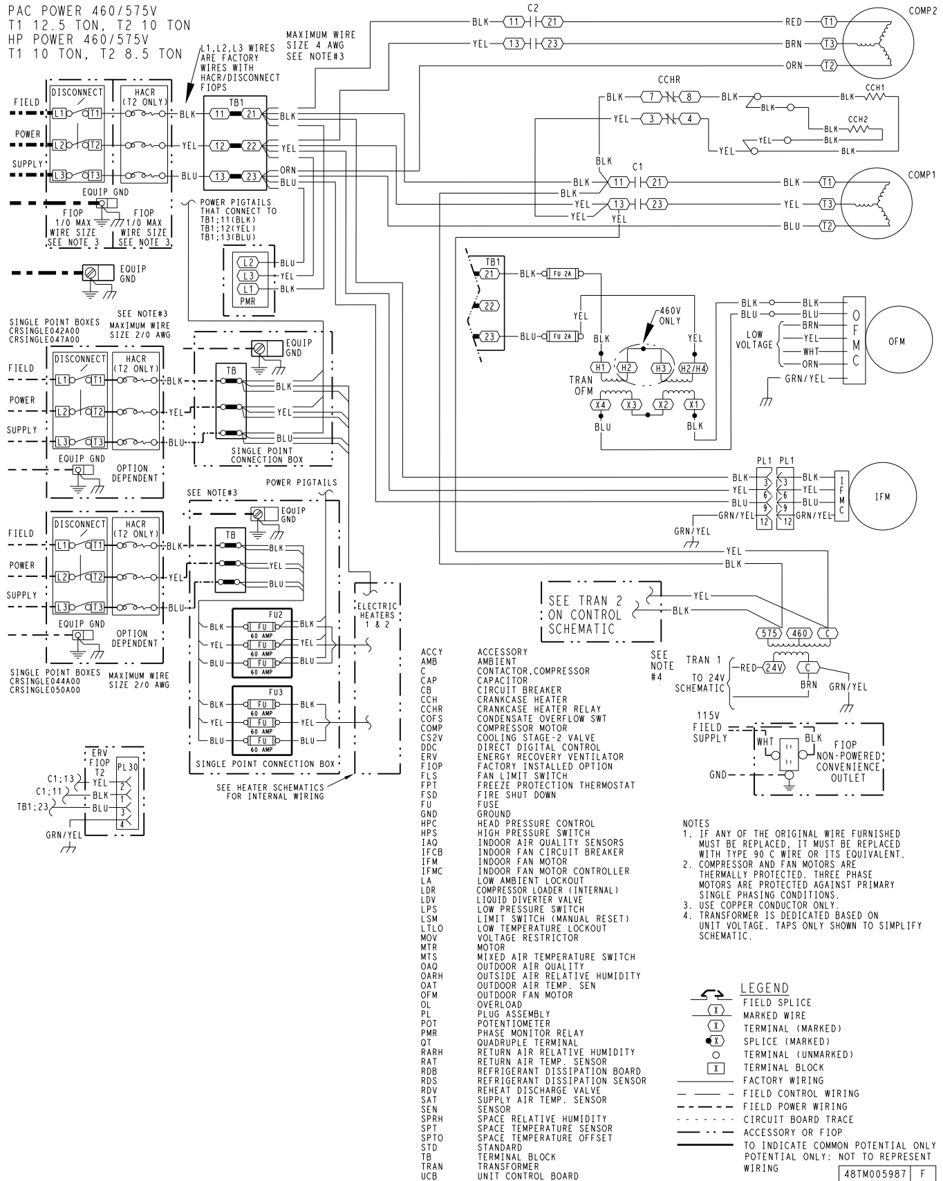
Fig. K — 50GC-*12 Power Wiring Diagram — 460, 575-3-60 Unit Electromechanical with POL224 Controller — Standard/Medium SCCR
