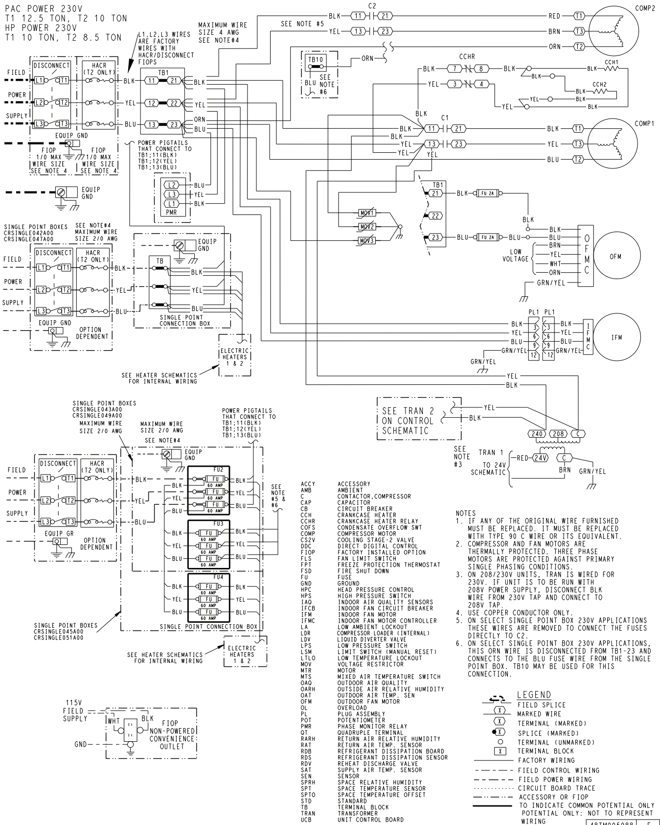
Fig. J — 50GC-*12 Power Wiring Diagram — 208/230-3-60 Unit Electromechanical with POL224 Controller — Standard/Medium SCCR
