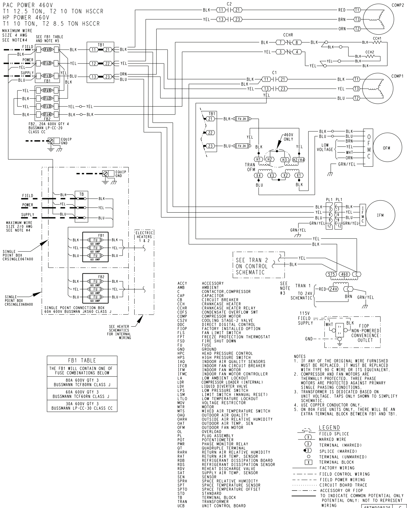
Fig. T — 50GC-*12 Control Wiring Diagram — 460-3-60 Unit Electromechanical with POL224 Controller — High SCCR
