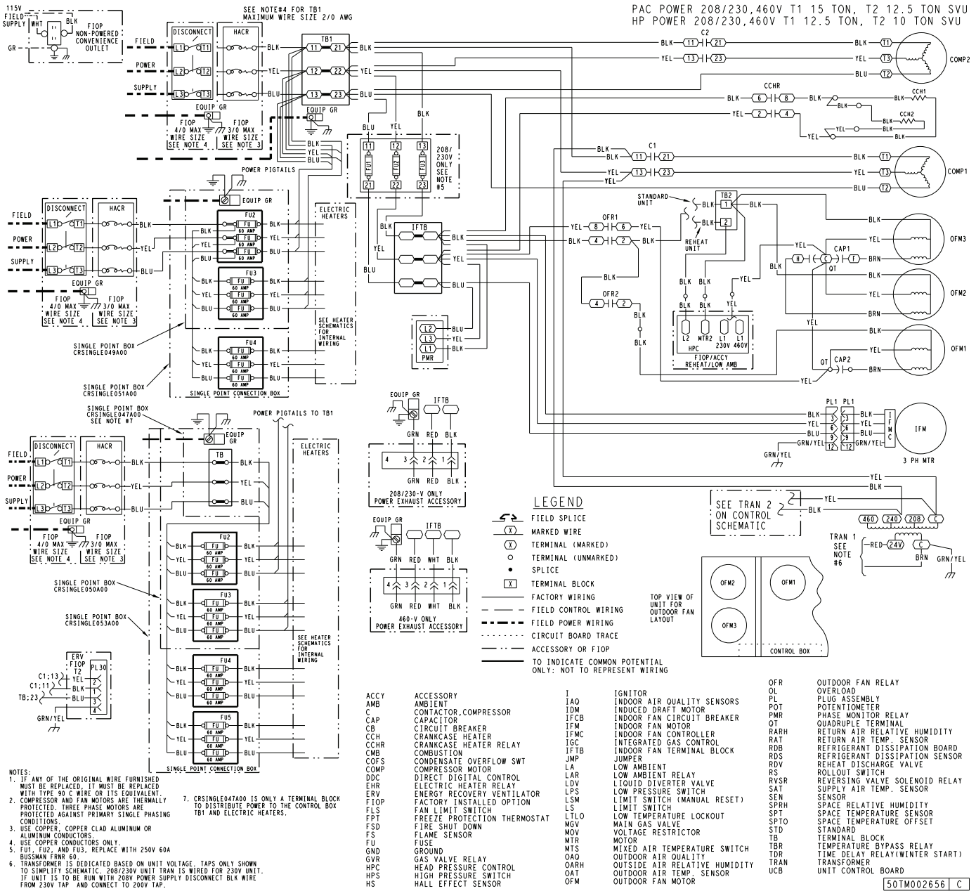
Fig. P – 50GC-*14 Power Wiring Diagram – 208/230, 460-3-60 Unit with SystemVu™ Control – Standard/Medium SCCR
