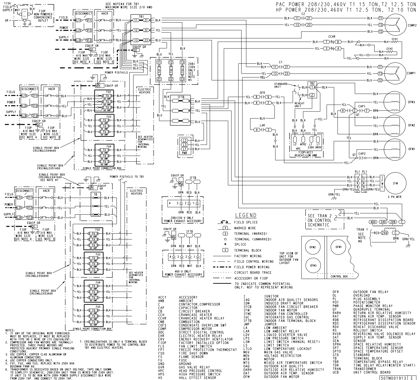
Fig. L — 50GC-*14 Power Wiring Diagram — 208/230, 460-3-60 Unit Electromechanical with POL224 Control — Standard/Medium SCCR
