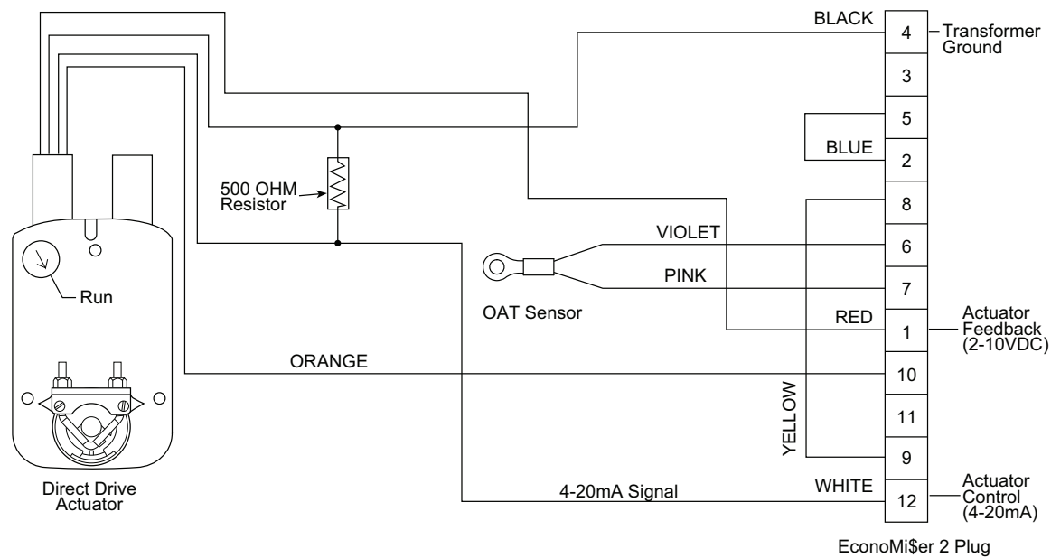
Fig. 56 — EconoMi$er2 with 4 mA to 20 mA Control Wiring
