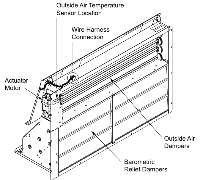
Fig. 54 — 50GC-*14 EconomizerONE Component Locations (CRECOMZR109A00 Shown)
