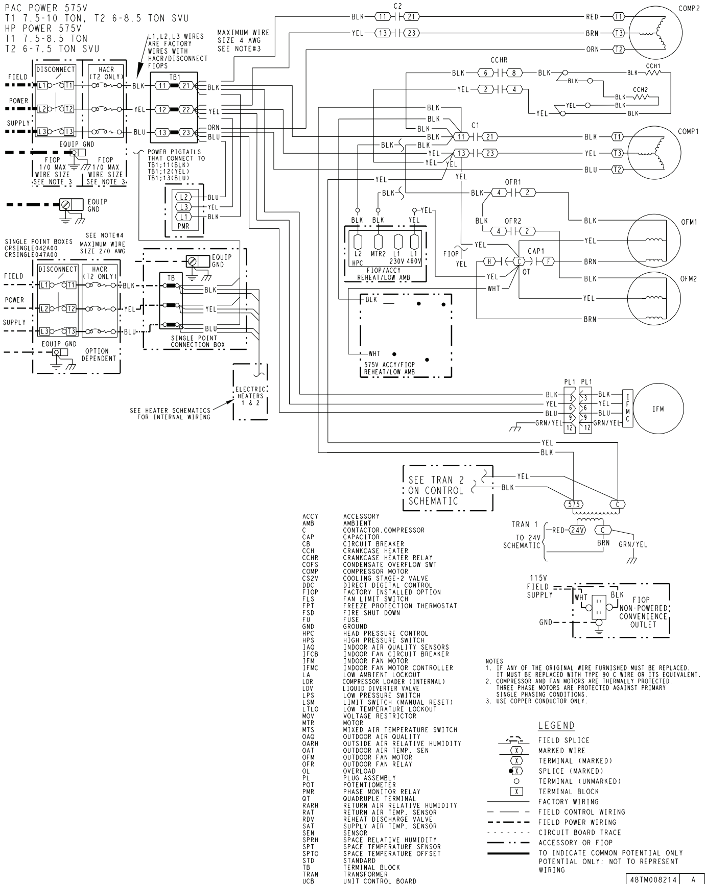
Fig. O — 50GC-*07-09 Power Wiring Diagram — 575-3-60 Unit with SystemVu™ Control — Standard/Medium SCCR
