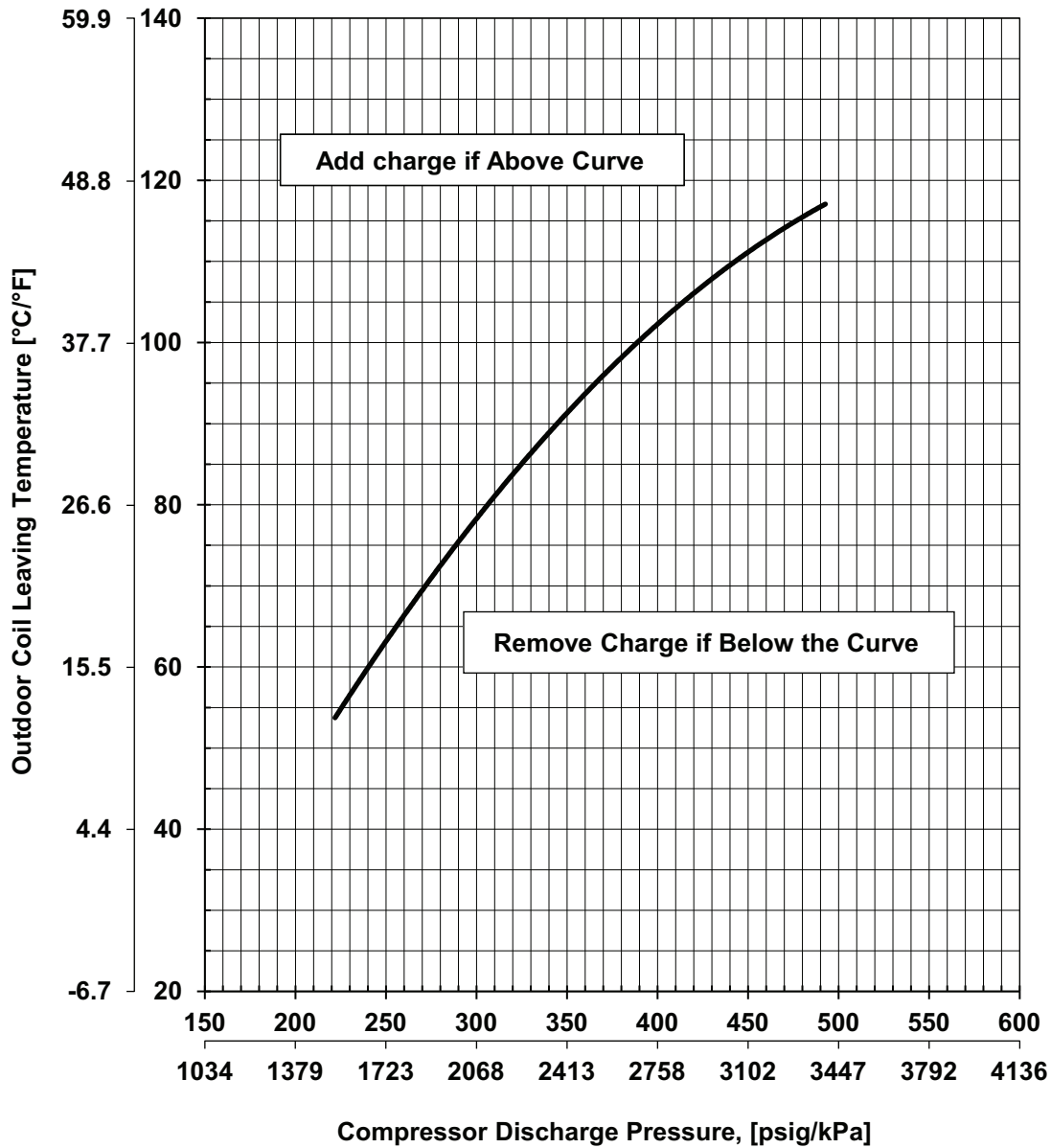
Fig. 26 — Cooling Charging Chart - 7.5 Ton
