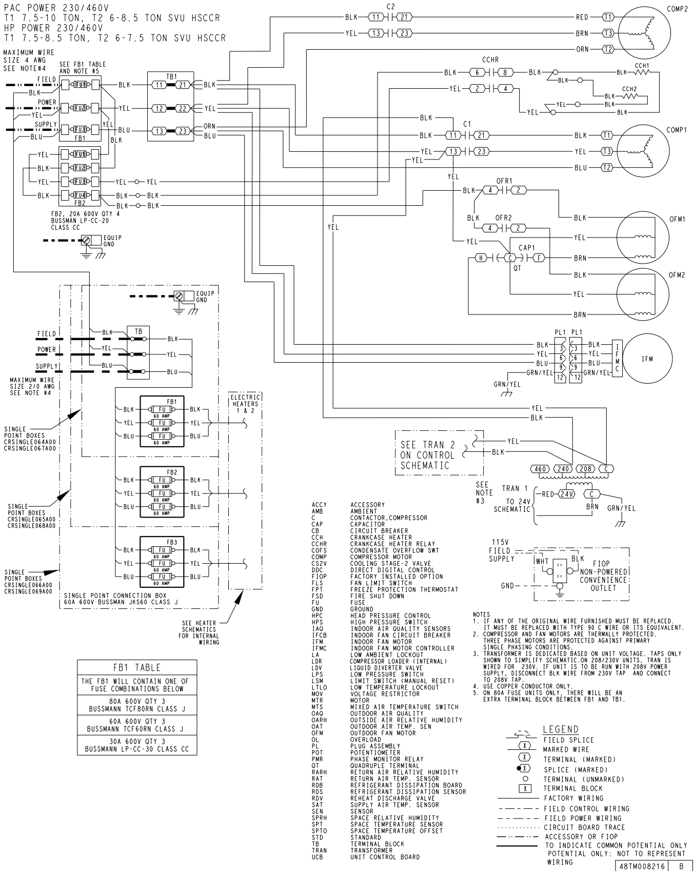
Fig. V — 50GC-*07-09 Power Wiring Diagram — 208/230, 460-3-60 Unit with SystemVu™ Control — High SCCR
