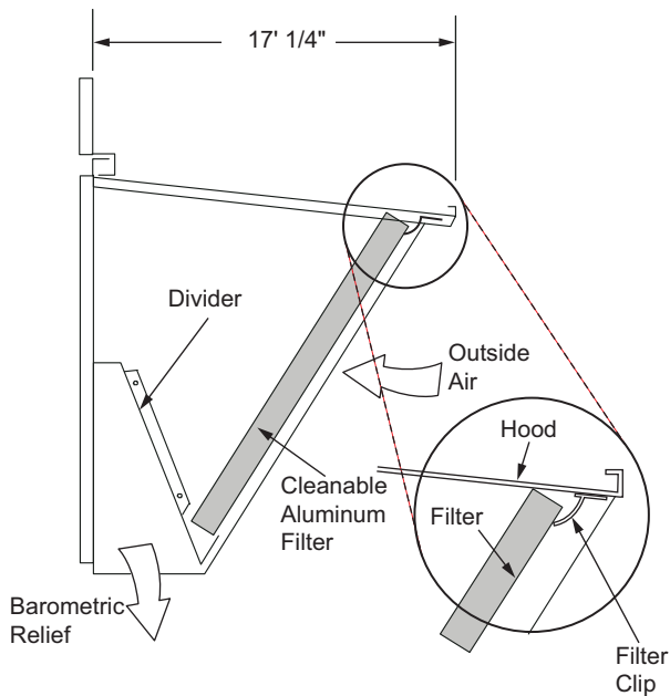
Fig. 5 — Filter Installation
