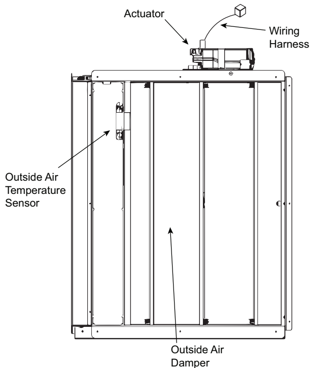
Fig. 53 — 50GC-*07-12 EconomizerONE Component Locations (CRECOMZR108A00 Shown)
