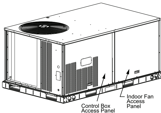
Fig. 3 — Blower Access Panel Location (size 12 units)
