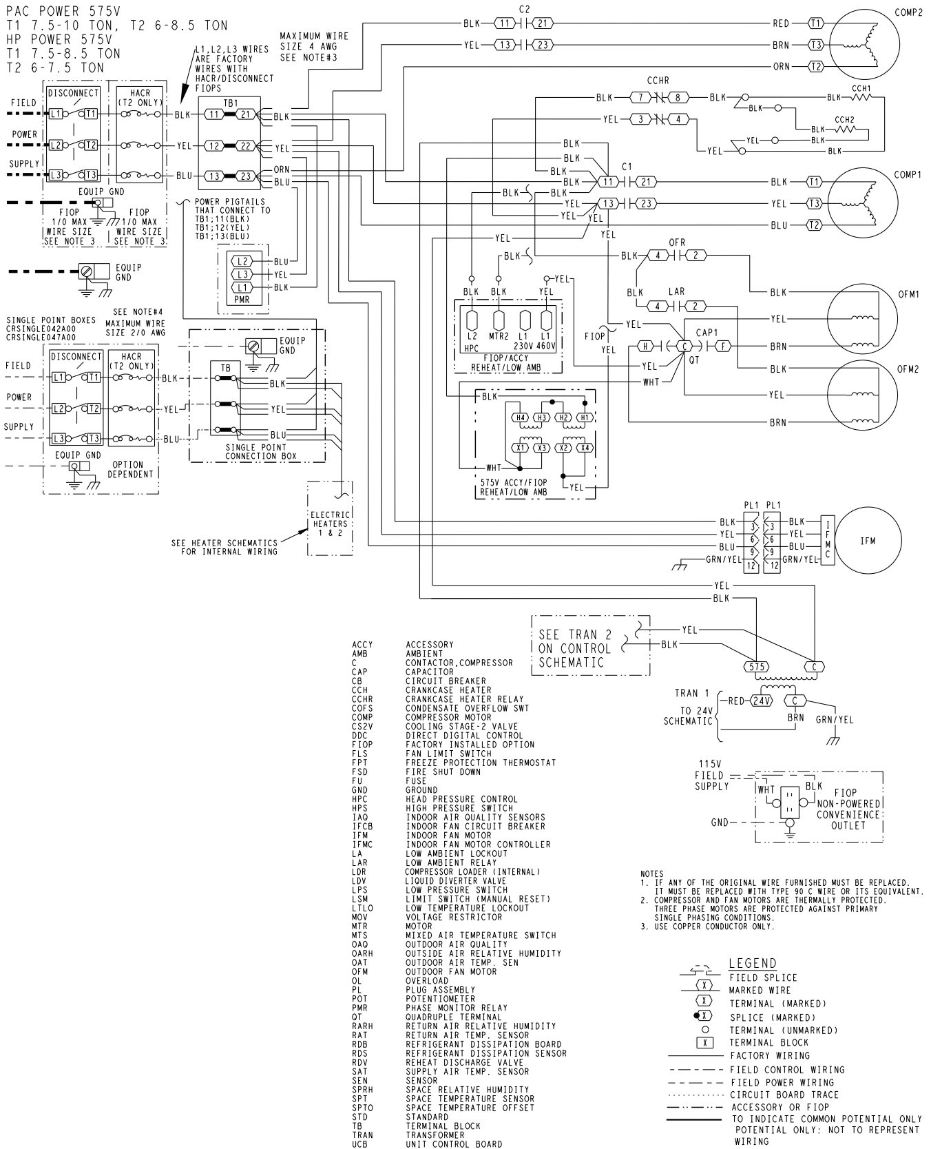
Fig. I — 50GC-07-09 Power Wiring Diagram — 575-3-60 Unit Electromechanical with POL224 Controller — Standard/Medium SCCR
