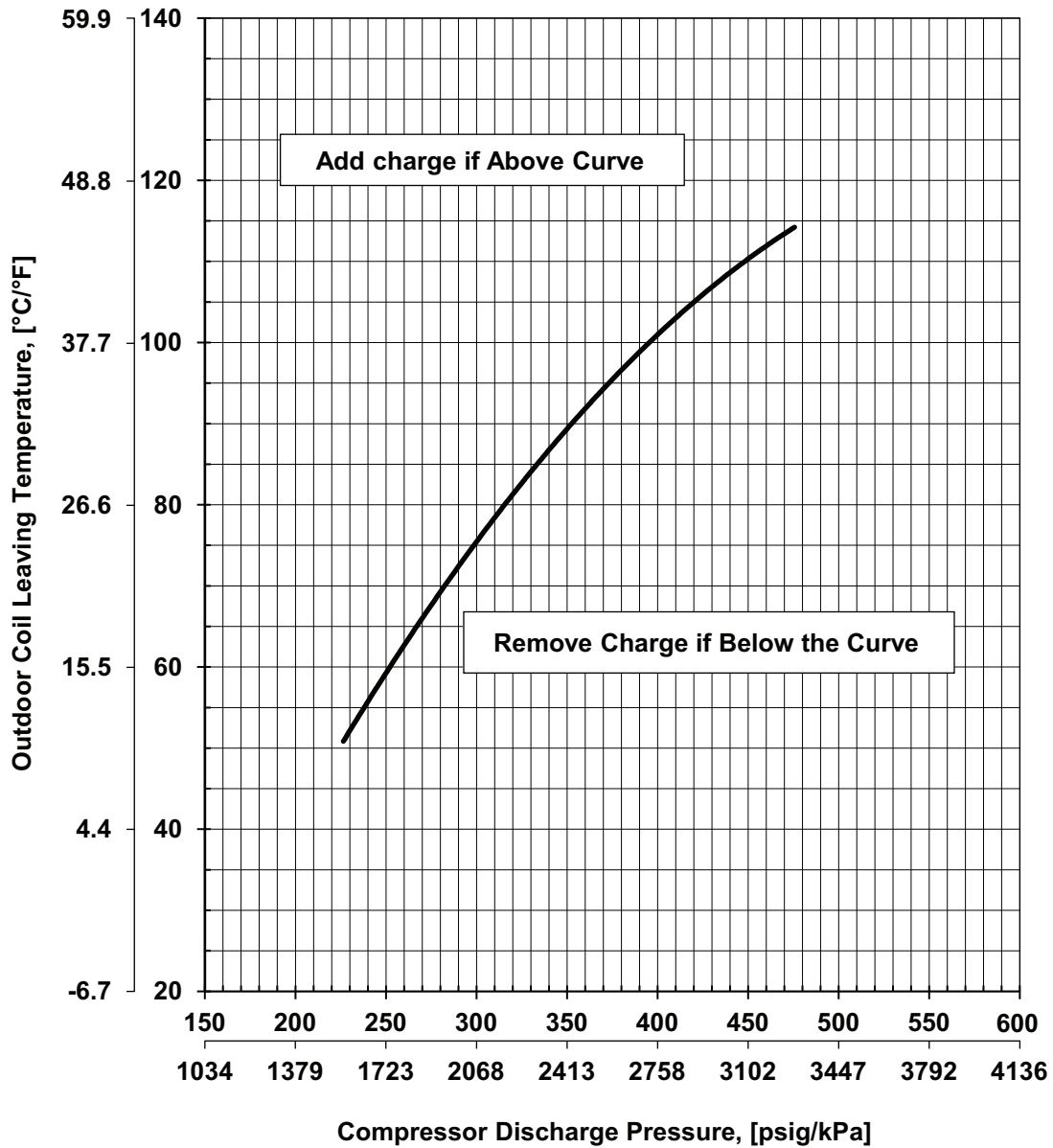
Fig. 28 — Cooling Charging Chart - 10 Ton
