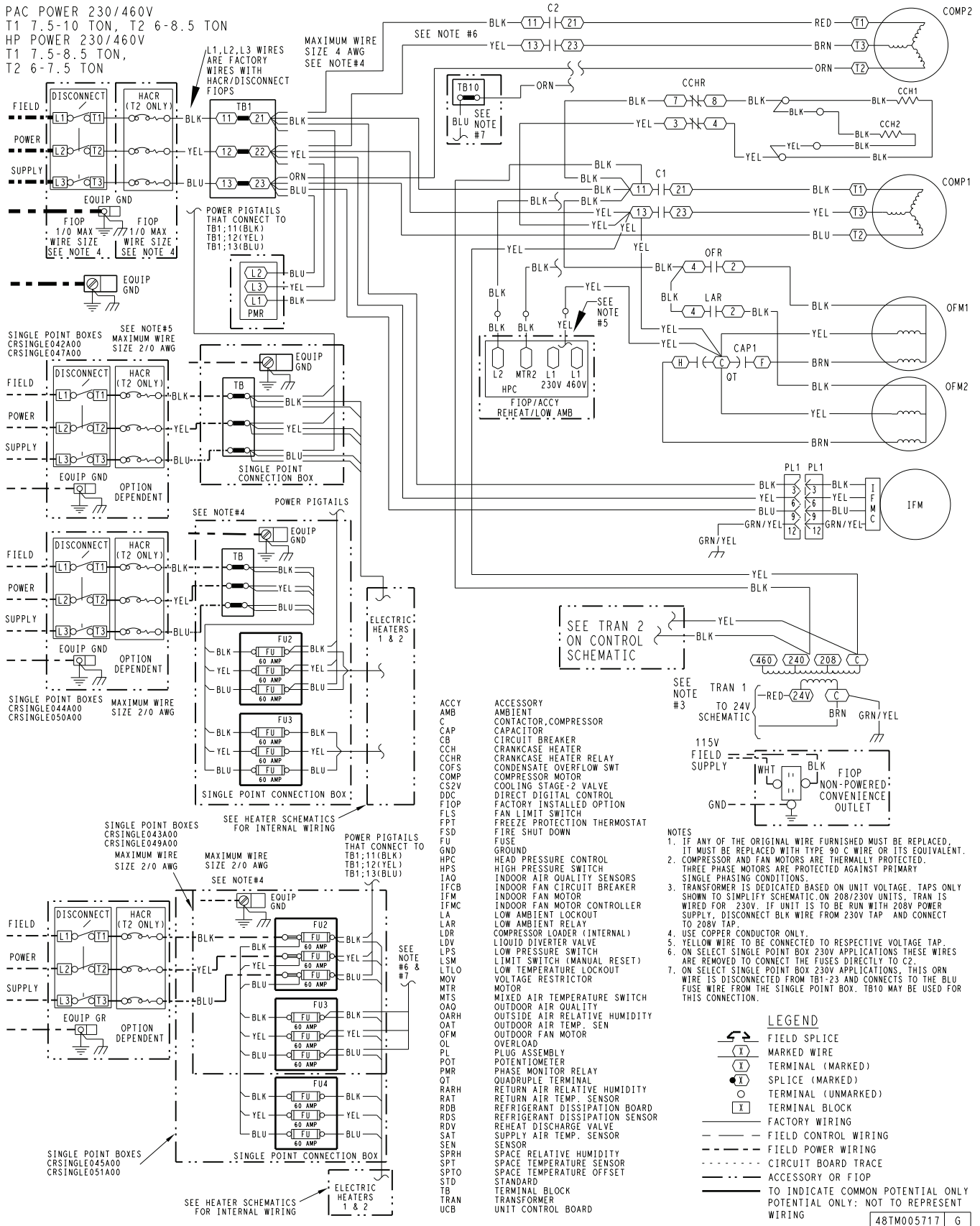
Fig. H — 50GC-*07-09 Power Wiring Diagram — 208/230, 460-3-60 Unit Electromechanical with POL224 Controller — Standard/Medium SCCR
