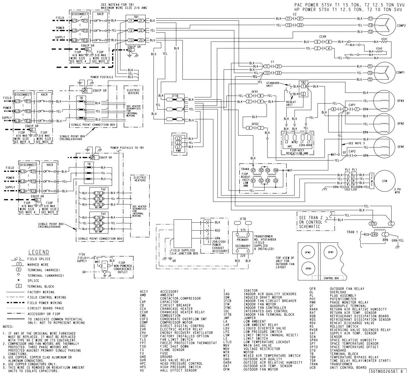
Fig. Q — 50GC-14 Power Wiring Diagram — 575-3-60 Unit with SystemVu™ Control — Standard/Medium SCCR
