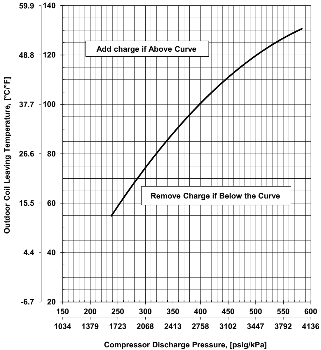
Fig. 27 — Cooling Charging Chart - 8.5 Ton
