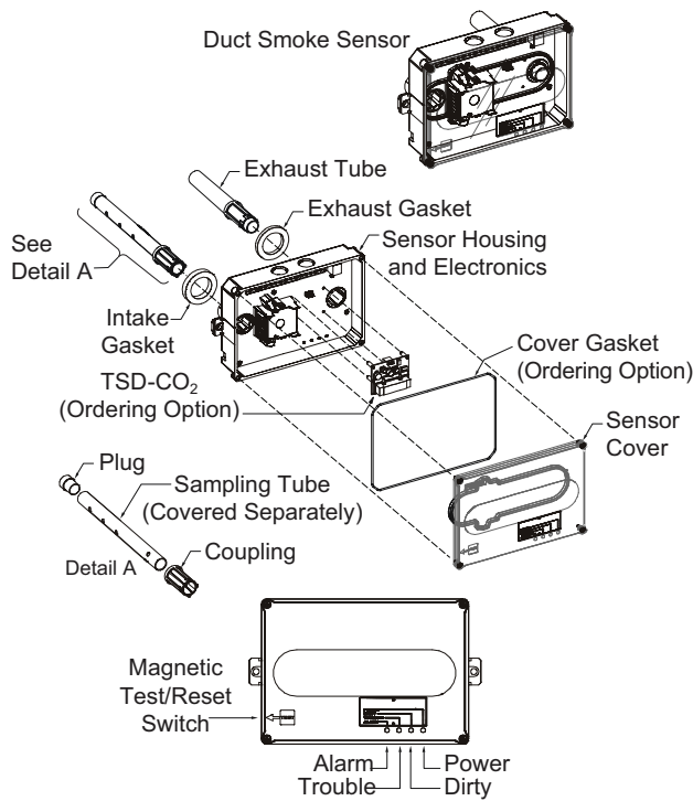
Fig. 43 — Smoke Detector Sensor
