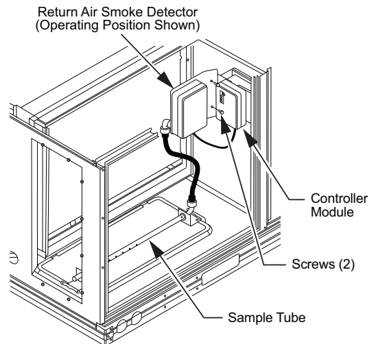
Fig. 45 — Return Air Smoke Detector Operating Position
