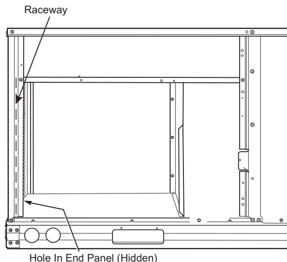
Fig. 39 — 50GC-*07-12 Low-Voltage Wiring Raceway
