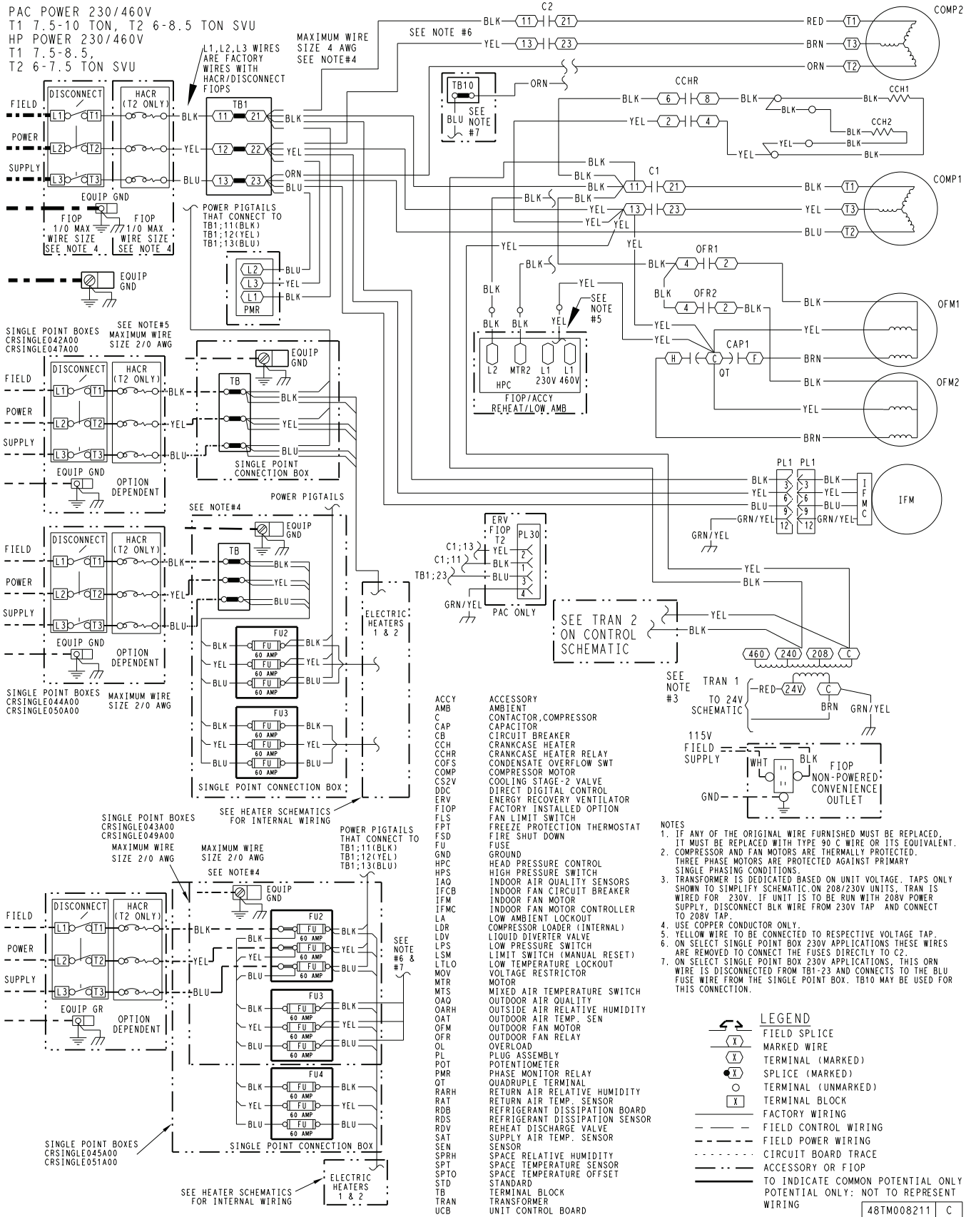
Fig. N — 50GC*07-09 Power Wiring Diagram — 208/230, 460-3-60 Unit with SystemVu™ Control — Standard/Medium SCCR
