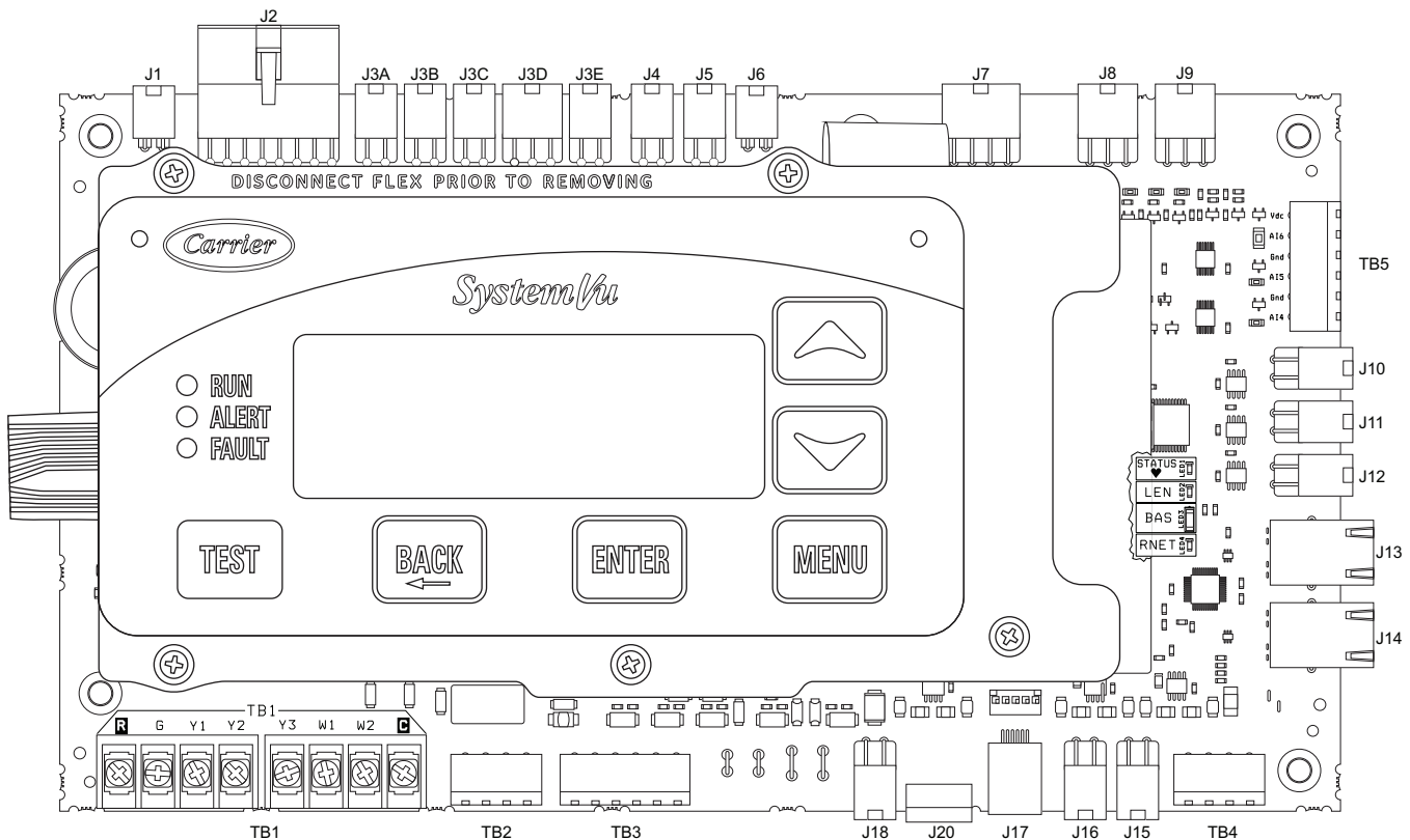
Fig. 52 — SystemVu Control
