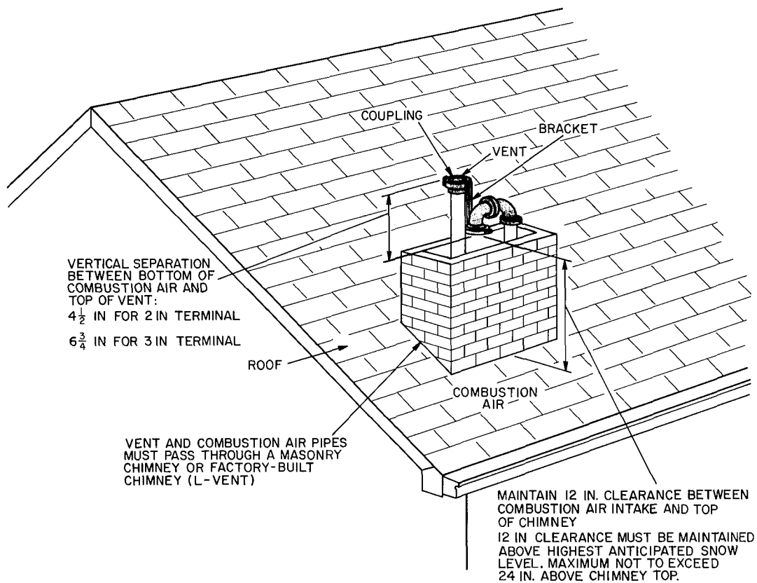
Fig. 1 — Rooftop Vent Termination
