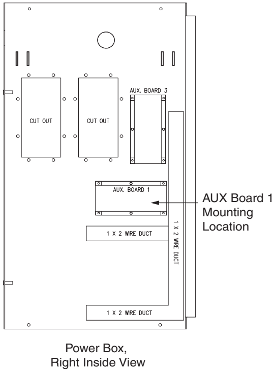
Fig. 7 — AUX Board Location
