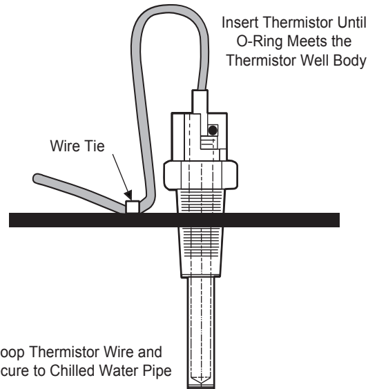
Fig. 3 — Accessory Leaving Water Thermistor
