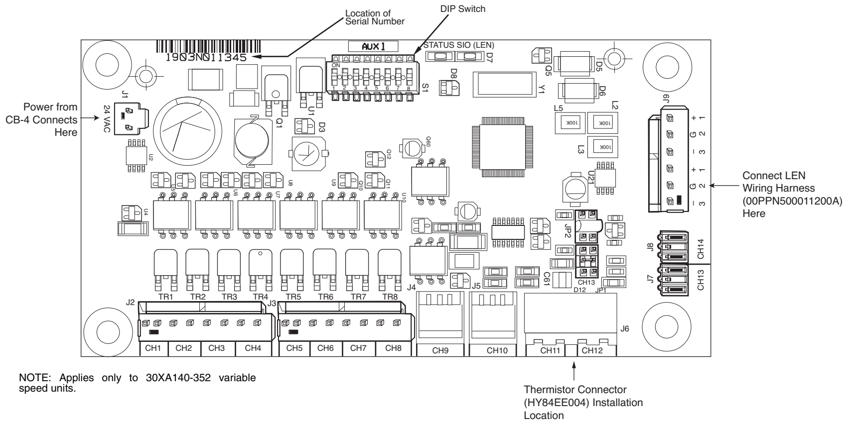
Fig. 6 — AUX Board
