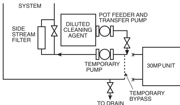
Fig. 60 — Cleaning Using a Side Stream Filter
