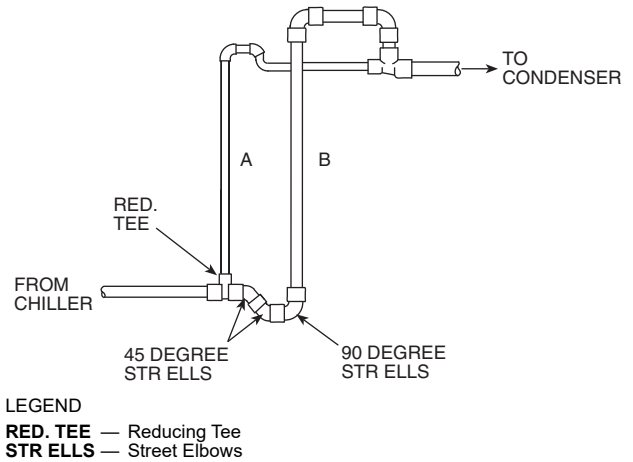
Fig. 33 — Double Discharge Riser Construction Detail
