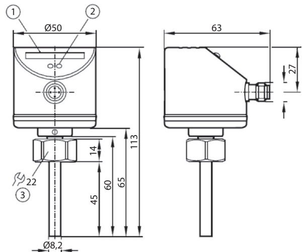
Fig. 55 — Chilled Water Flow Switch
