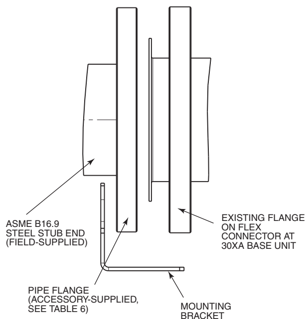
Fig. 11 — Connect Steel Suction Line at the 30XA Base Unit (Shown) and Cooler (30XA140, 160: Circuit A and 30XA180-350: All Circuits)
