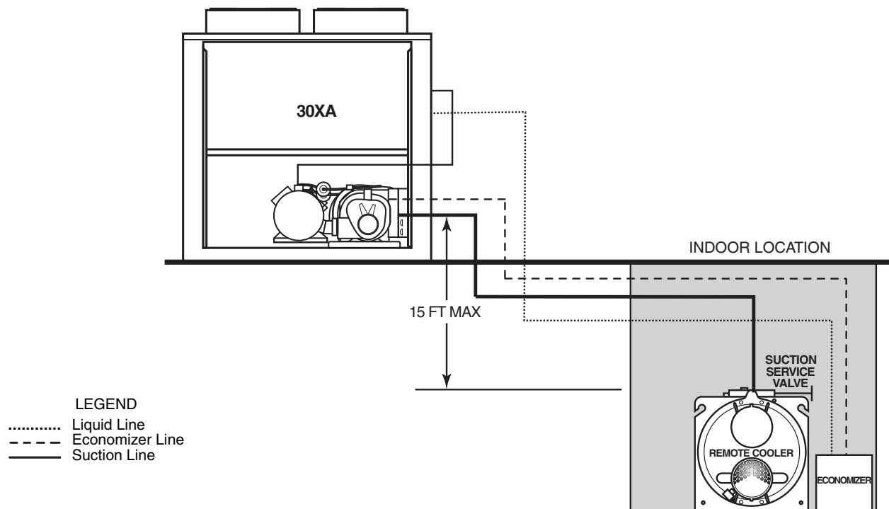
Fig. 3 — 30XA Unit with Cooler Located Below Unit (Single Circuit Shown)
