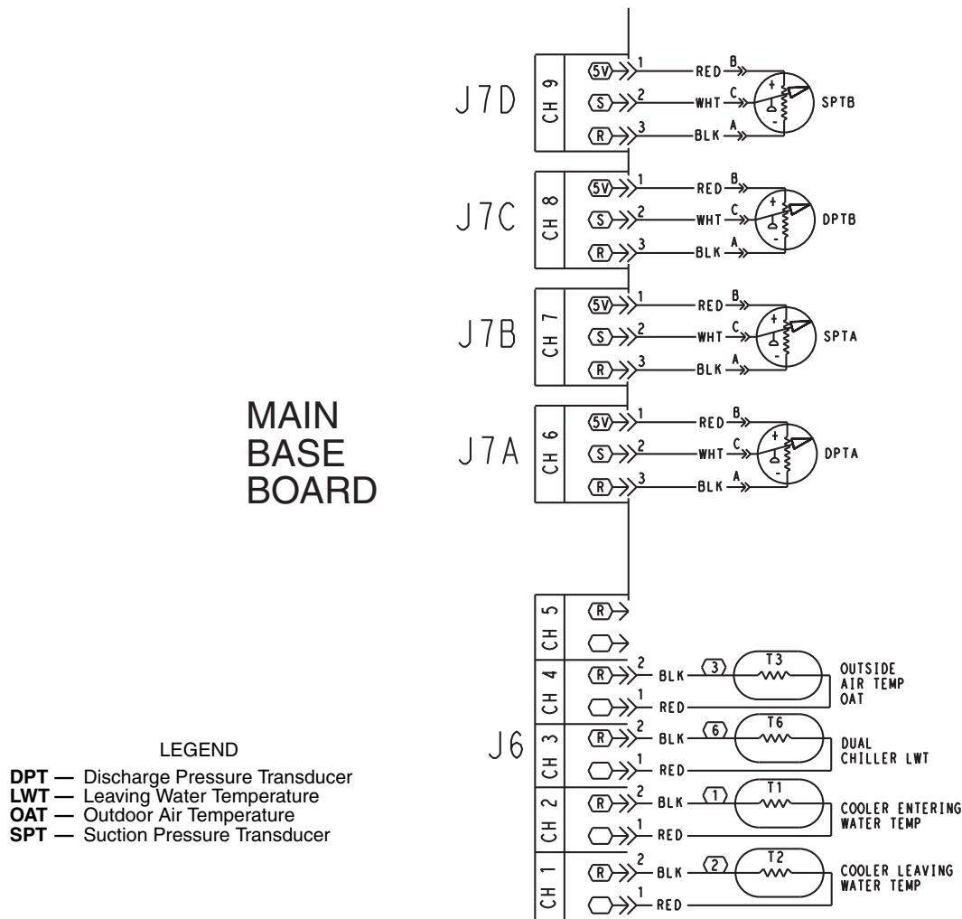
Fig. 13 — Thermistor Connections
