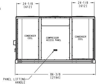
RIGHT DEDICATED VERTICAL AIRFLOW UNIT 17 SIZE
