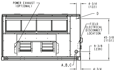
LEFT SHOWN WITH THE POWER EXHAUST OPTION INSTALLED
