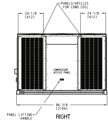
DEDICATED VERTICAL AIRFLOW UNIT 28 SIZE
