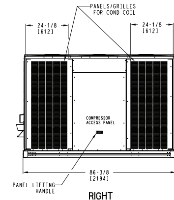
DEDICATED HORIZONTAL AIRFLOW UNIT 28 SIZE
