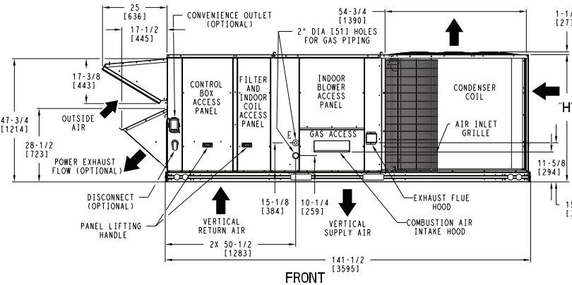
DEDICATED VERTICAL AIRFLOW UNIT 20,24 SIZE
