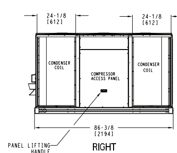
DEDICATED HORIZONTAL AIRFLOW UNIT 20,24 SIZE
