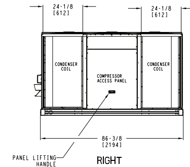
DEDICATED VERTICAL AIRFLOW UNIT 17 SIZE
