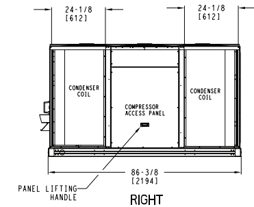
DEDICATED HORIZONTAL AIRFLOW UNIT 17 SIZE
