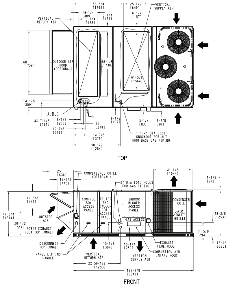
DEDICATED VERTICAL AIRFLOW UNIT 17 SIZE
