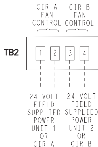
Fig. 29 — 09RC050-230 with Dual Control Circuit Wiring
