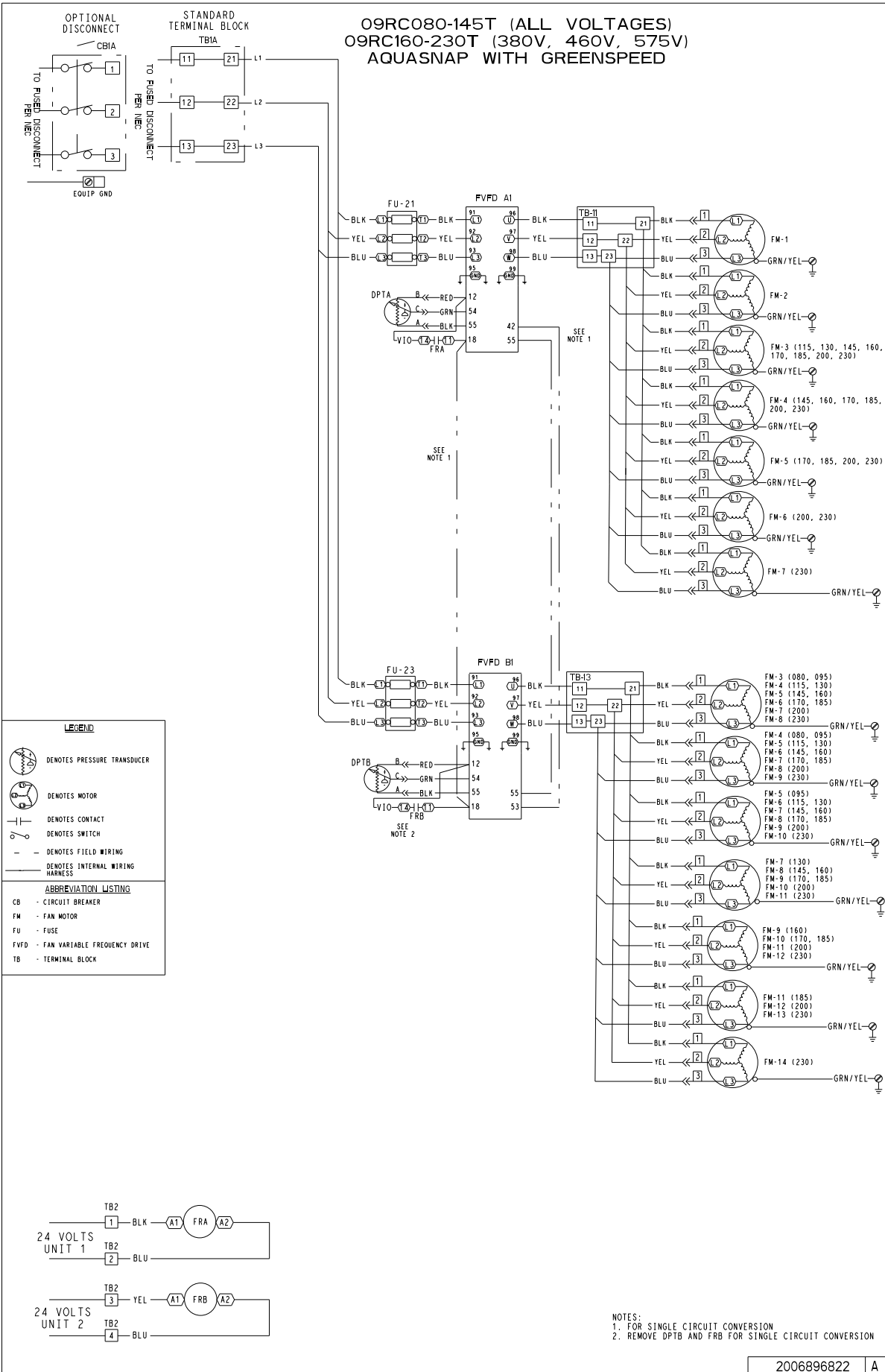
Fig. 38 — 09RC080-145 (All Voltages), 09RC160-230 (380-v, 460-v, 575-v) Aquasnap with Greenspeed Controller
