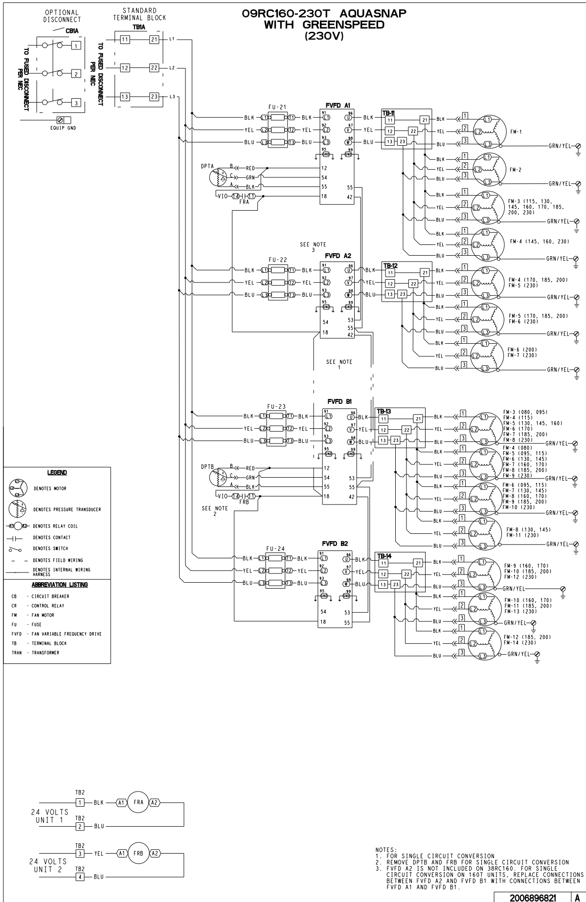
Fig. 37 — 09RC160-230 (230-v) Aquasnap with Greenspeed Controller
