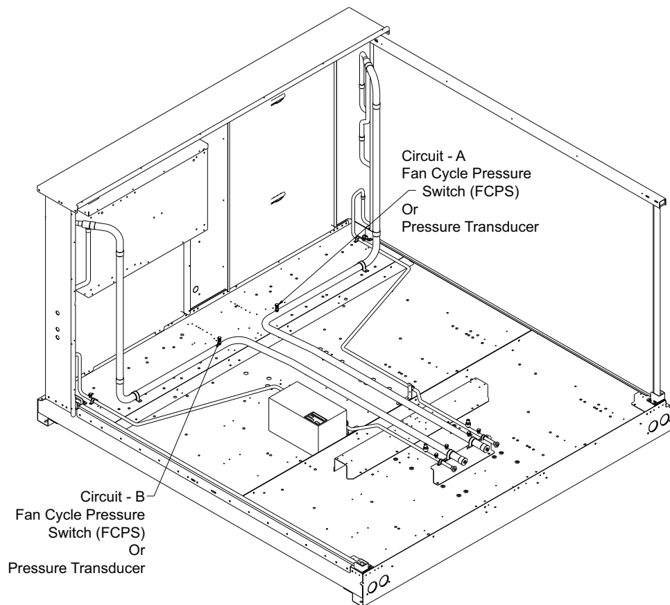
Fig. 22 — Unit Piping — Sizes 035-060
