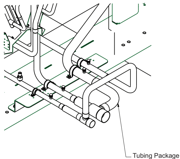
Fig. 25 — Tubing Package Installed in Unit
