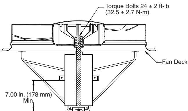
Fig. 34 — AeroAcoustic Fan Mounted Position
