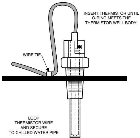
Fig. 18 — Dual Chiller Leaving Water Thermistor (Part No. 30RB660036)
