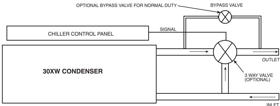
Fig. 13 — Condenser Fluid Control Valve Installation
