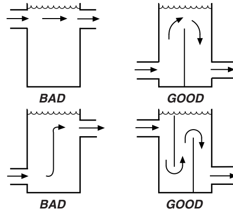
Fig. 1 — Tank Baffling
