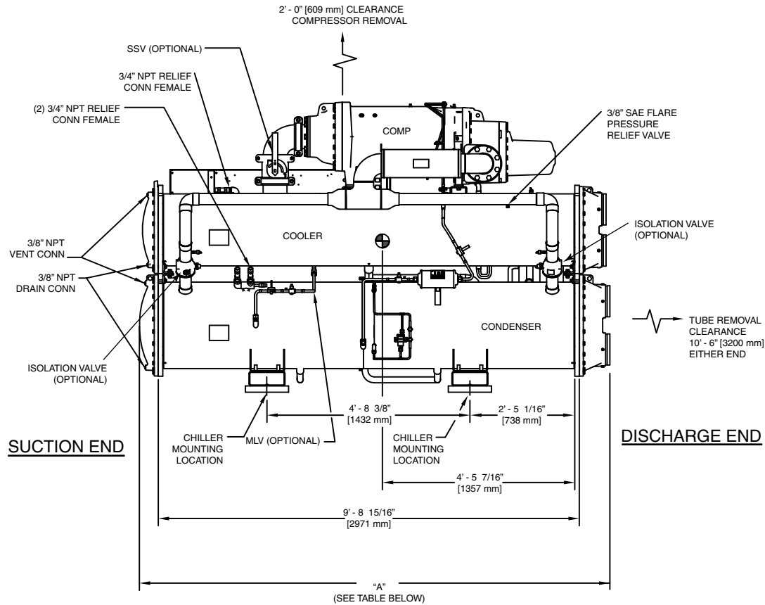
CHILLER DIMENSIONS
