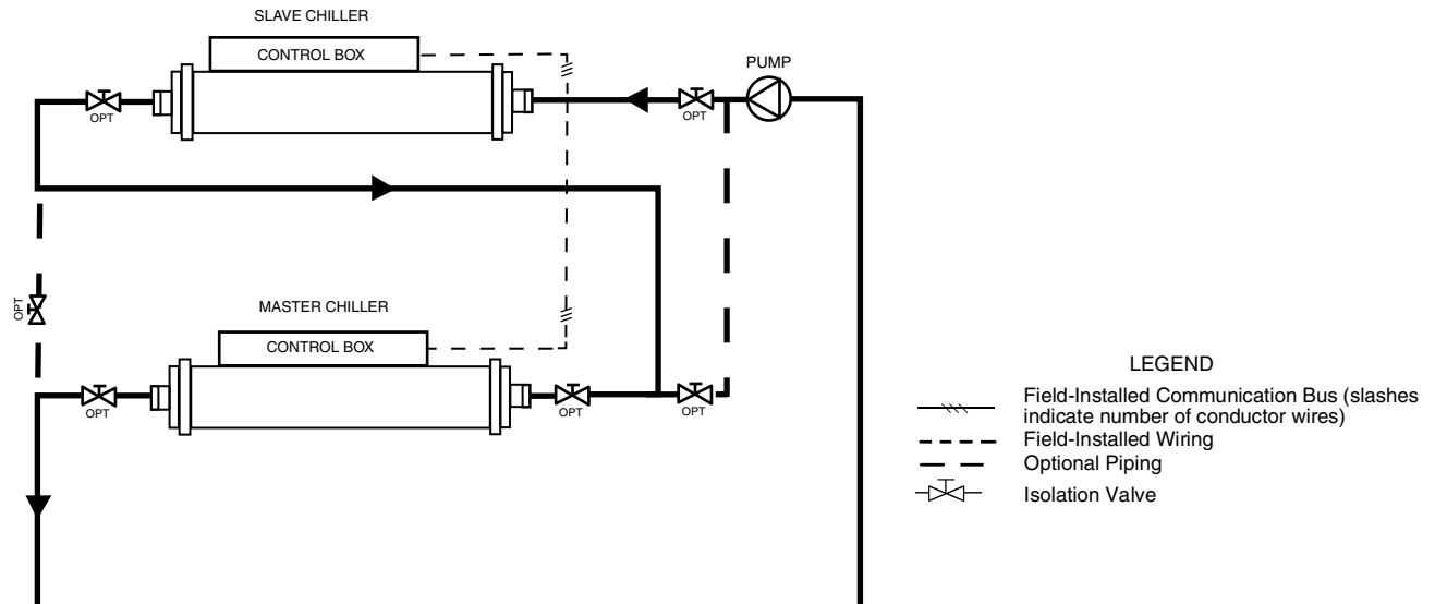
Fig. 16 — Series Dual Chiller Operation
