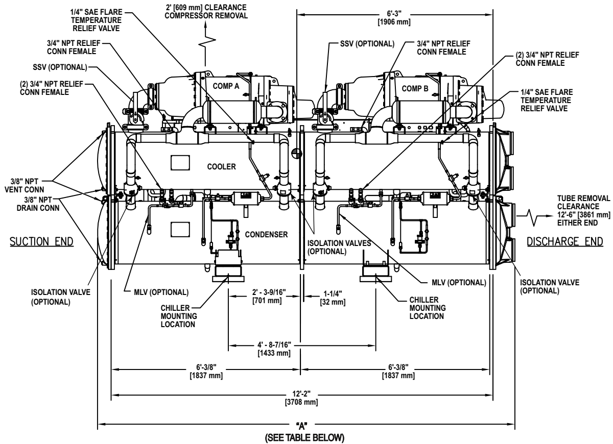
CHILLER DIMENSIONS
