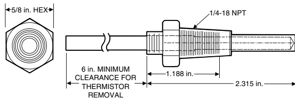
Fig. 17 — Dual Chiller Leaving Water Thermistor Well (Part No. 00PPG000008000A)
