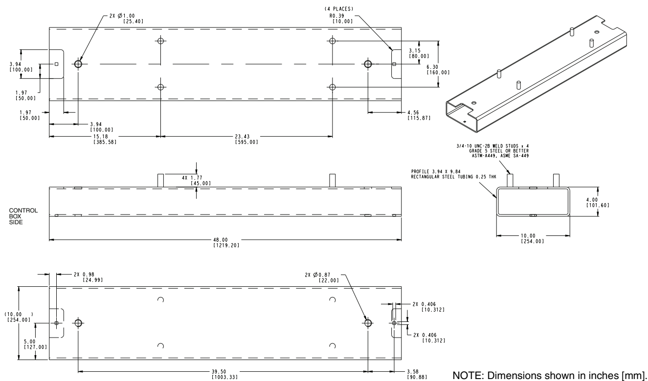
Fig. 6 — 30XW150-200 Unit Mounting Feet Dimensions
