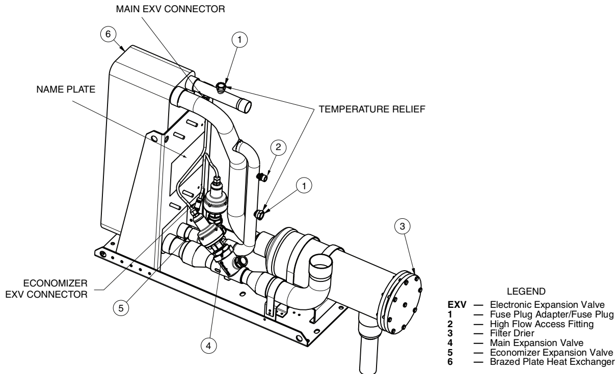
Fig. 14 — Typical Economizer Assembly
