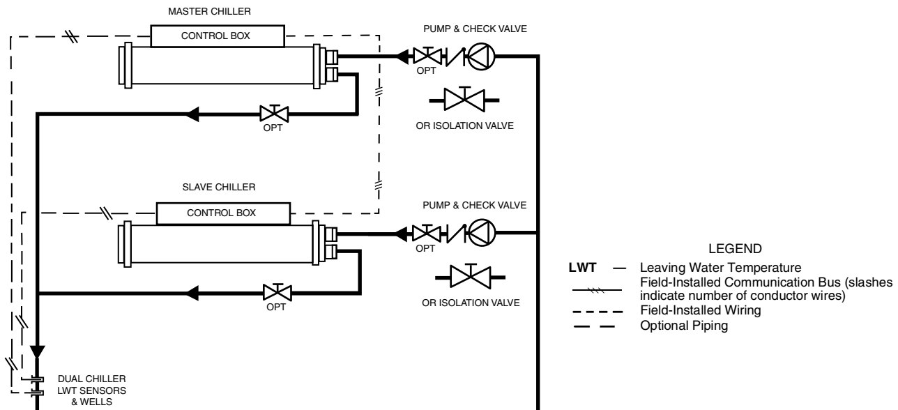
Fig. 15 — Parallel Dual Chiller Operation
