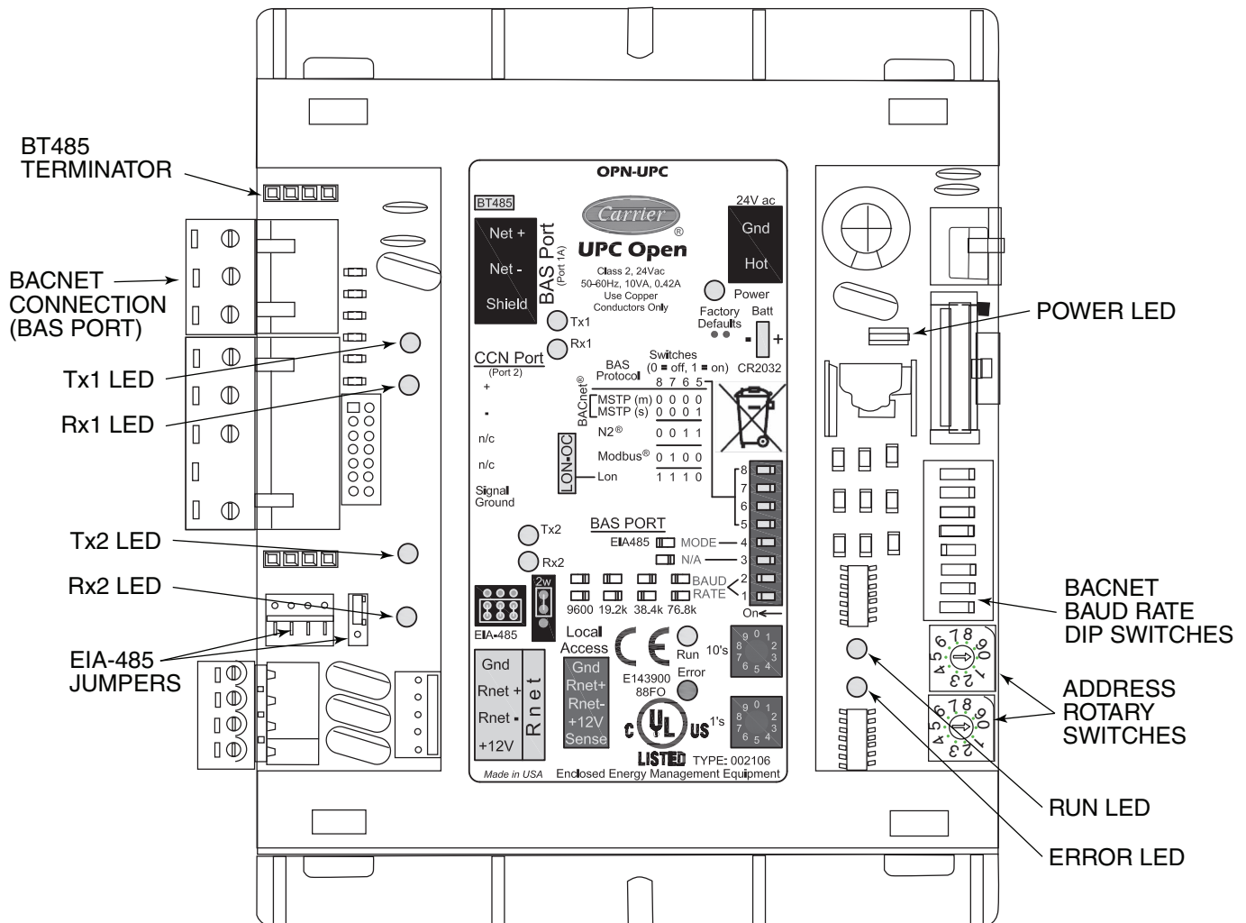
Fig. 22 — UPC Open Controller
