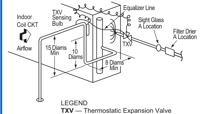
Location of Sight Glass(es) and Filter Driers (typical 38AXQ / 40RLQ size 07 and 08 system)
