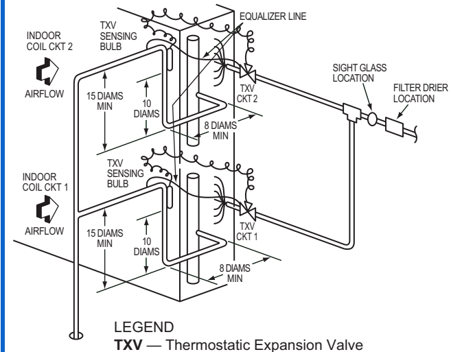
Location of Sight Glass(es) and Filter Driers (typical 38AXQ / 40RLQ size 12 system)
