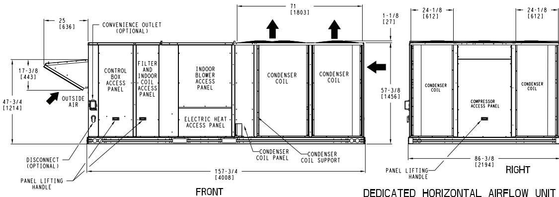
DEDICATED HORIZONTAL AIRFLOW UNIT 30 SIZE
