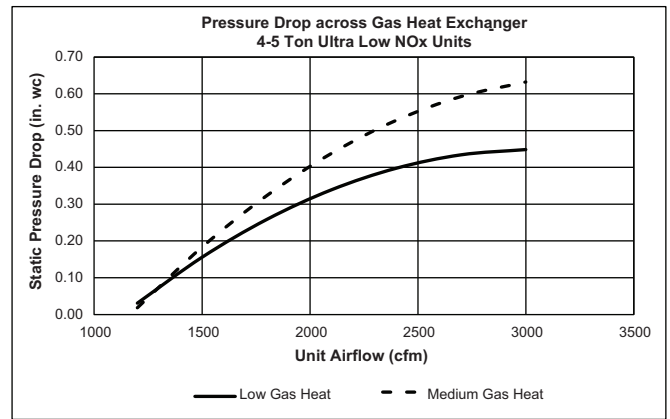
Pressure Drop across Gas Heat Exchanger, 48FE Ultra Low NOx — 4 to 5 Ton Units
