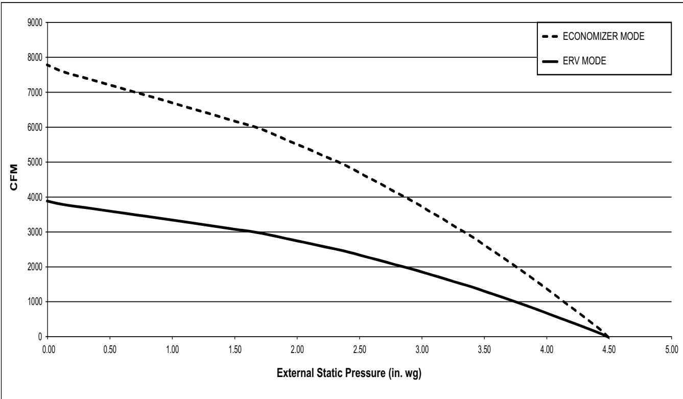
48HC**20 SUPPLY AND EXHAUST FAN PERFORMANCE CURVES
