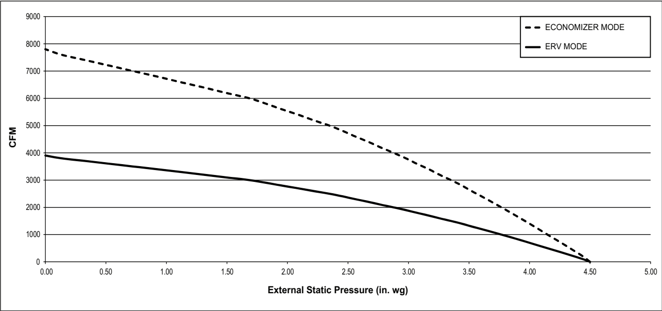
48HC**17 SUPPLY AND EXHAUST FAN PERFORMANCE CURVES
