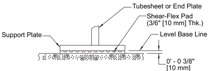
VIEW B-B
