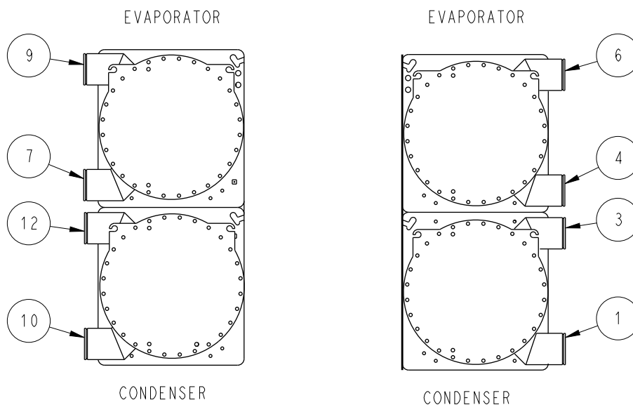
NOZZLE ARRANGEMENT CODES FOR MARINE WATERBOXES
