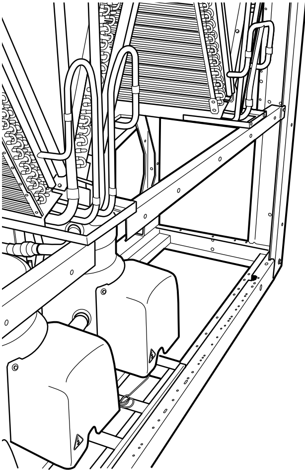
Fig. 26 — Compressor Side with Metal Supports Installed (30RB090 Shown)
