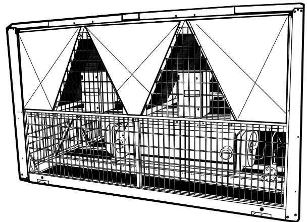
Fig. 29 — Water Connection Side with Metal Supports/Grilles Installed (30RB090 Shown)
