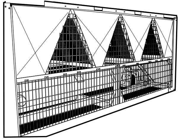
Fig. 33 — Water Connection Side, Installation Complete (30RB150 Shown)
