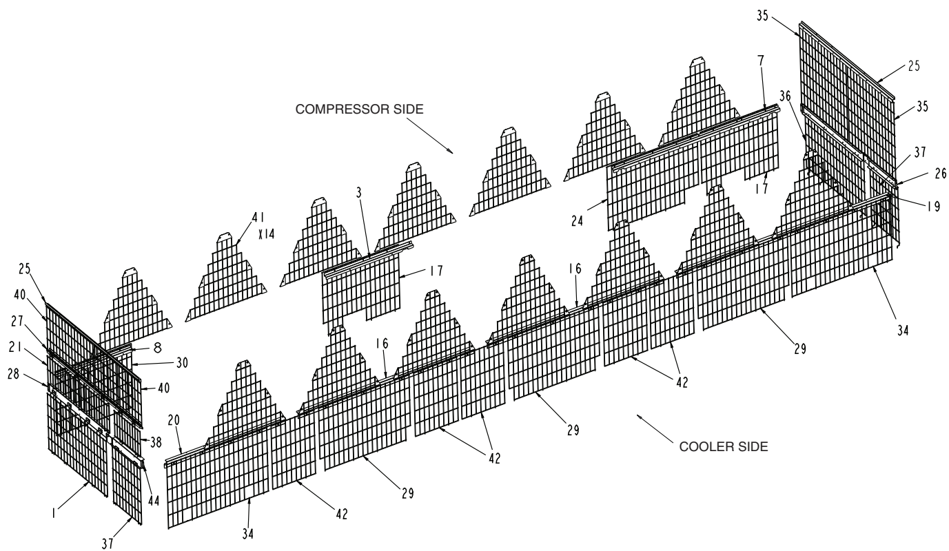
Fig. 17 — Metal Support and Grille Placement, 30XA260-302 Units with High SCCR Option
