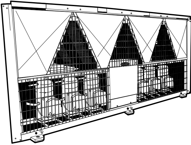
Fig. 31 — Compressor Side, Installation Complete (30RB150 Shown)
