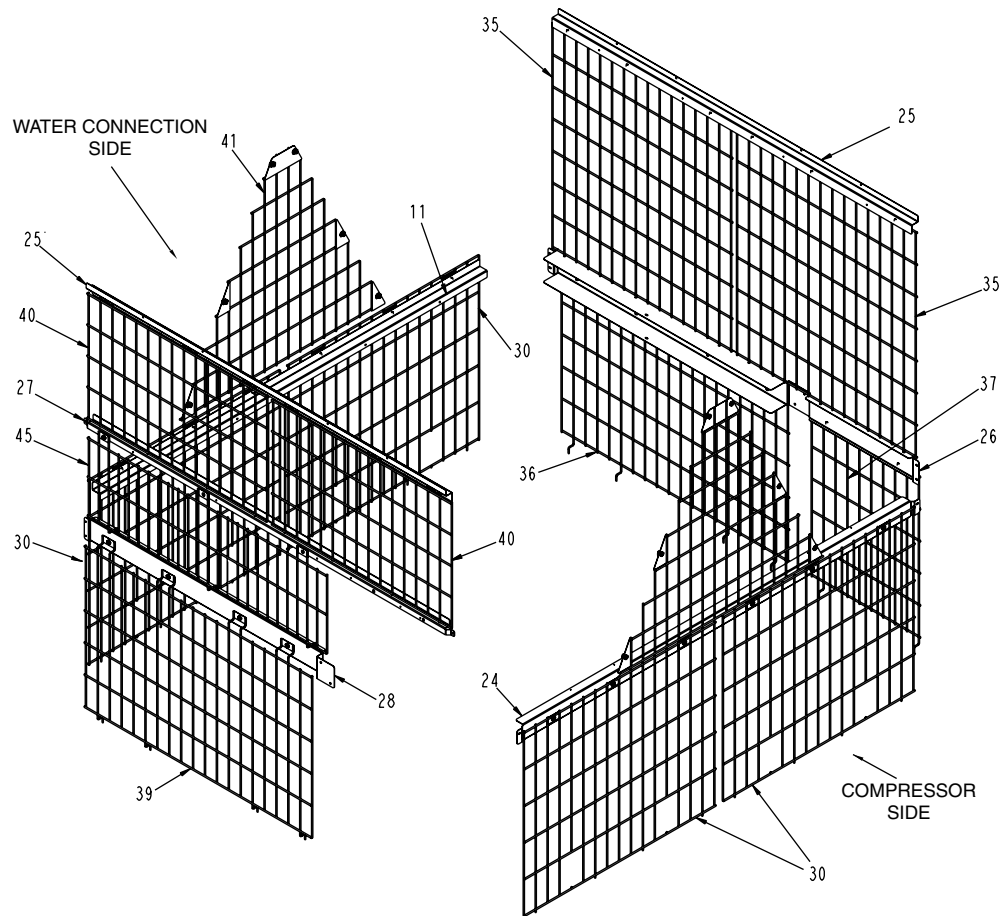
Fig. 2 — Metal Support and Grille Placement, 30RB060-080
