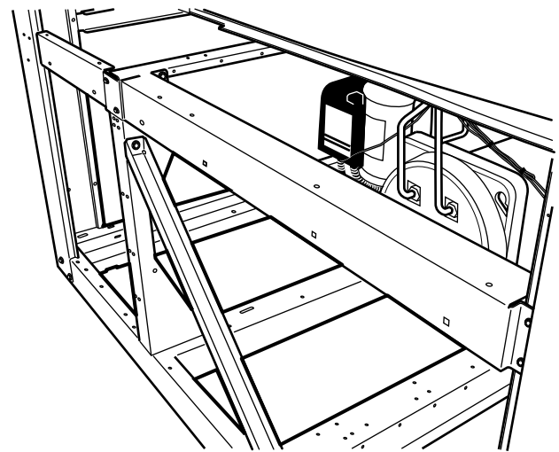
Fig. 28 — Blank End with Metal Supports Installed (30RB090 Shown)
