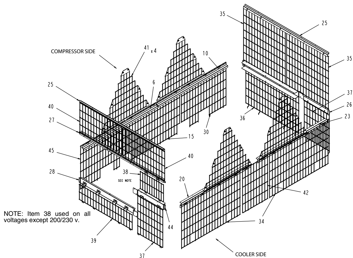
Fig. 11 — Metal Support and Grille Placement, 30XA080,082
