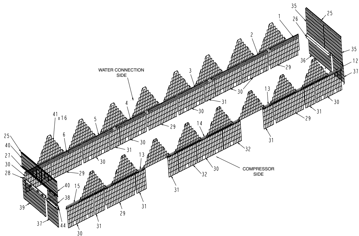
Fig. 10 — Metal Support and Grille Placement, 30RB300
