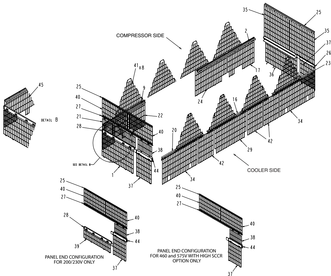
Fig. 13 — Metal Support and Grille Placement, 30XA140-162
