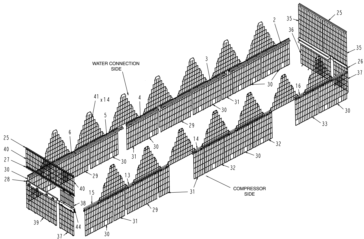
Fig. 9 — Metal Support and Grille Placement, 30RB275
