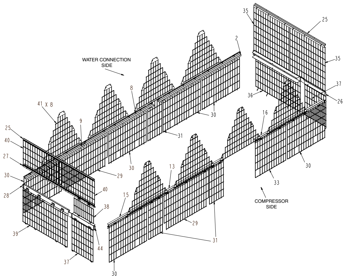
Fig. 5 — Metal Support and Grille Placement, 30RB160,170,315A/B,330A/B,345A/B,360B
