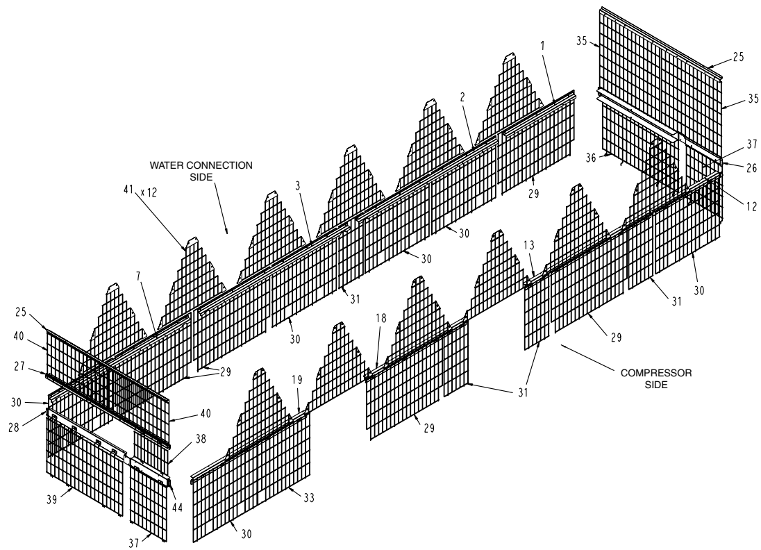
Fig. 8 — Metal Support and Grille Placement, 30RB250
