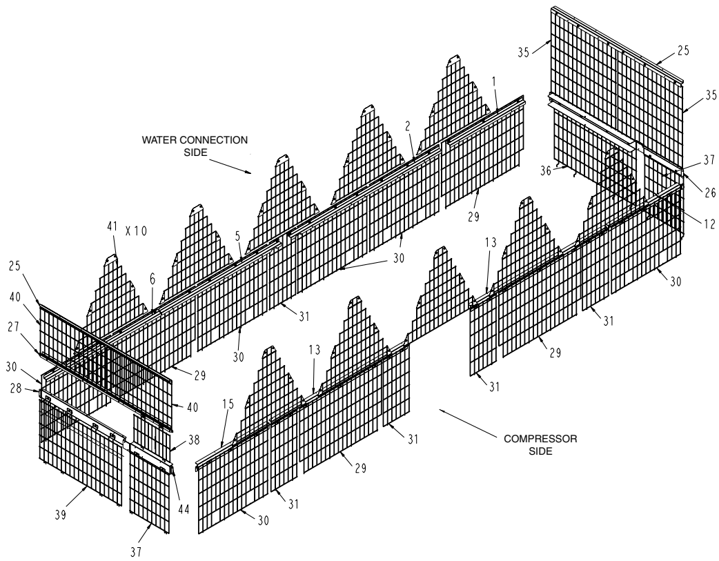
Fig. 6 — Metal Support and Grille Placement, 30RB190,360A,390A/B
