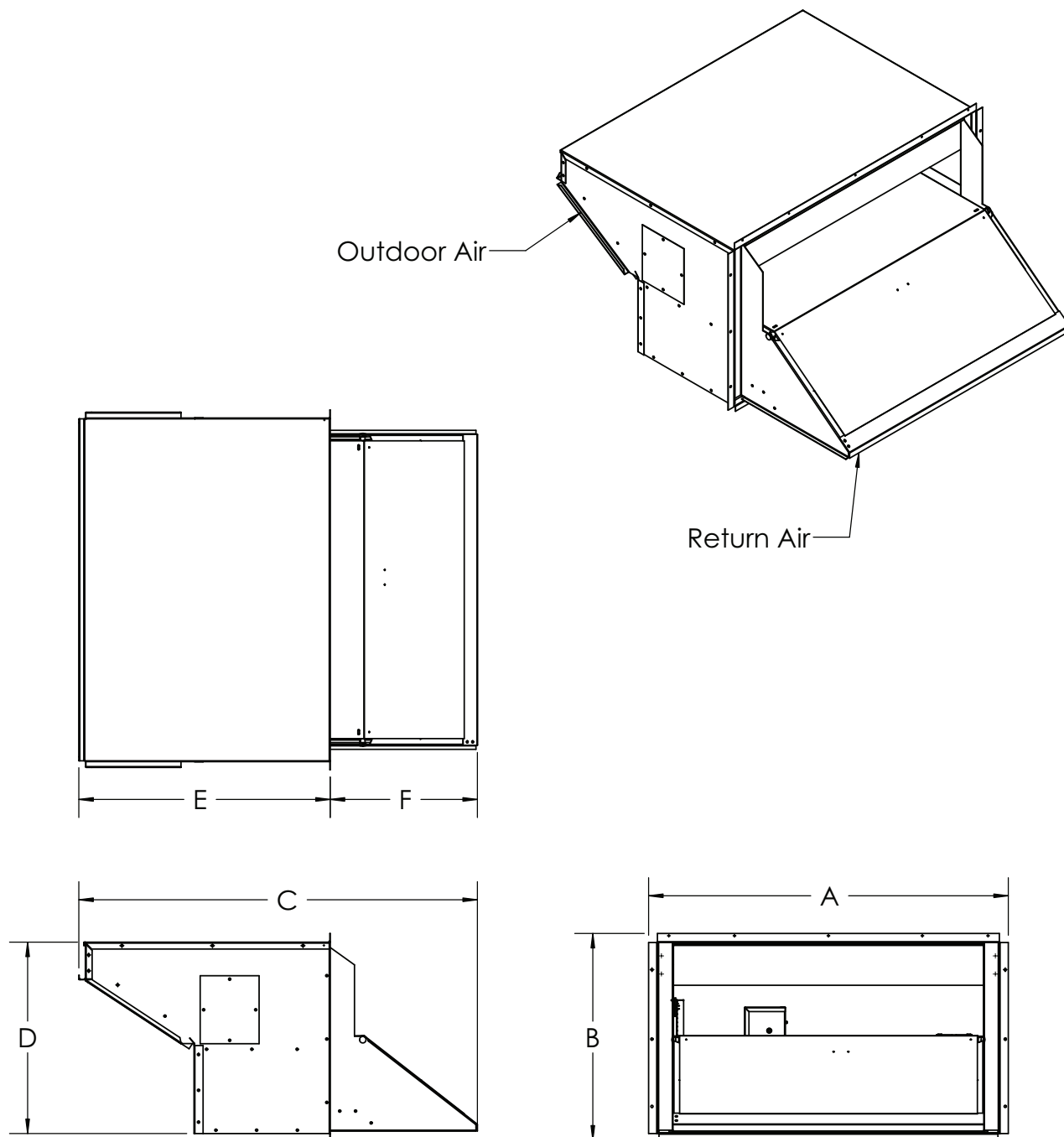
DIMENSIONS (in.)
