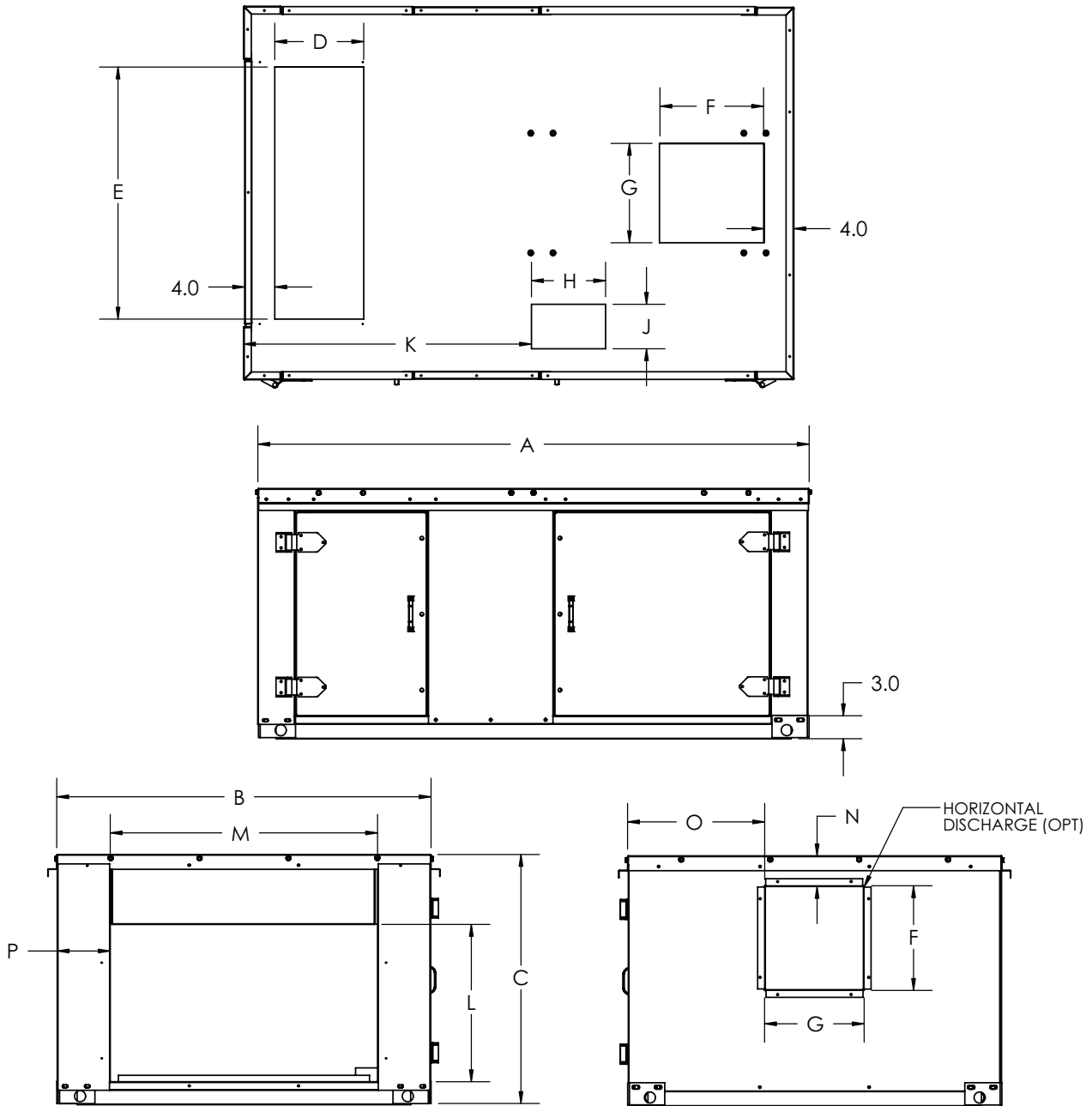
DIMENSIONS (in.)
