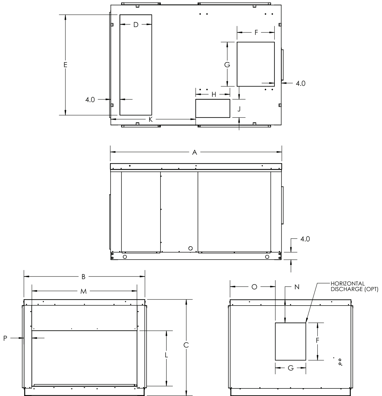
DIMENSIONS (in.)
