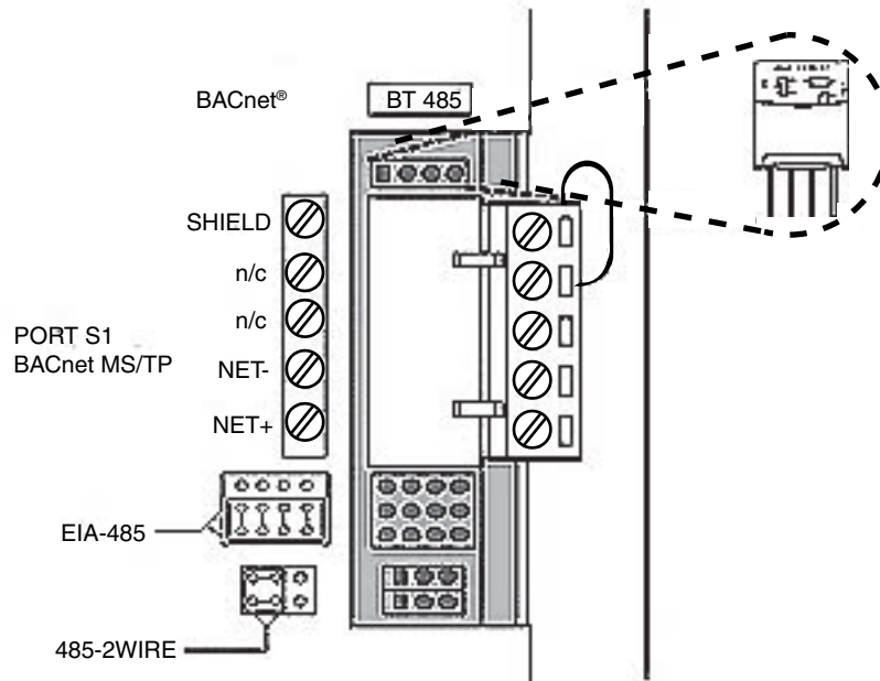
Fig. 63 — BT485 Installation
