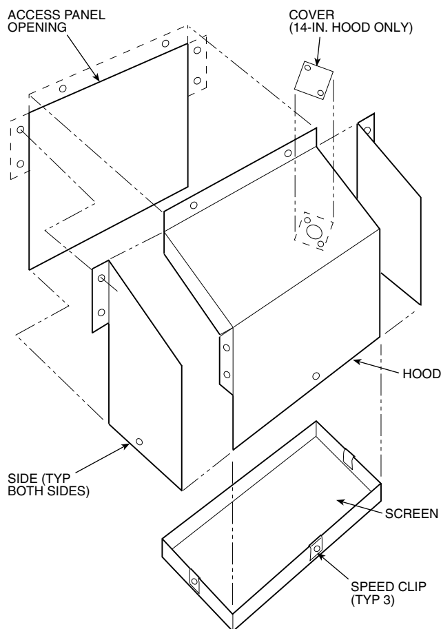
Fig. 31 — Inlet Hood Assembly (6 in. and 14 in.)
