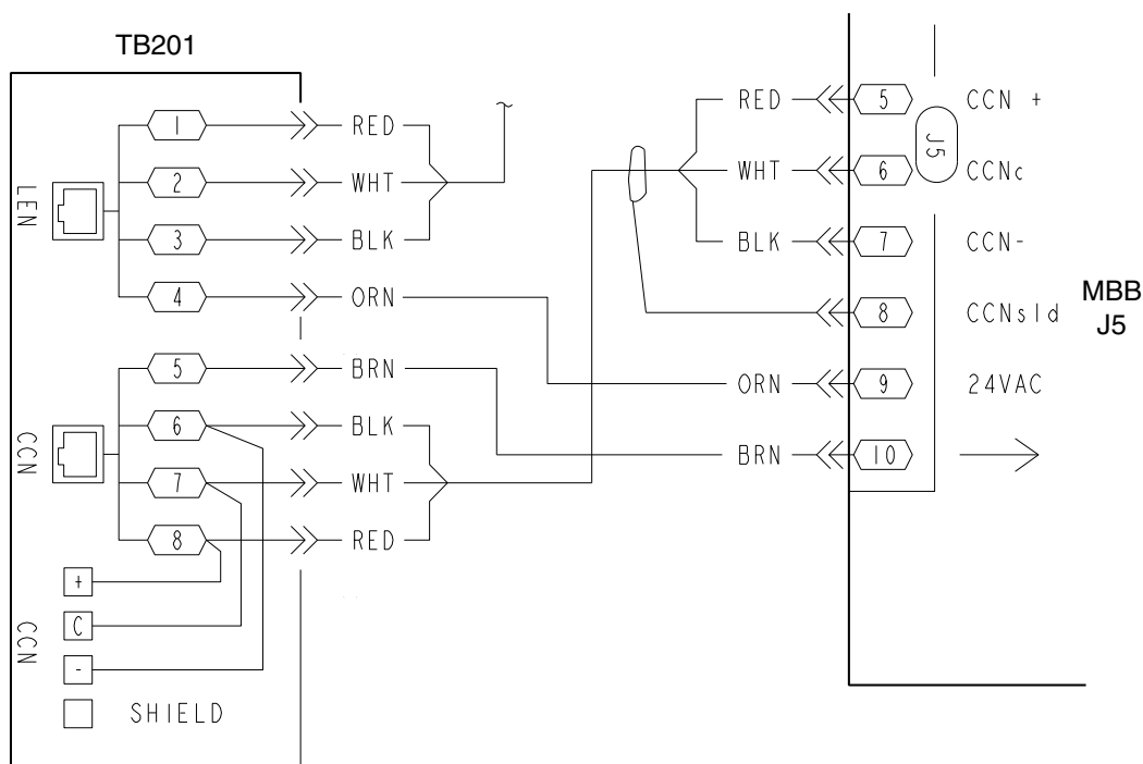
Fig. 60 — CCN Connections
