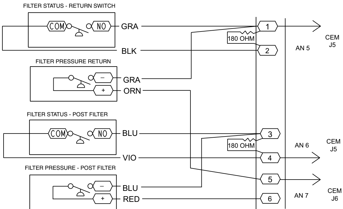
Fig. 53 — Filter Status Wiring
