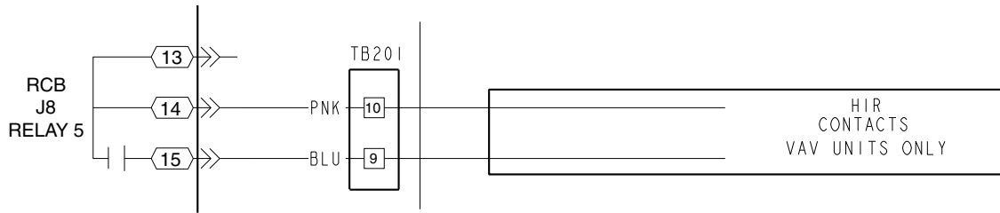
Fig. 50 — Heat Interlock Relay Wiring
