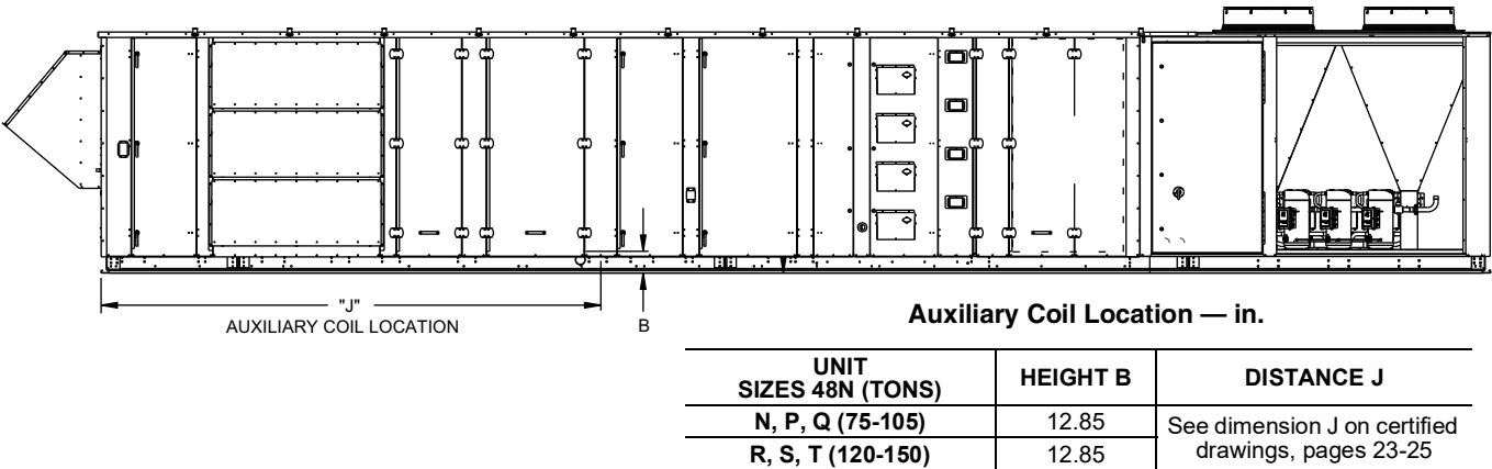
Fig. 13 — Units with Optional Extended Chassis — Location of Coil Tracks
