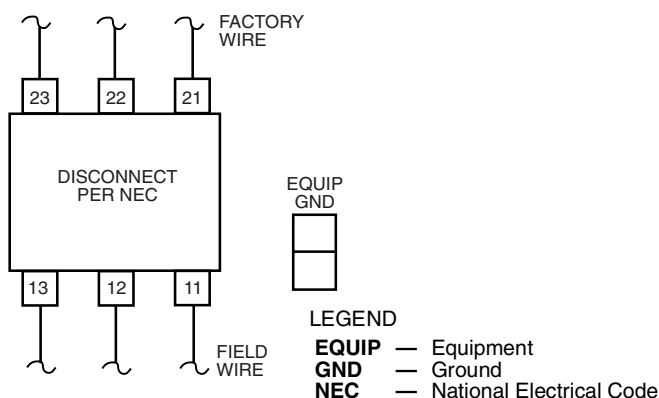
Fig. 23 — Field Power Wiring Connections for Factory-Installed Disconnect
