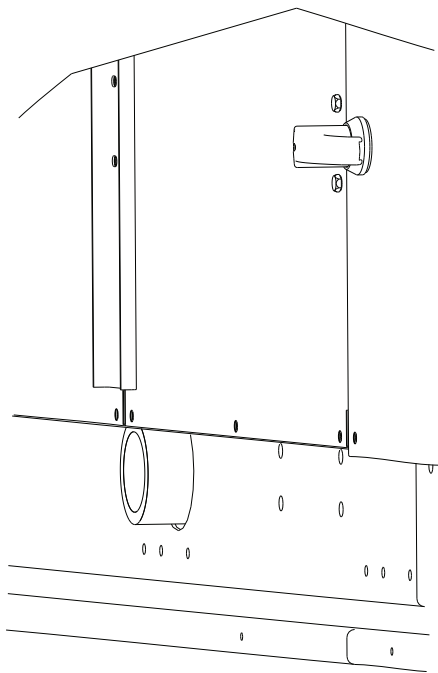
Fig. 14 — Primary Drain Connection
