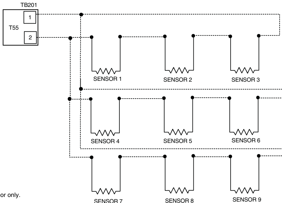
SPACE TEMPERATURE AVERAGING (9 SENSOR APPLICATION)
