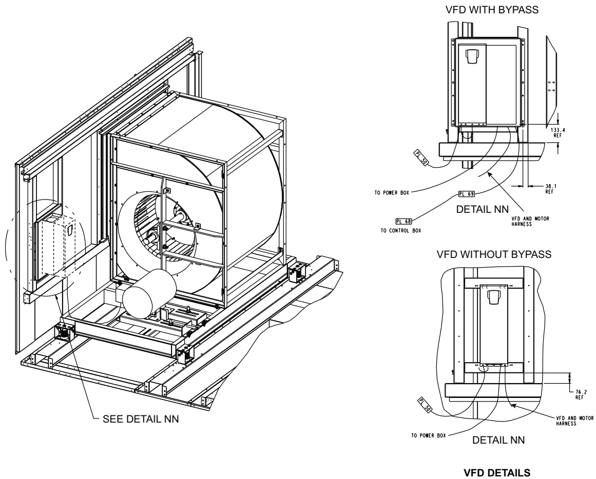
Fig. 45 — Return Section Component Locations
