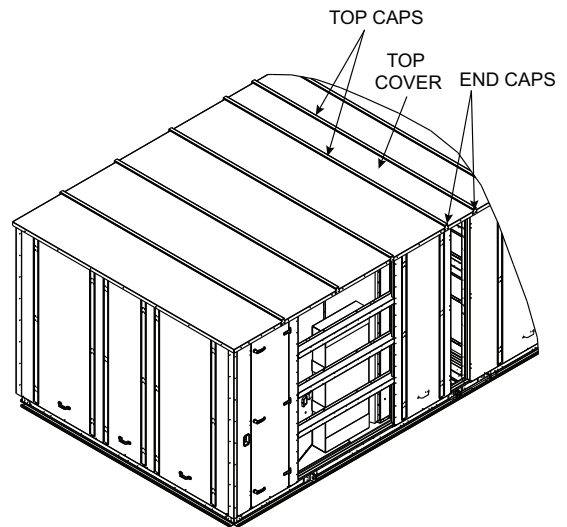
Fig. 43 — Main Unit and Return Section Top Cover Assemblies
