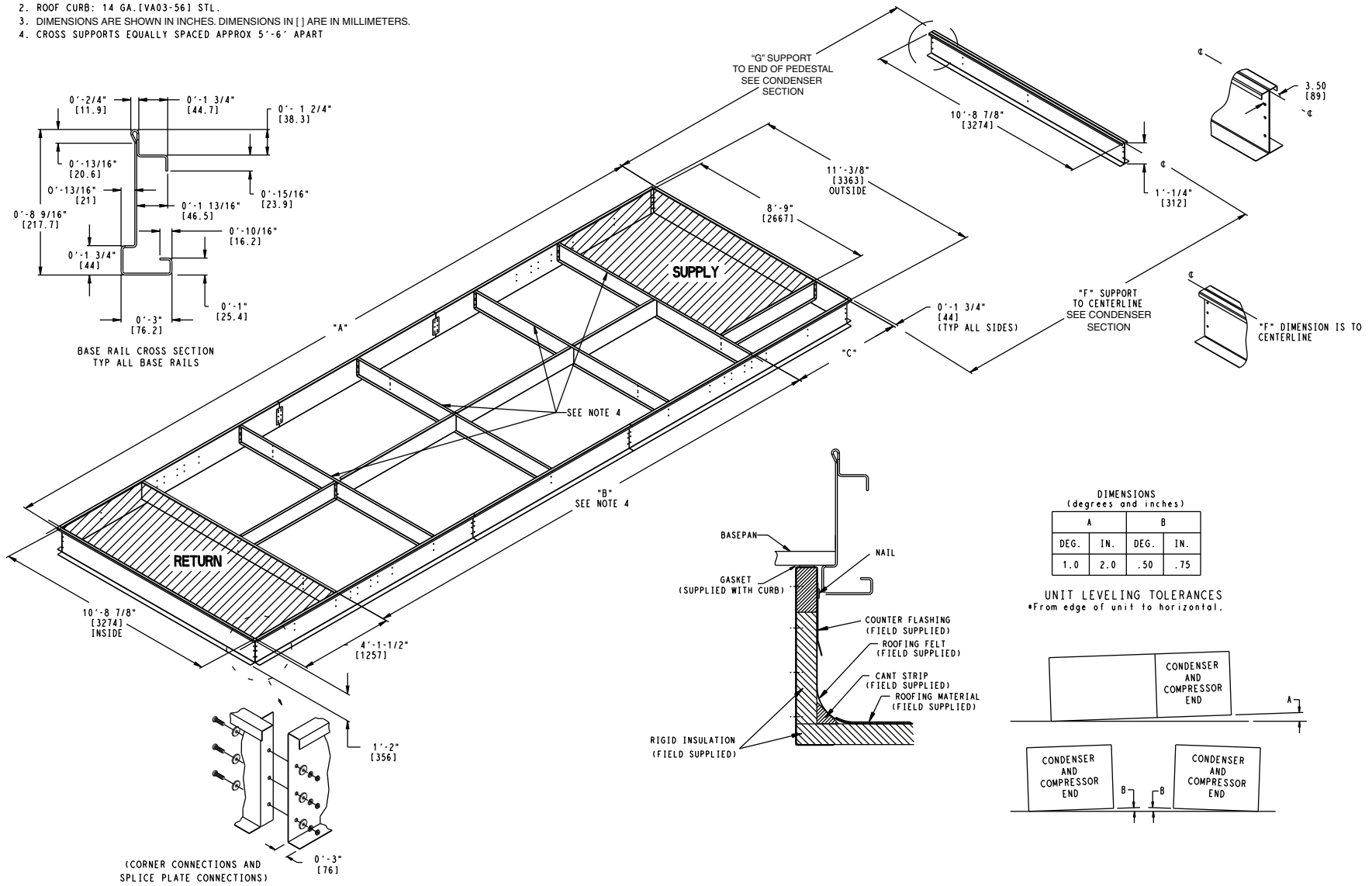
Fig. 3 — Roof Curb Units
