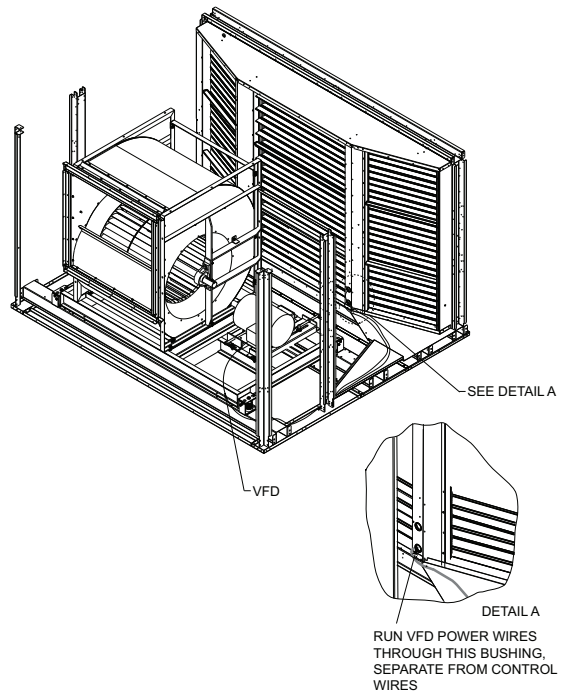
Fig. 44 — Wire Routing
