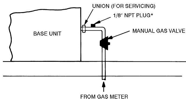
Fig. 28 — Gas Piping Details
