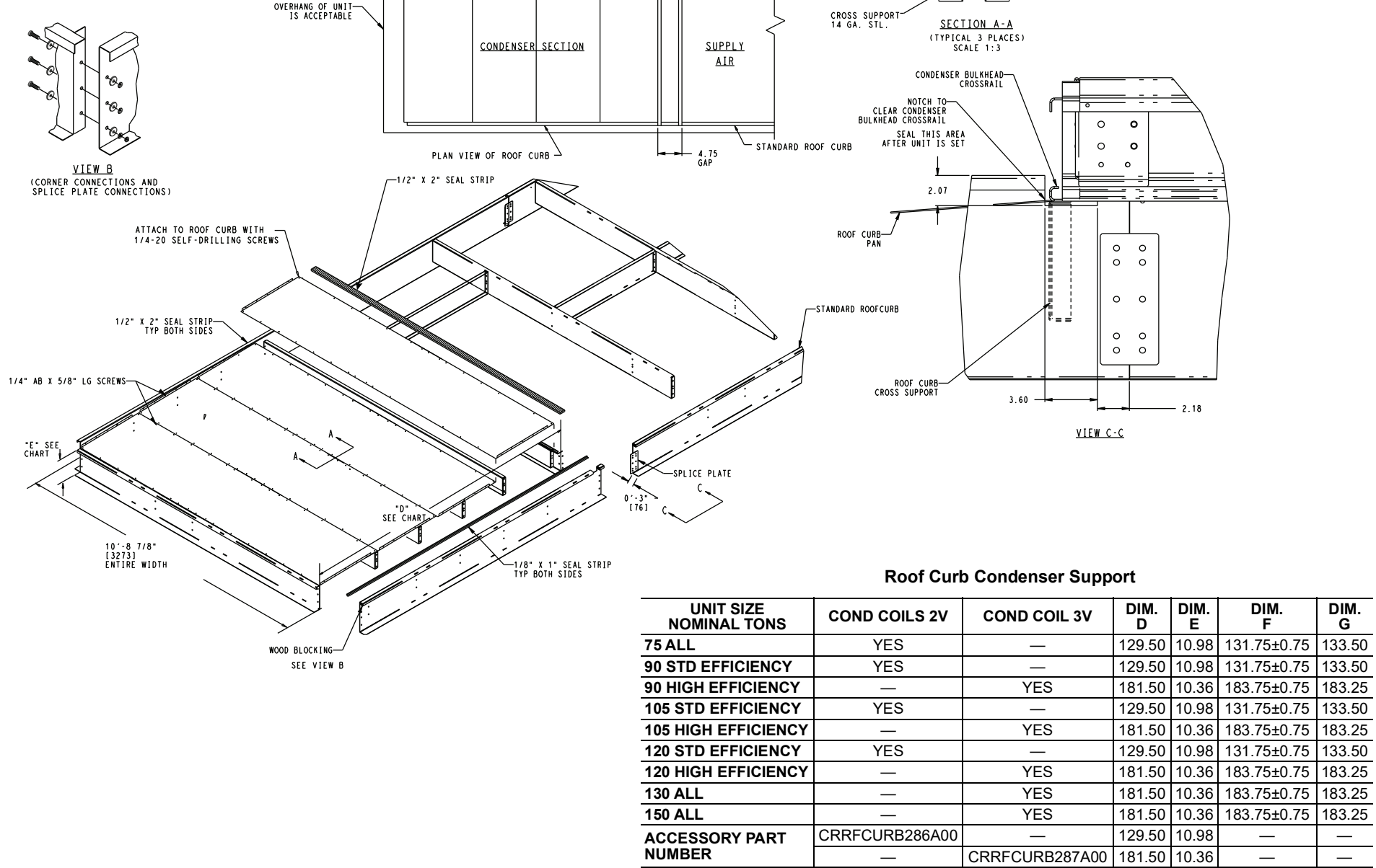
Fig. 3 — Roof Curb Units (cont)
