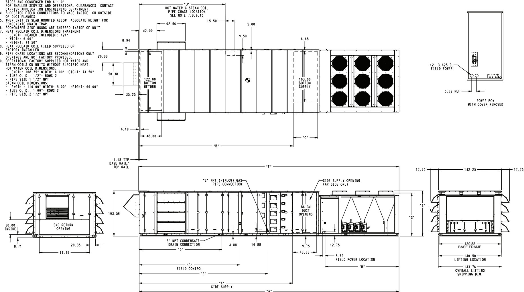
Fig. 12 — 48N Unit Sizes R, S, T (120-150 Ton Nominal Capacity)
