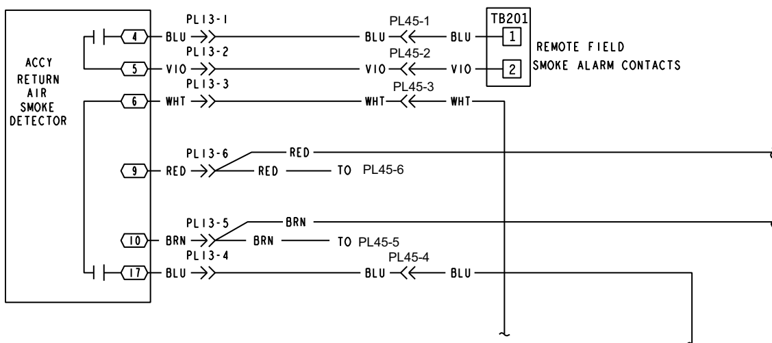
Fig. 57 — Return Air Smoke Detector Wiring
