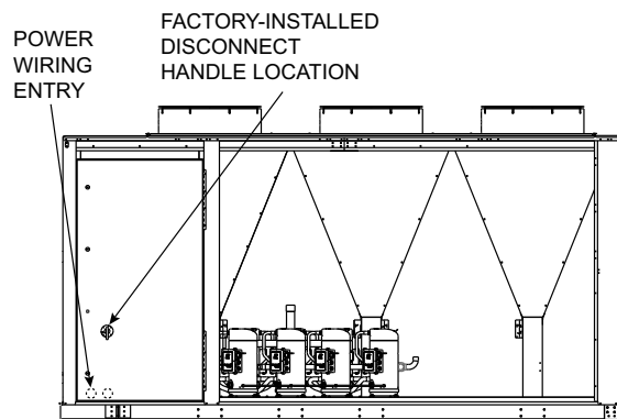
Fig. 22 — Factory-Installed Disconnect Location (End of Unit Shown)
