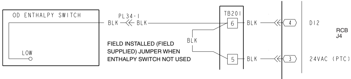
Fig. 51 — Outdoor Air Enthalpy Switch Wiring
