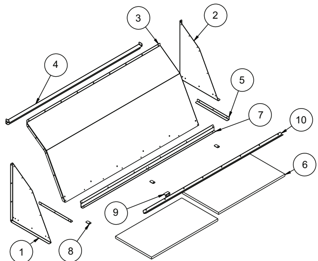
Fig. 19 — Hood Assembly
