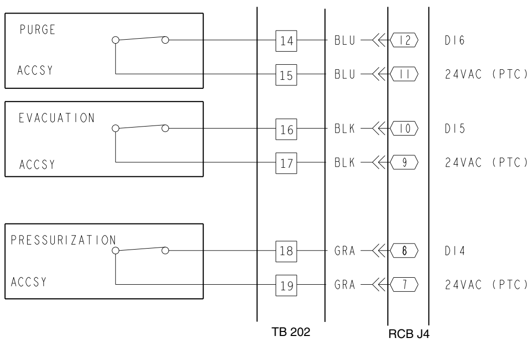
Fig. 59 — Purge, Evacuation, and Pressurization Wiring
