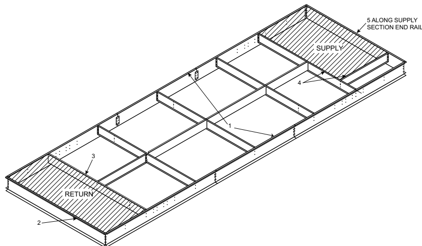
Fig. 5 — Gasket Location on Roof Curb
