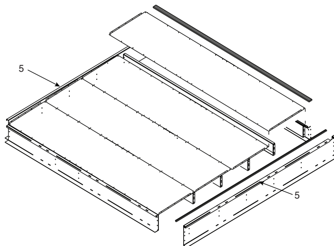
Fig. 6 — Gasket Location — Condenser Section Roof Curb
