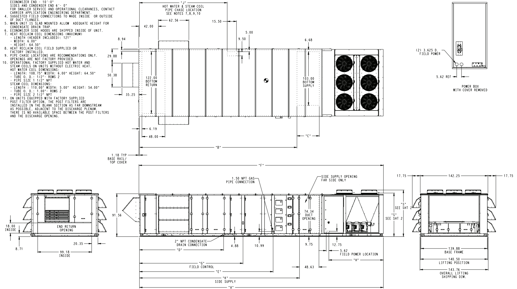
Fig. 11 — 48N Unit Sizes N, P, Q (75-105 Ton Nominal Capacity)
