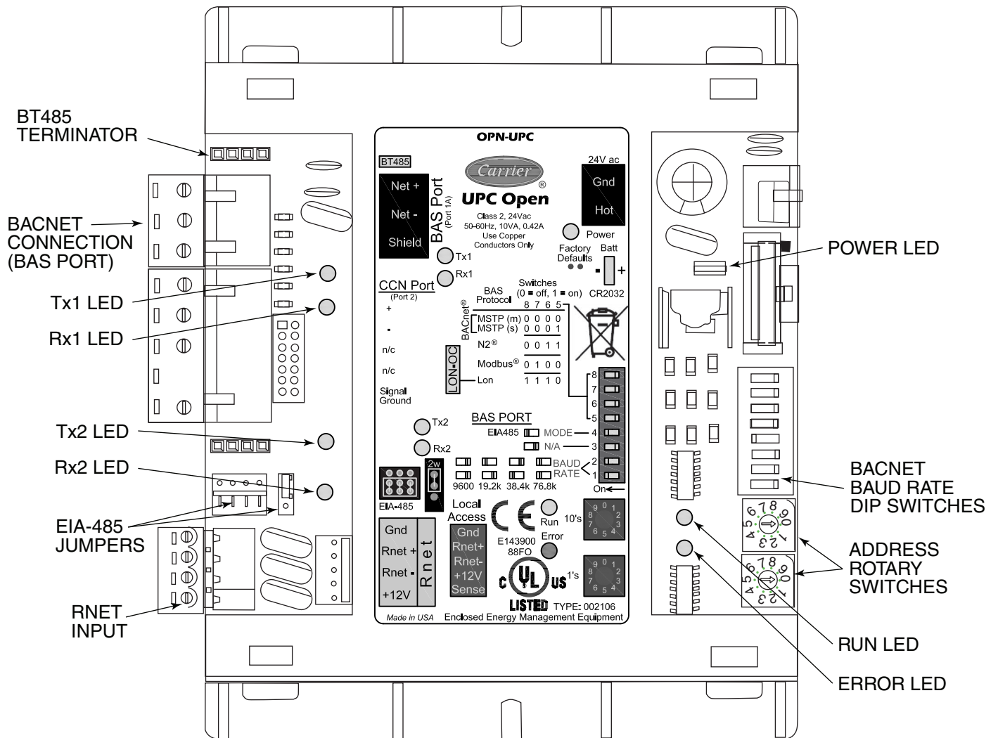
Fig. 61 — UPC Open Controller
