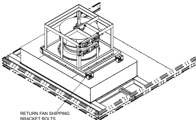
Fig. 26 — Return Fan Shipping Bracket Bolts
