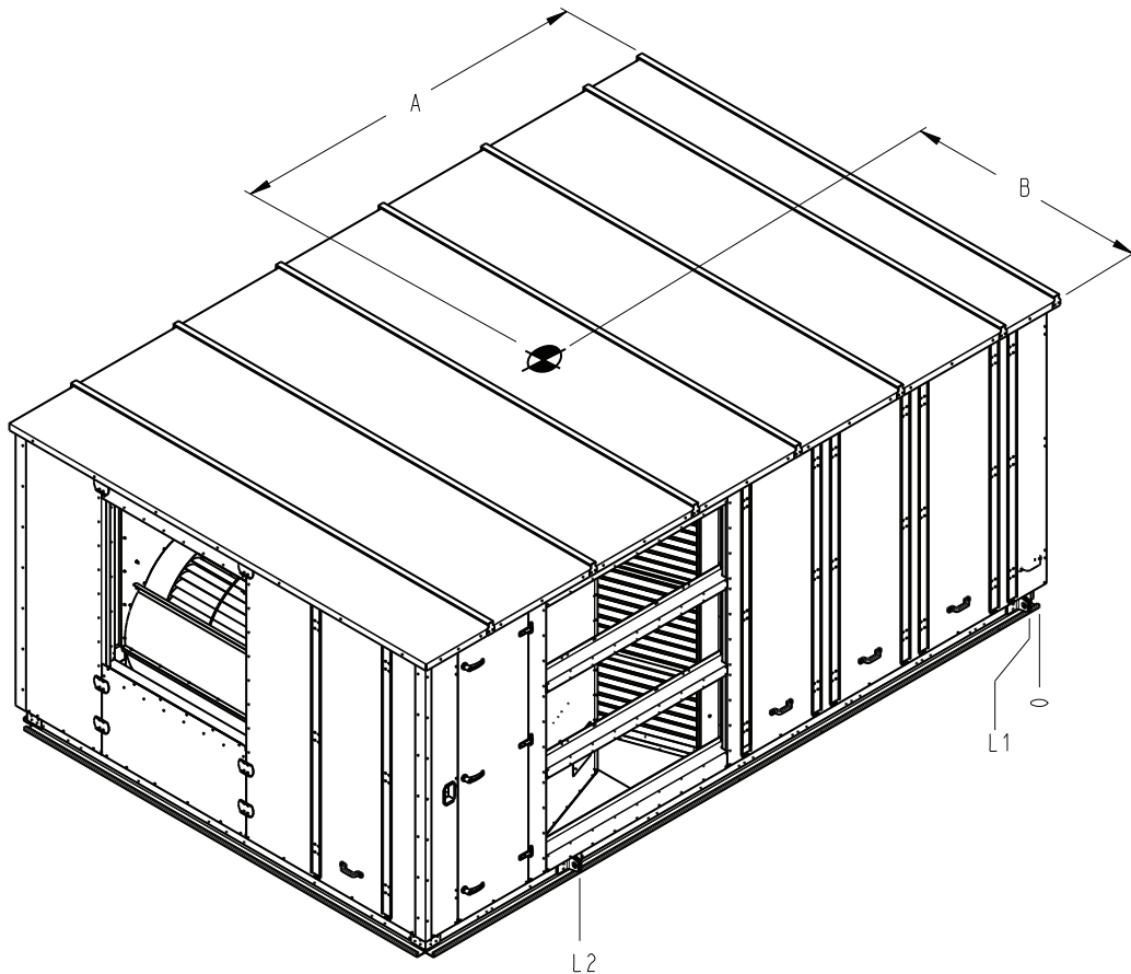
Fig. 9 — 48N 75-150 Ton Split (Return Section) Rigging
