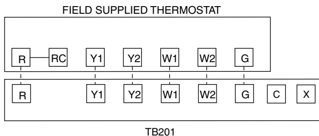
Fig. 47 — Field Control Thermostat Wiring
