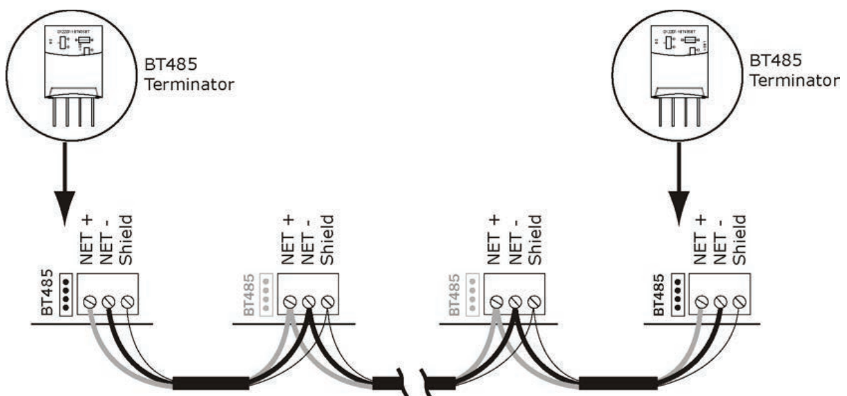
Fig. 62 — Open System Network Wiring
