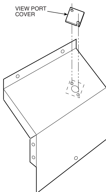
Fig. 32 — Inlet Hood View Port Cover Installation (14 in.)
