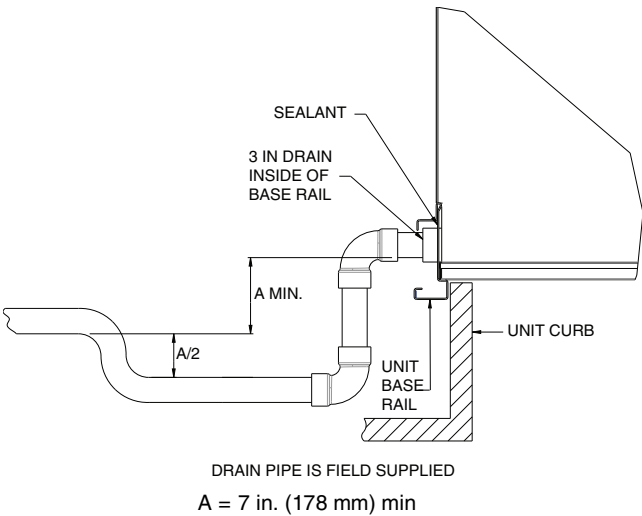
Fig. 15 — Condensate Drain Piping Details (Slab and Curb Mounted)
