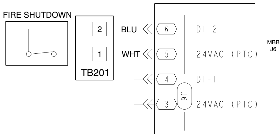
Fig. 58 — Fire Shutdown Wiring
