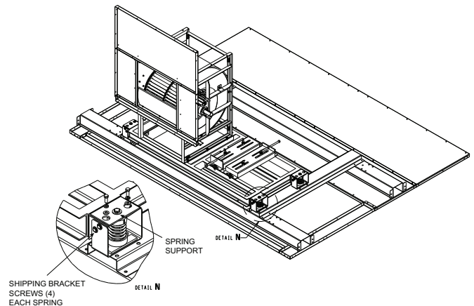
Fig. 27 — Supply Fan and Power Exhaust Fan Shipping Bracket Bolts
