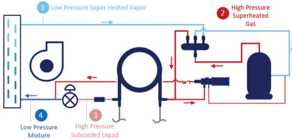
Hot Gas Bypass (HGBP)
