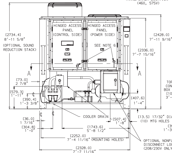
END VIEW
