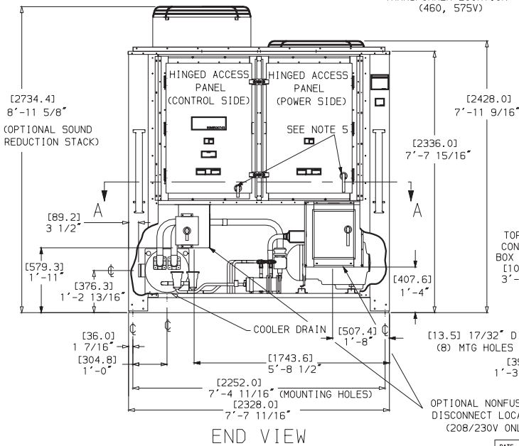
END VIEW
