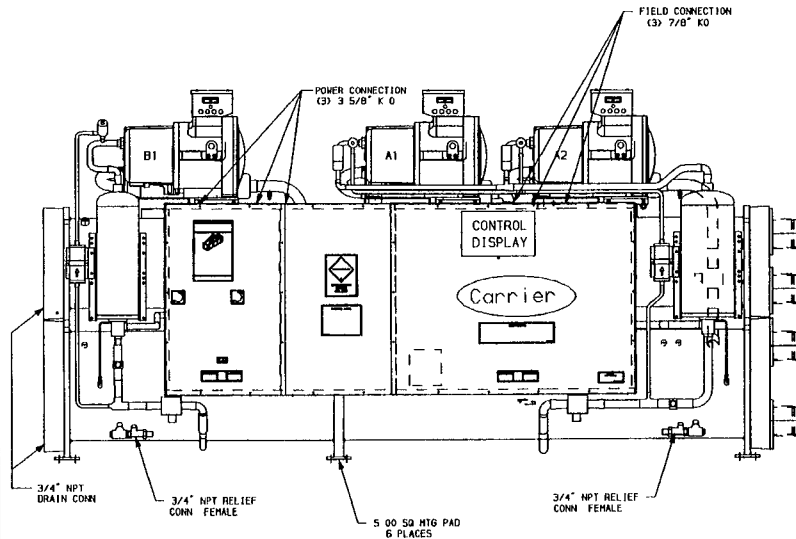
UNIT WITH SOUND ENCLOSURE ACCESSORY (NOT TO SCALE)
