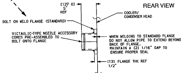
DETAIL "A" NOZZLE ACCESSORY, TYPICAL
