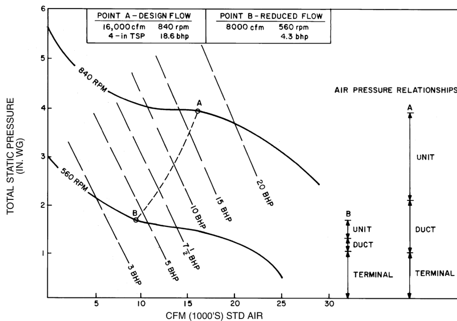
Variable Frequency Fan Speed Control
