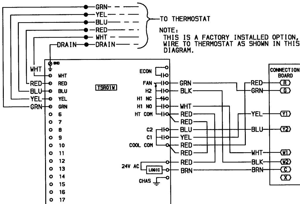
APOLLO AND THERMOSTAT WIRING (48GJ008, 012)
