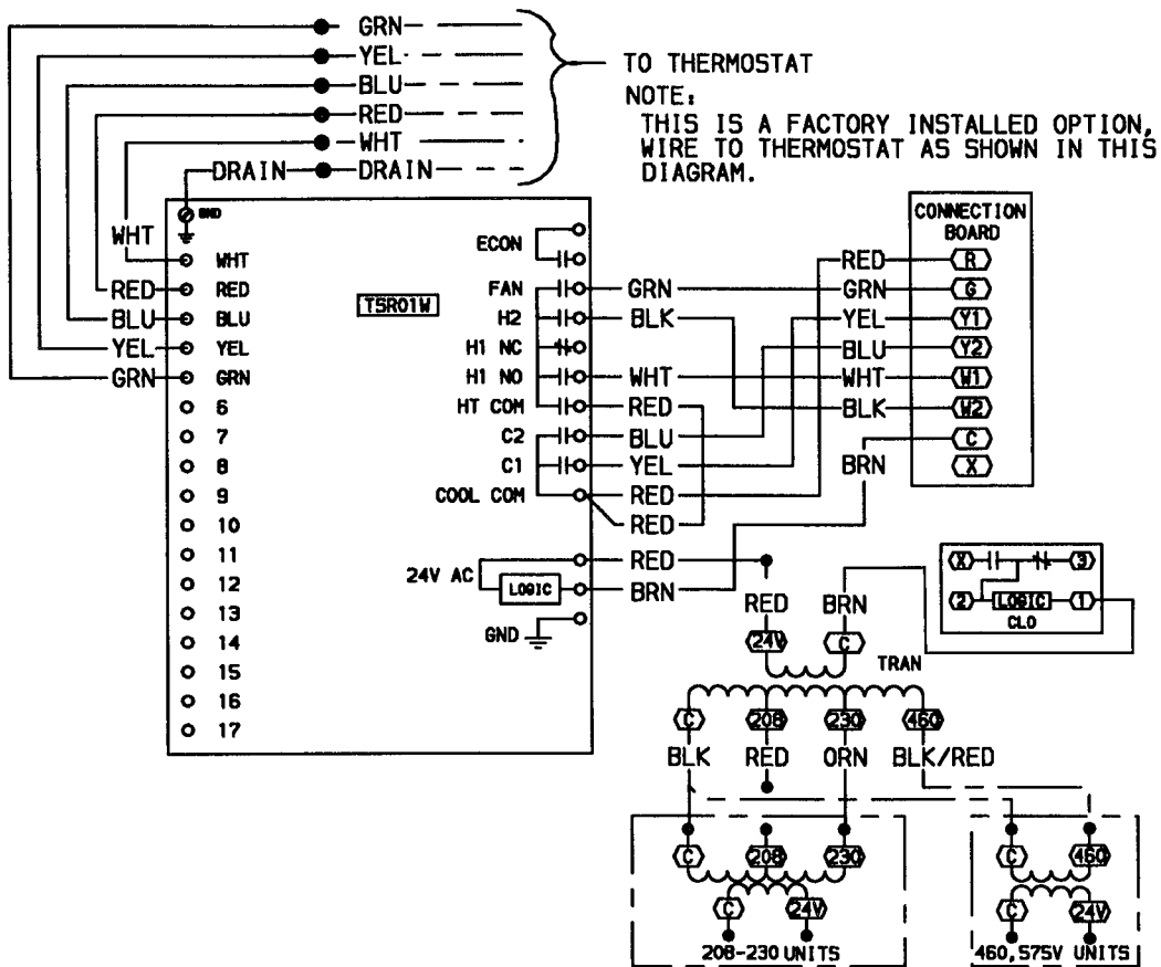
APOLLO AND THERMOSTAT WIRING (48GJ008, 012)
