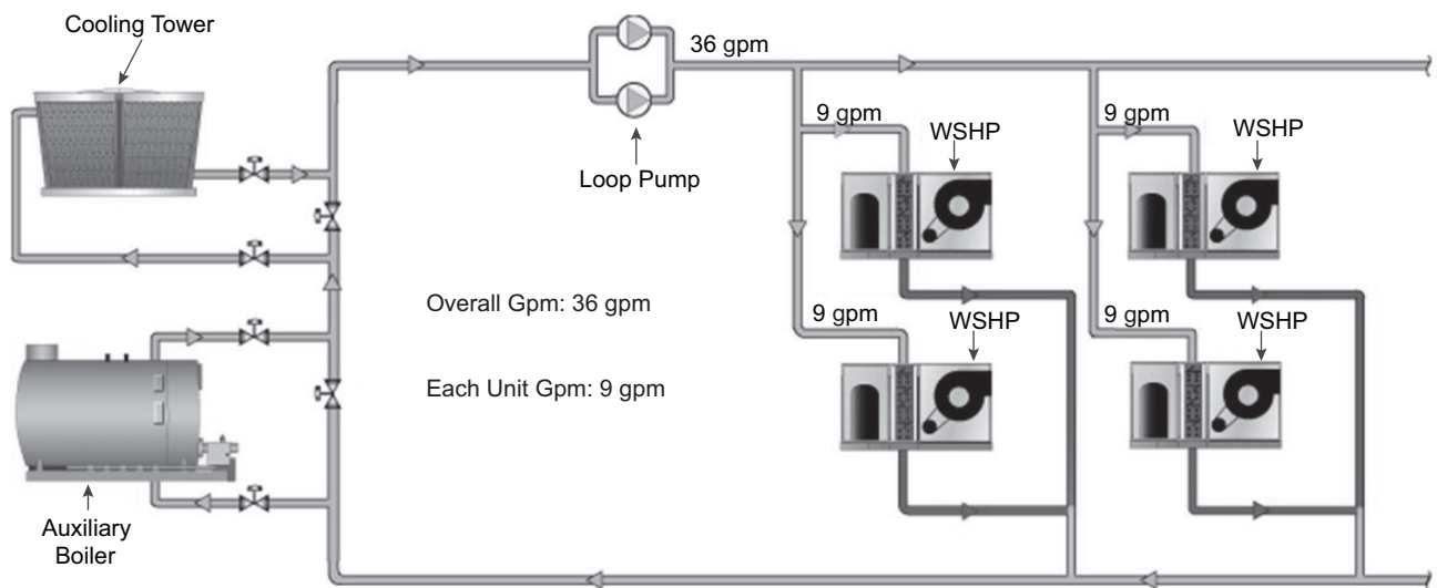
Fig. 13 — Standard Closed Water Loop System with Boiler and Cooling Tower
