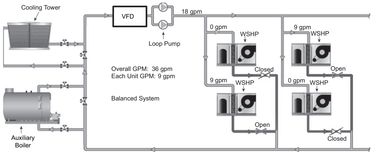
Fig. 15 — Water Loop System with Autoflow Regulator and Solenoid Valve
