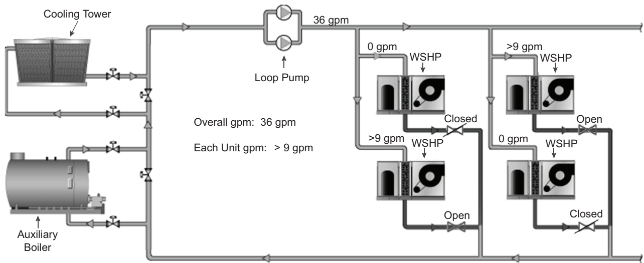
Fig. 14 — Water Loop System with Isolation Valves
