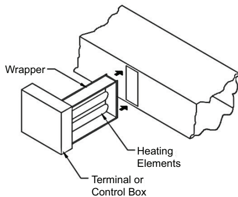
Fig. 10 — Slip-In Heater
