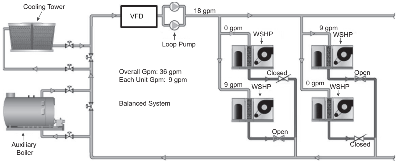
Fig. 16 — Water Loop System with Variable Frequency Drive
