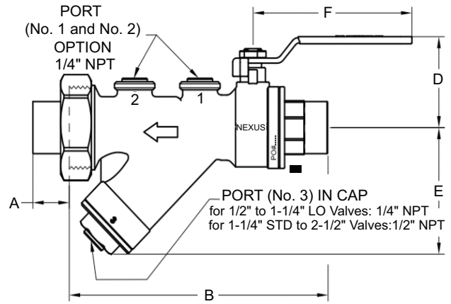
Fig. 8 — Strainer and Ball Valve Dimensions
