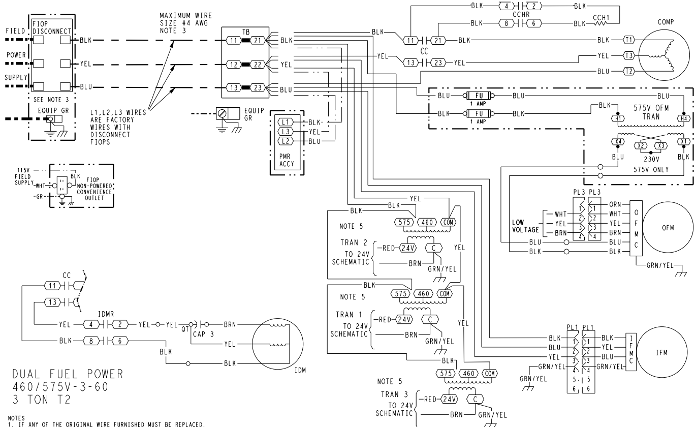
Typical Power Wiring Diagram — 549Q 04 460/575-3-60 Units Shown
