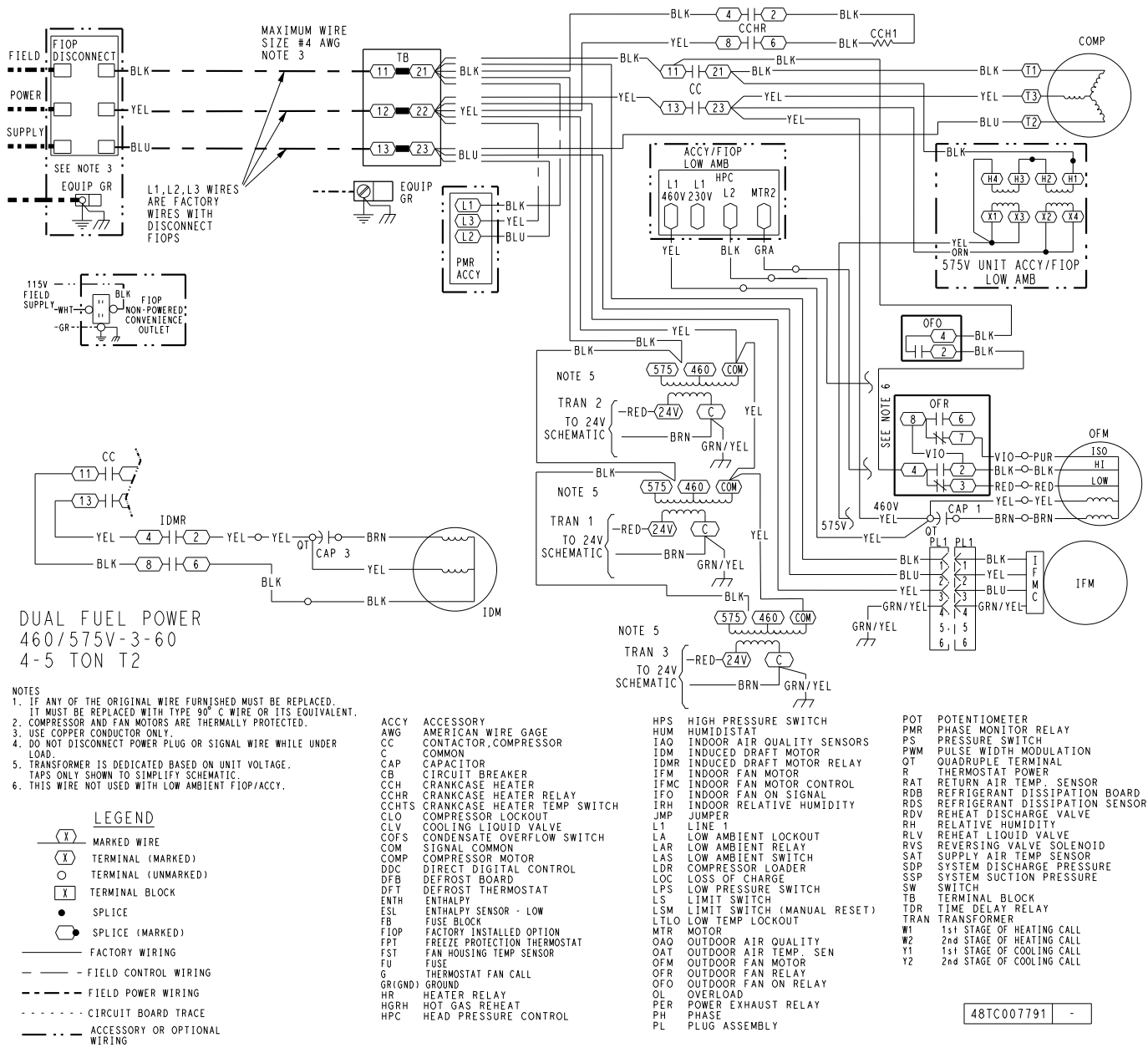
Typical Power Wiring Diagram — 549Q 05-06 460/575-3-60 Units Shown
