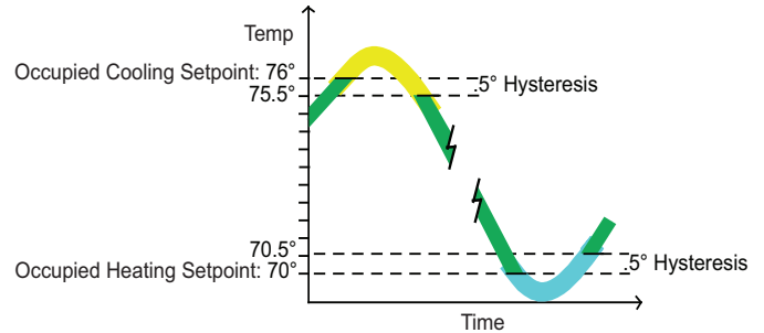
Fig. 11 — Hysteresis Example
