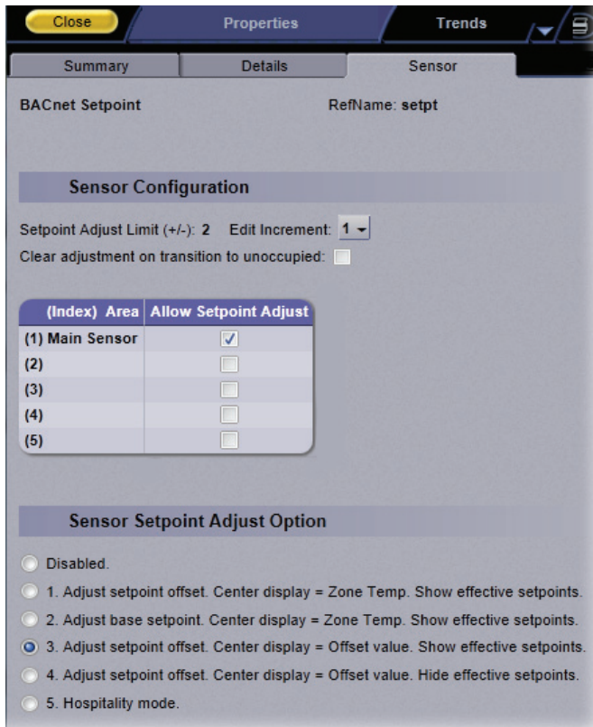
Fig. 15 – Adjusting Setpoints
