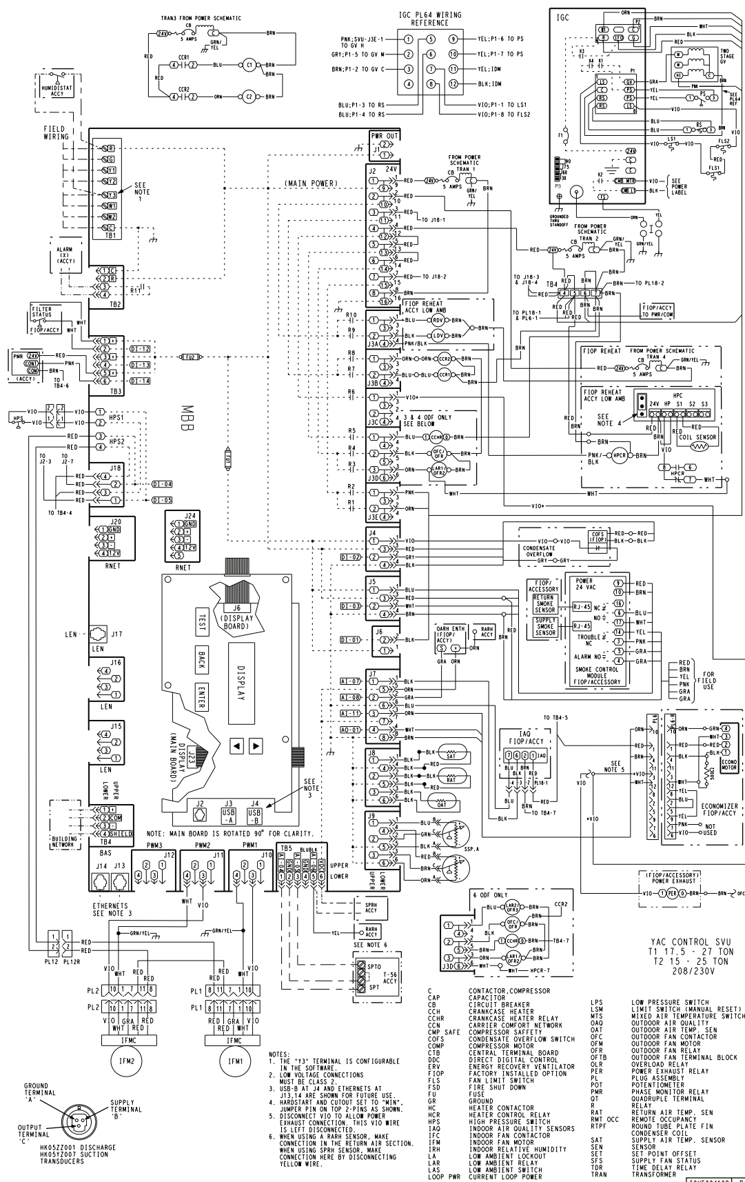
48FC**20-30 Control Wiring Diagram, SystemVu™ Controller
