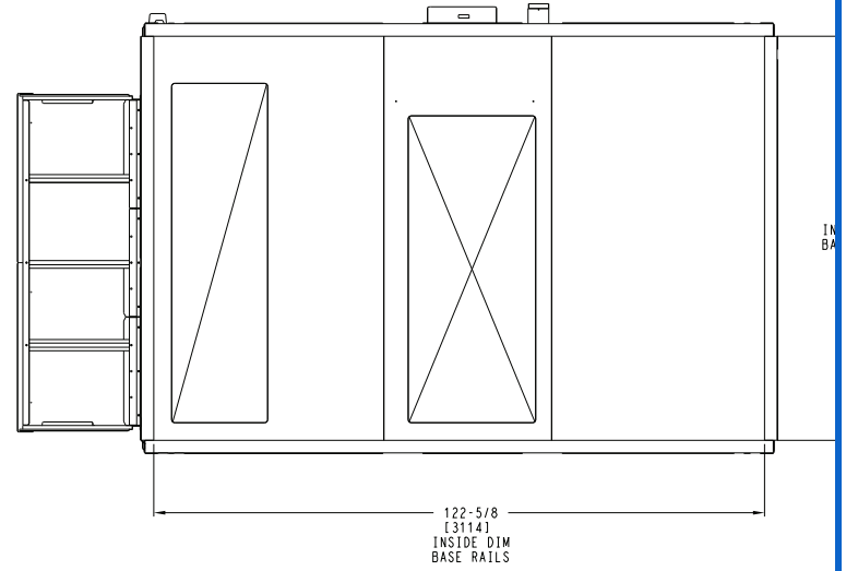
BOTTOM INSIDE BASERAIL DIMENSIONS
