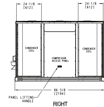
DEDICATED HORIZONTAL AIRFLOW UNIT 30 SIZE
