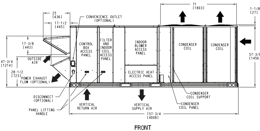
DEDICATED VERTICAL AIRFLOW UNIT 30 SIZE
