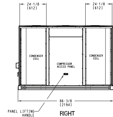
DEDICATED VERTICAL AIRFLOW UNIT 30 SIZE
