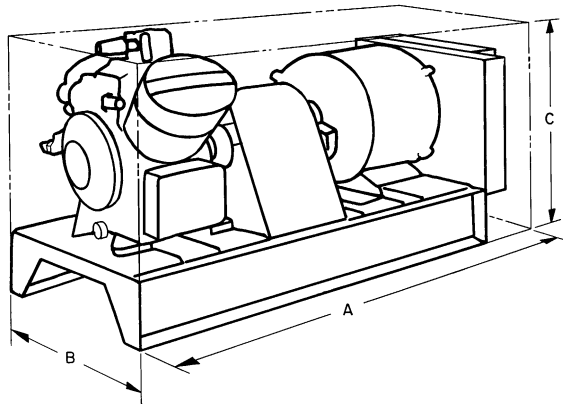
COMPRESSOR UNIT, DIRECT DRIVE (DD)
