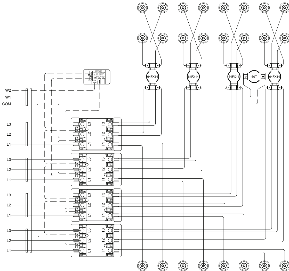
Fig. W — CRHEATER451A Wiring Assembly
