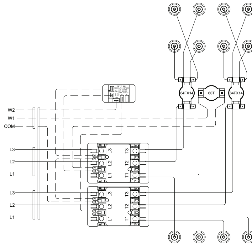
Fig. U — CRHEATER413A, 414A, 415A, 421A, 422A, 423A, 424A, 427A, 428A Wiring Assembly
