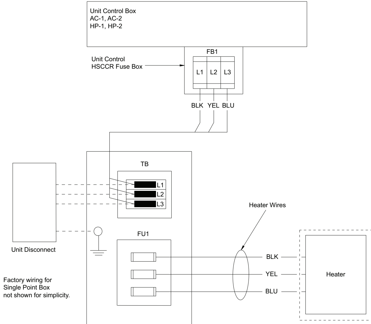
Fig. P — AC/HP Single Point Box 064A00 and 067A00 (AC-1: Sizes 08-16; AC-2: Sizes 07-14; HP-1: Sizes 09-14; HP-2: Sizes 07-12)
