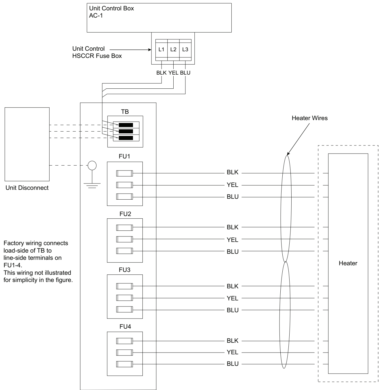
Fig. S — AC Single Point Box CRSINGLE070A00, 073A00
