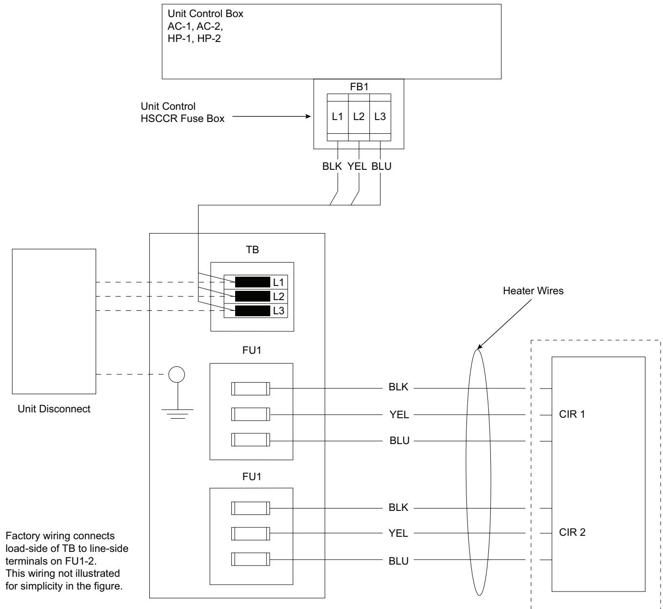
Fig. Q — AC/HP Single Point Box CRSINGLE065A00 and 068A00, 071A00 (AC-1: Sizes 08-16; AC-2: Sizes 07-14; HP-1: Sizes 09-14; HP-2: Sizes 07-12)
