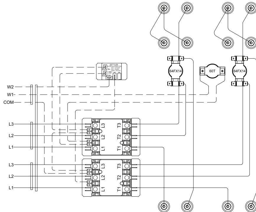
Fig. Y — CRHEATER426A Wiring Assembly
