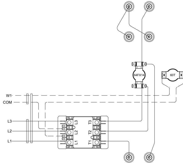
Fig. X — CRHEATER418A, 419A Wiring Assembly
