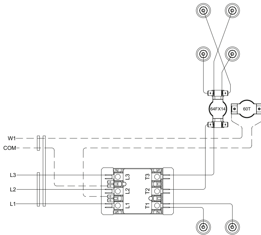
Fig. T — CRHEATER410A, 411A, 412A, 420A, 425A Wiring Assembly
