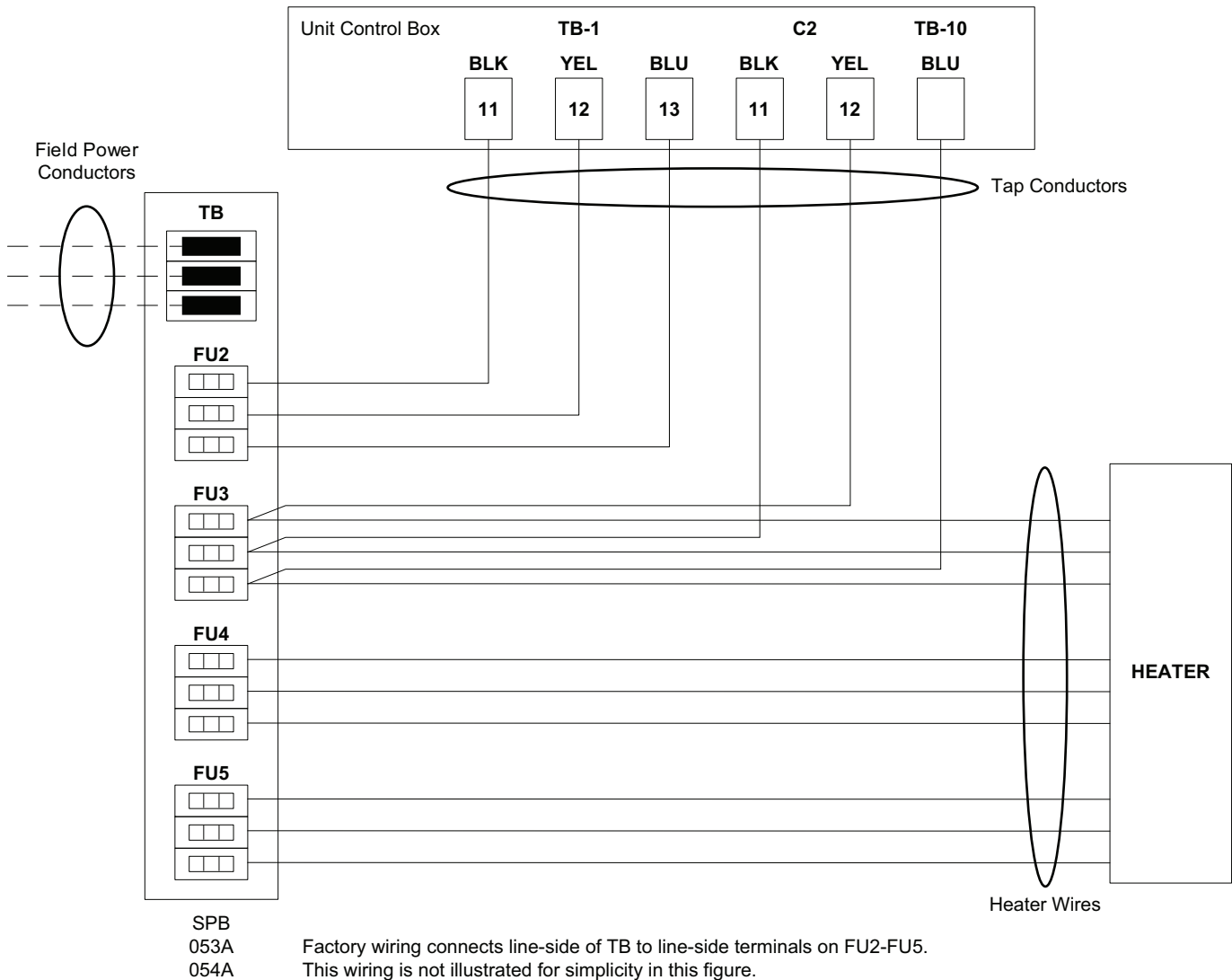
Fig. L — HP Single Point Box CRSINGLE053A00 (HP-1: Sizes 08-12; HP-2: Sizes 08-09) CRHEATER416A00 and 417A00 — 3 Bank
