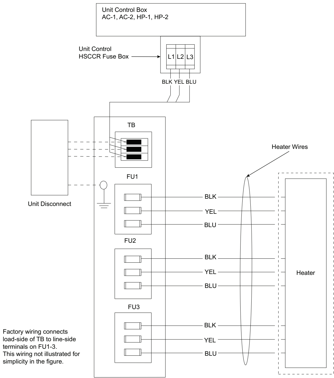
Fig. R — AC/HP Single Point Box CRSINGLE066A00 and 069A00, 072A00 (AC-1: Sizes 09-16; AC-2: Sizes 08-14; HP-1: Sizes 09-14; HP-2: Size 12)
