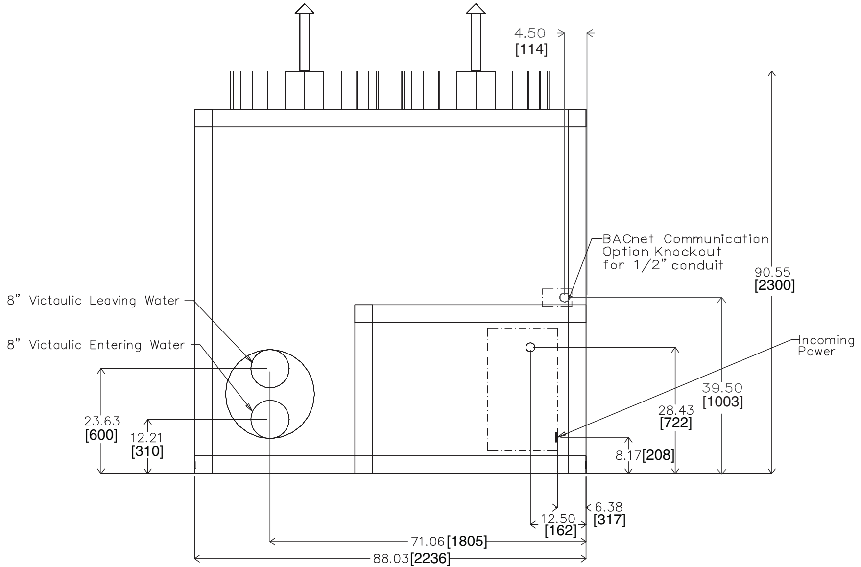
RIGHT END VIEW
