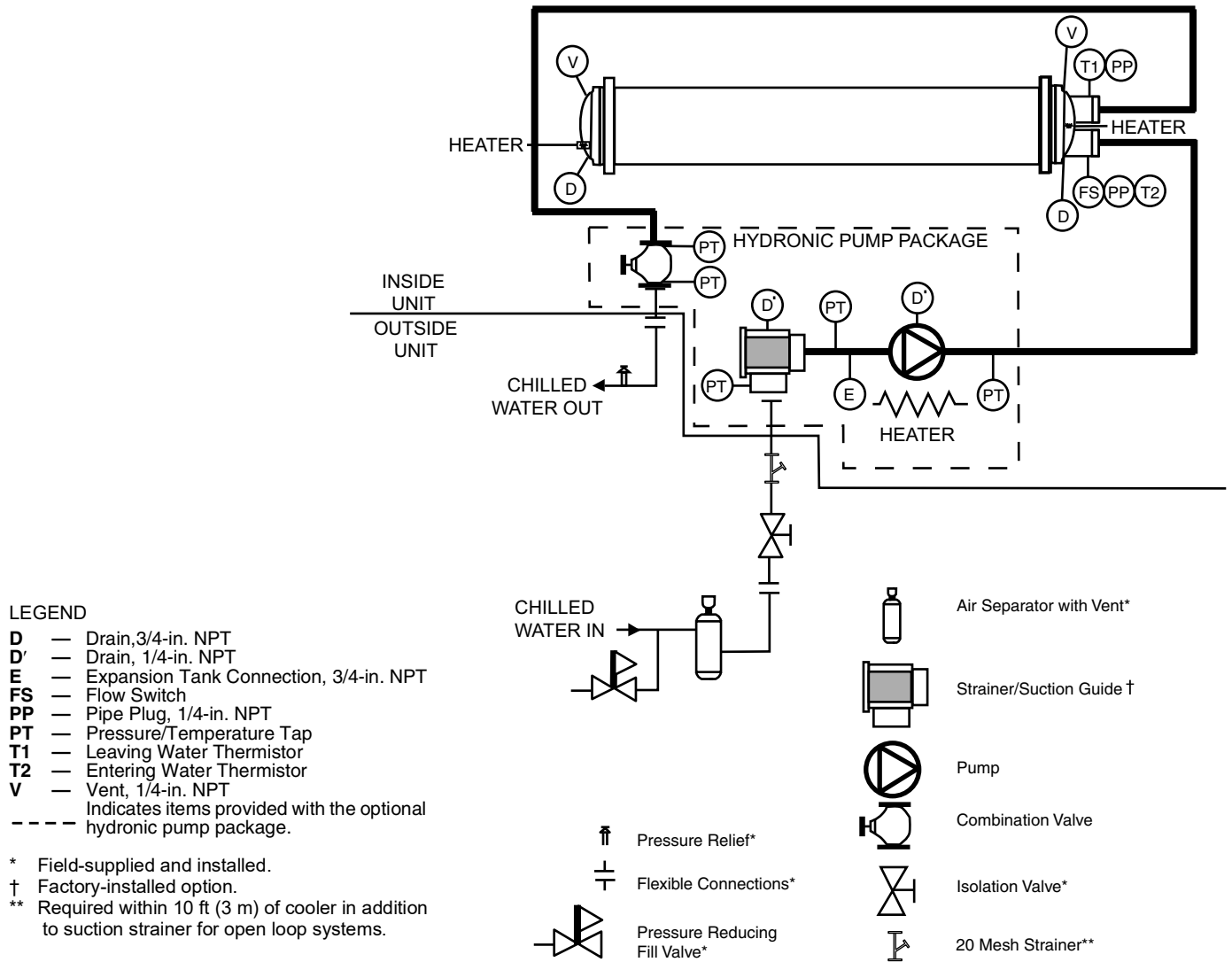
Fig. 46 — Typical Piping Diagram on 30XA Units with Hydronic Package — Single Pump (Flooded Cooler)
