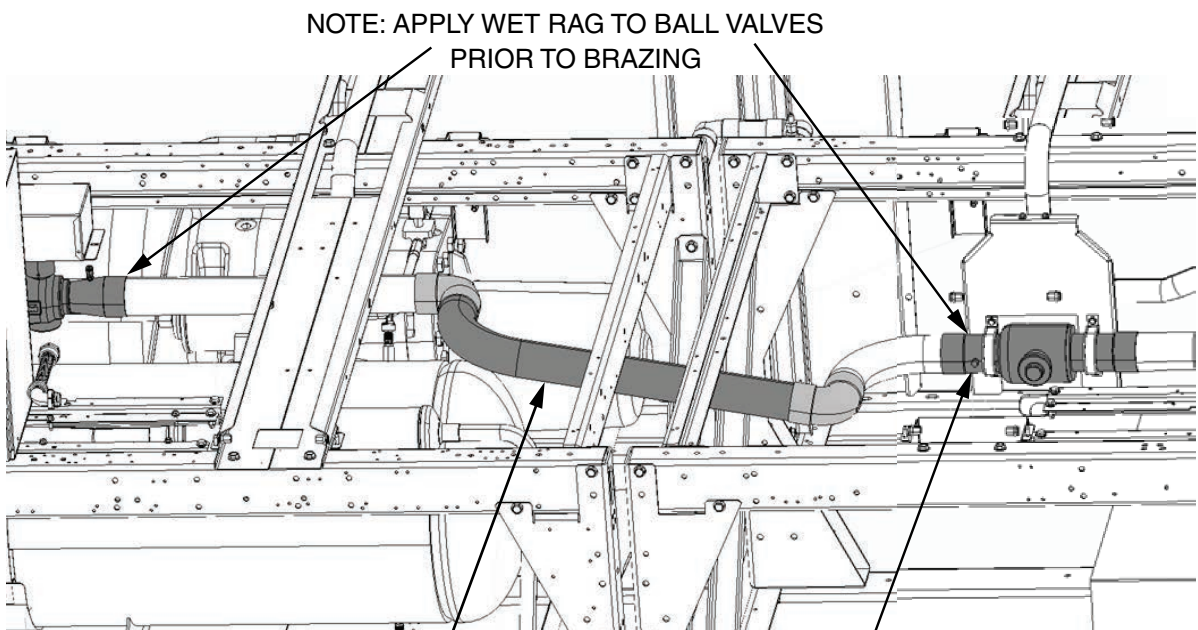
Fig. 31 — 30XA501 Discharge Line Brazed Caps to be Removed
