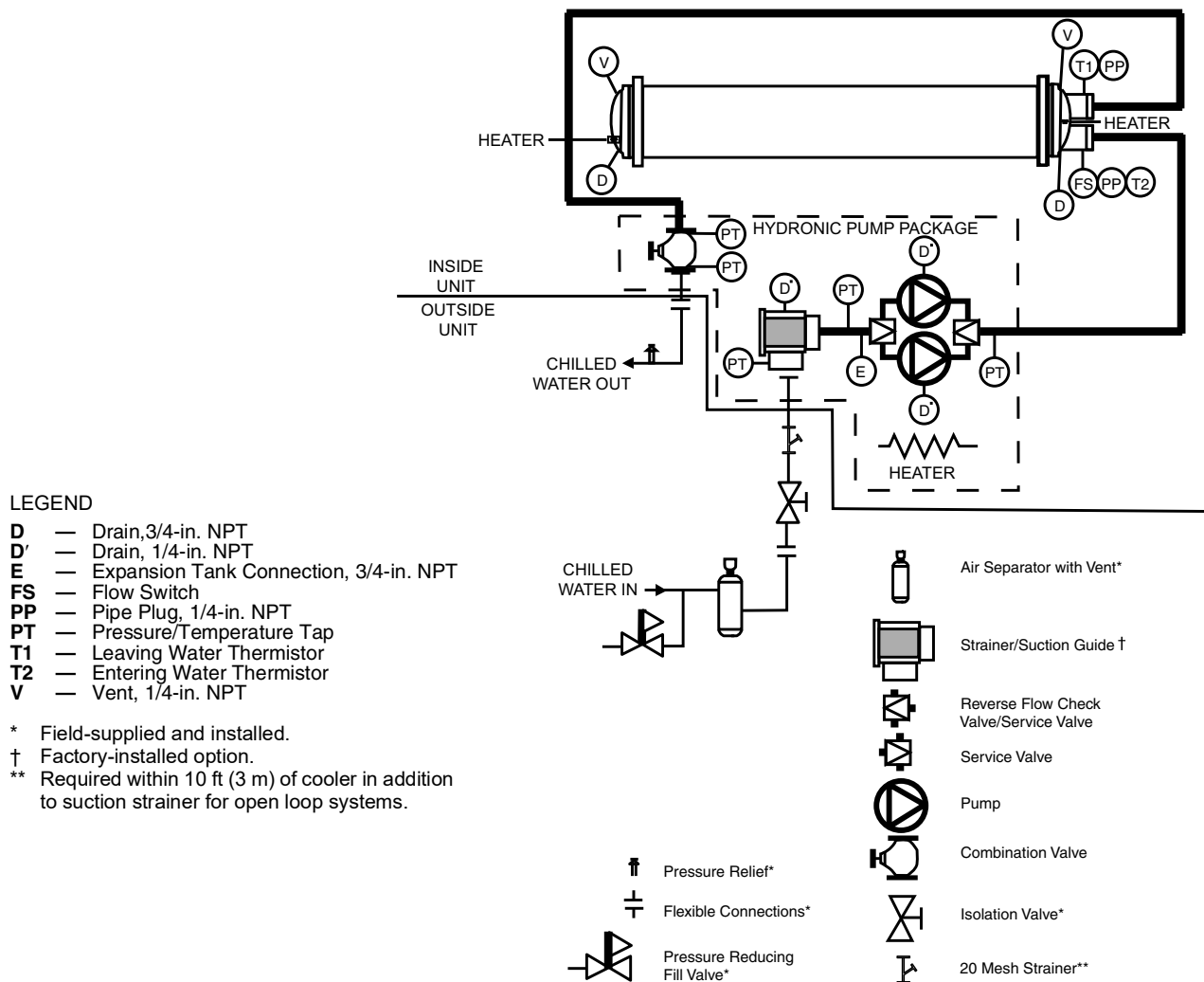
Fig. 47 — Typical Piping Diagram on 30XA Units with Hydronic Package — Dual Pumps (Flooded Cooler)
