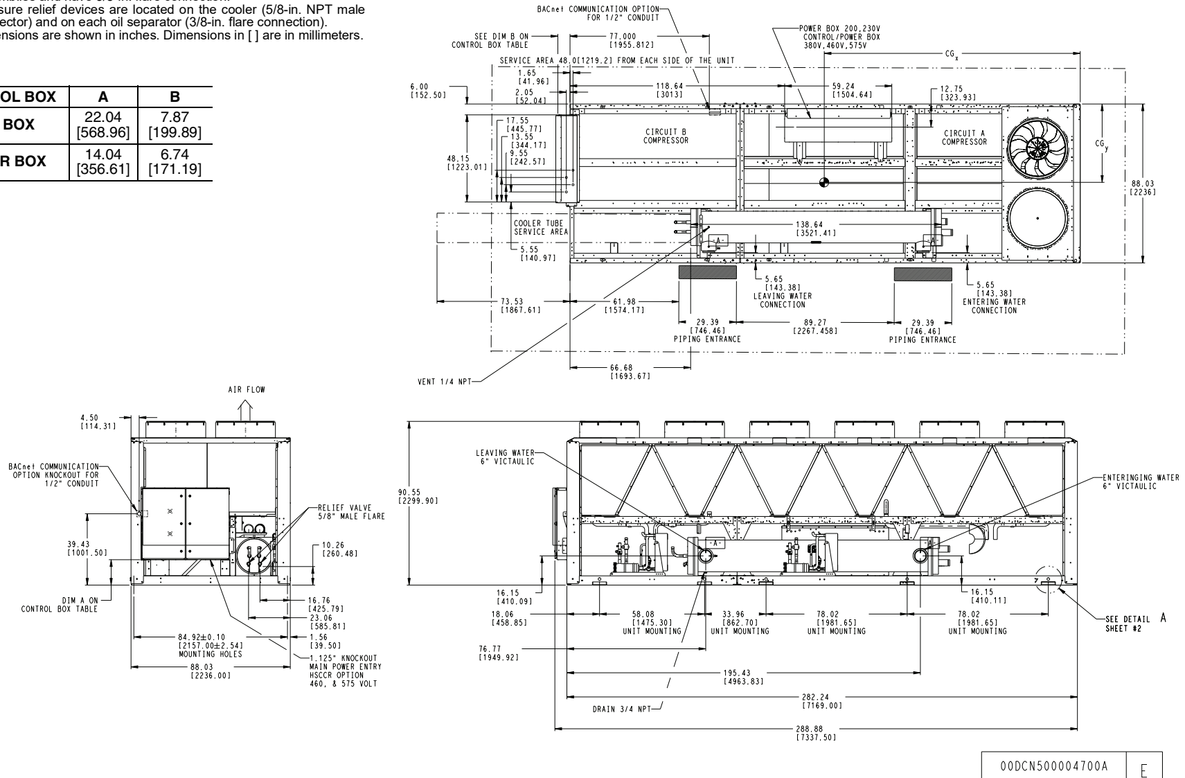
Fig. 12 — 30XA182,202 Air-Cooled Liquid Chiller Dimensions
