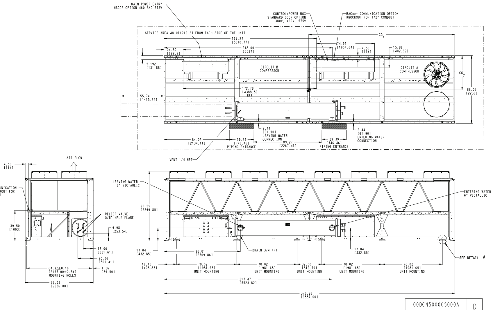
Fig. 16 — 30XA262, 282 Air-Cooled Liquid Chiller Dimensions
