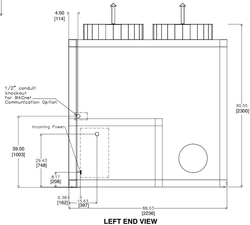
Fig. 8 — 30XA140,160 Air-Cooled Liquid Chiller Dimensions without Pump (cont)
