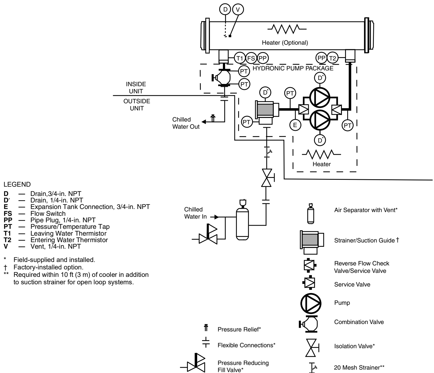
Fig. 53 — Typical Piping Diagram on 30XA DX Cooler Units with Hydronic Package — Dual Pumps
