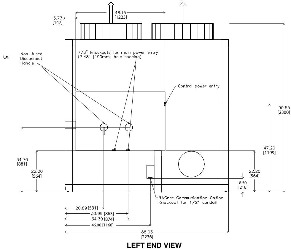
Fig. 2 — 30XA080 Air-Cooled Liquid Chiller Dimensions (cont)
