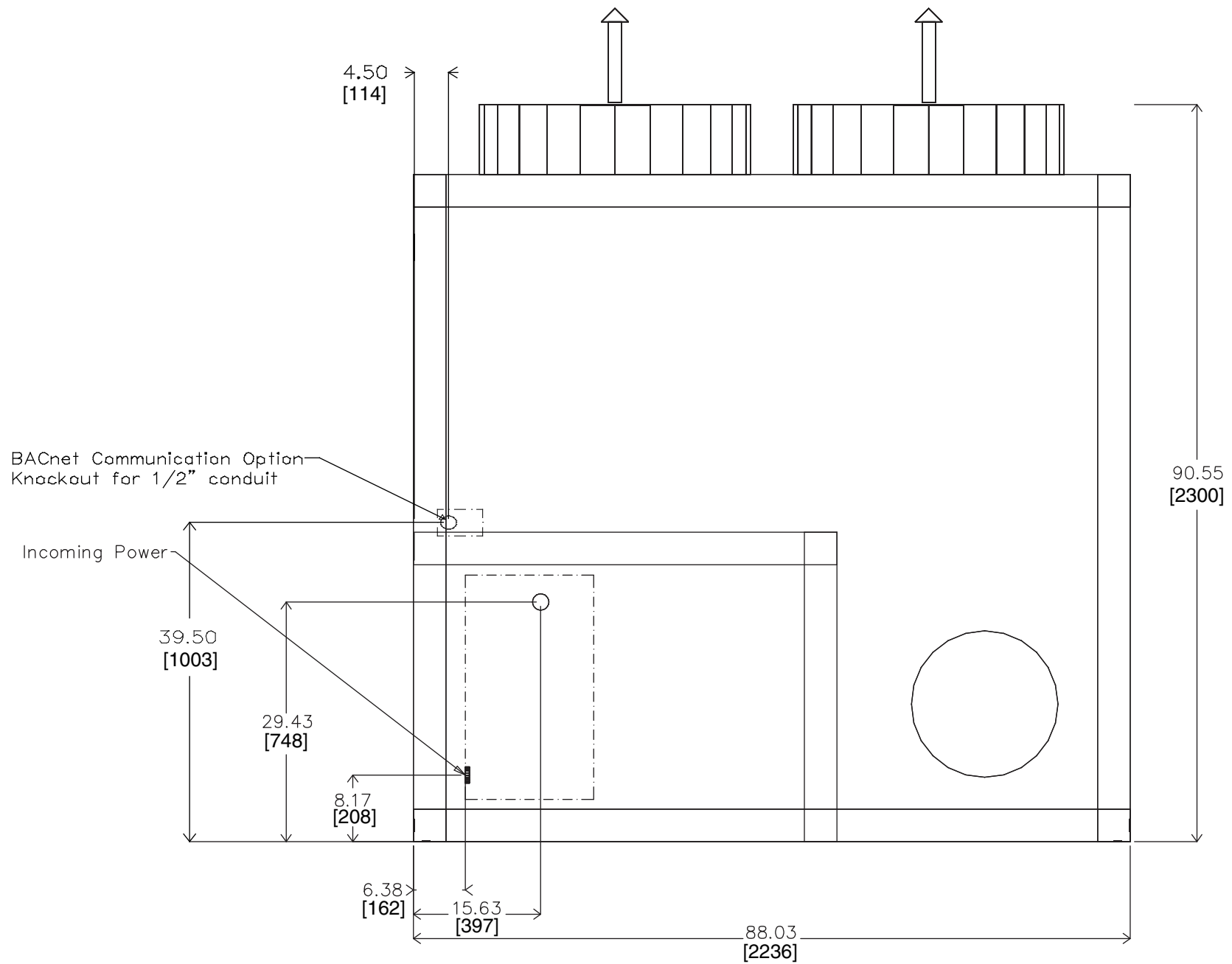
Fig. 13 — 30XA220,240 Air-Cooled Liquid Chiller Dimensions (cont)
