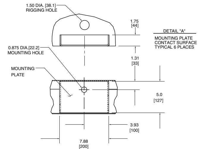
Fig. 4 — 30XA090, 100, 110, 120 Air-Cooled Liquid Chiller Dimensions without Pump (cont)
