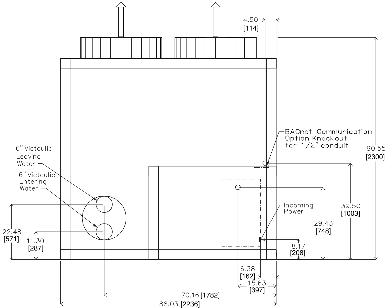
RIGHT END VIEW
