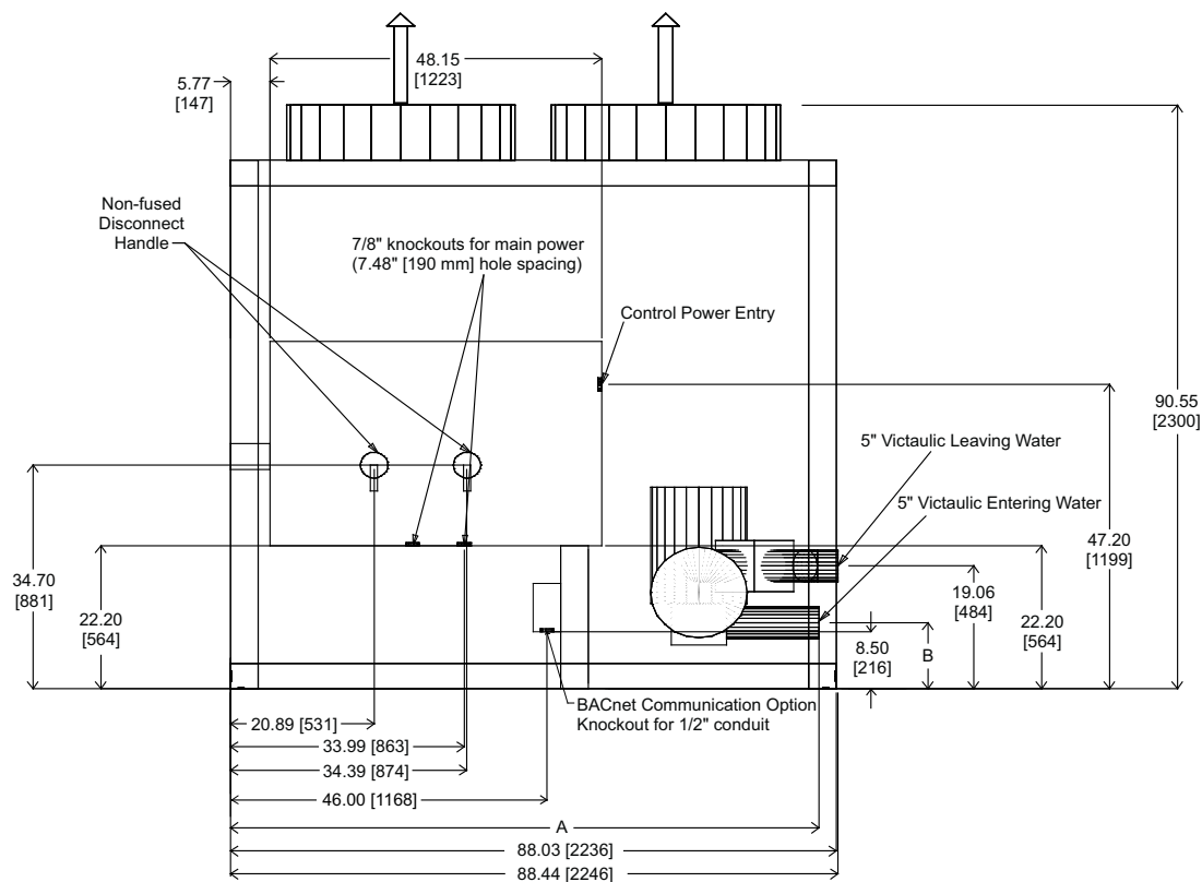
LEFT END VIEW
