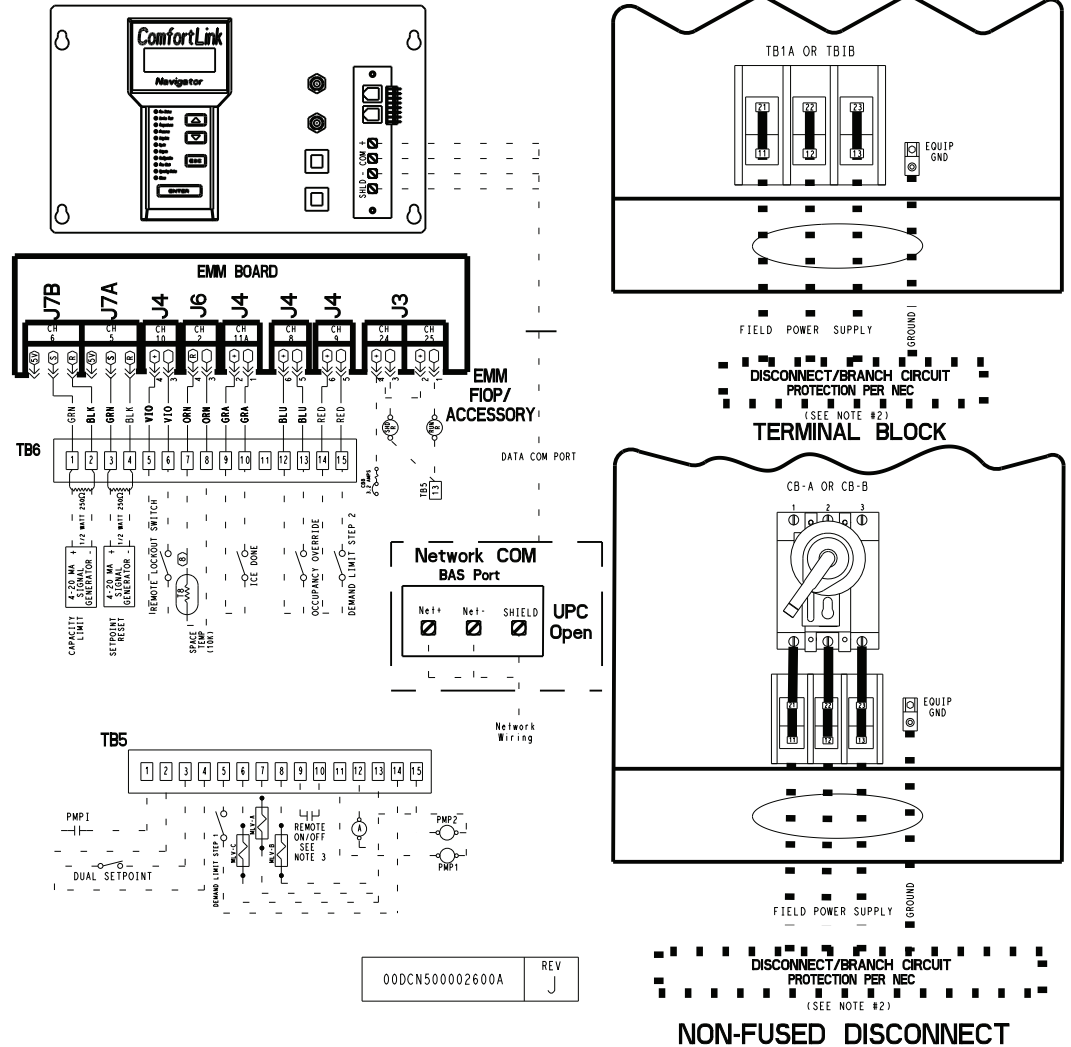
Fig. 61 — Control and Power Wiring Schematic
