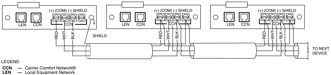
Fig. 62 — TB3 — CCN Wiring Table 19 — CCN Communication Bus Wiring
