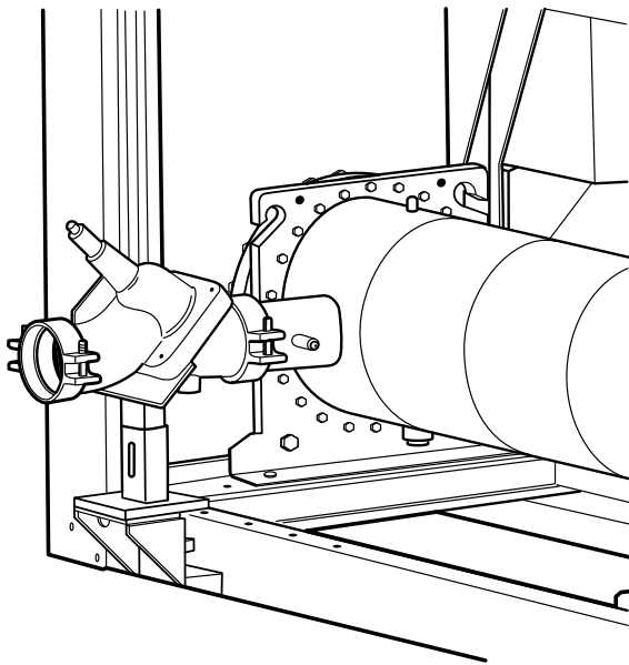
Fig. 55 — Balancing Valve
