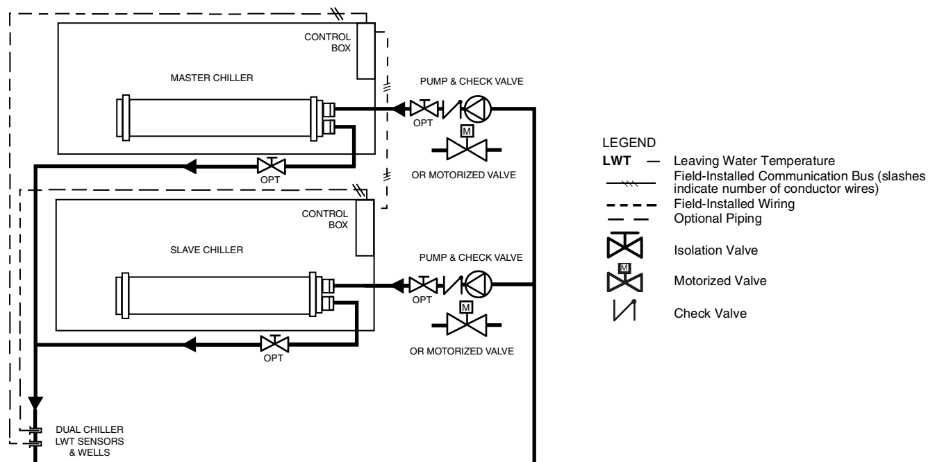
Fig. 50 — Parallel Dual Chiller Operation
