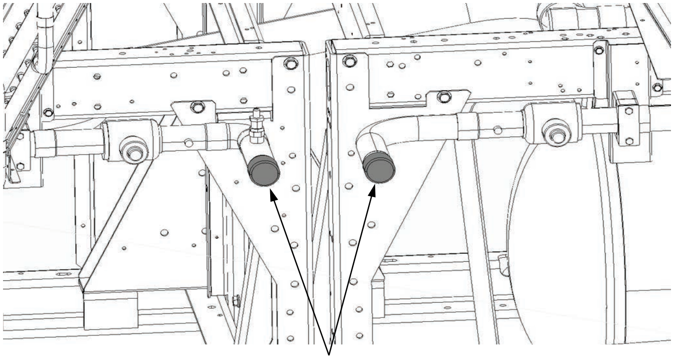
Fig. 34 — 30XA501 Liquid Line Brazed Caps to be Removed
