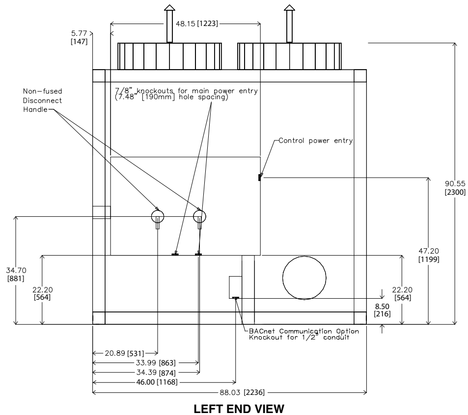
Fig. 4 — 30XA090, 100, 110, 120 Air-Cooled Liquid Chiller Dimensions without Pump (cont)
