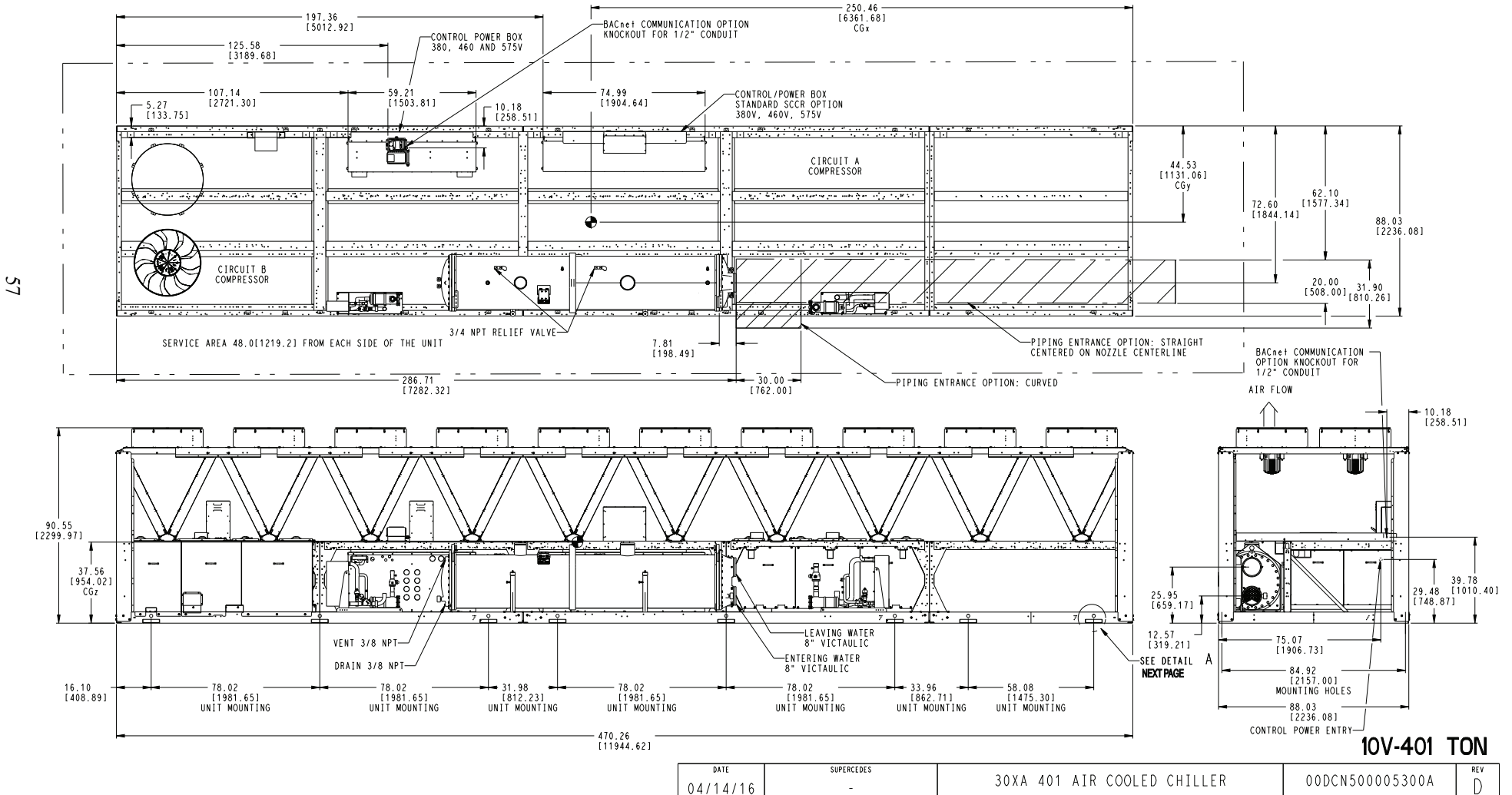
Fig. 20 — 30XA401 Air-Cooled Liquid Chiller Dimensions (See Note 4)
