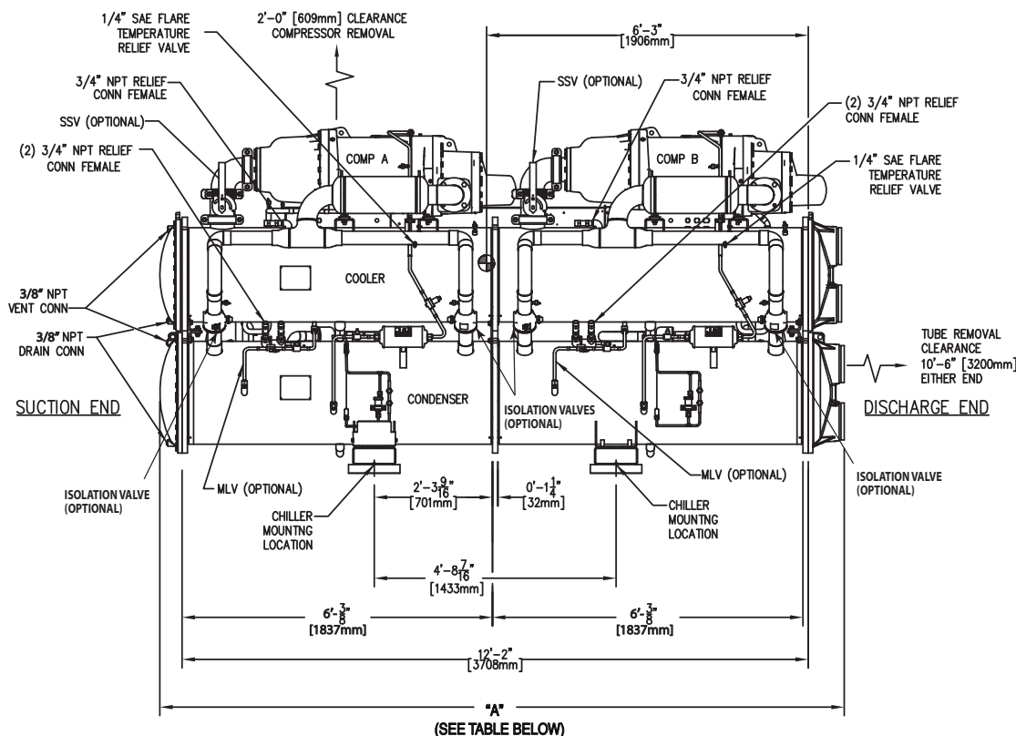
CHILLER DIMENSIONS
