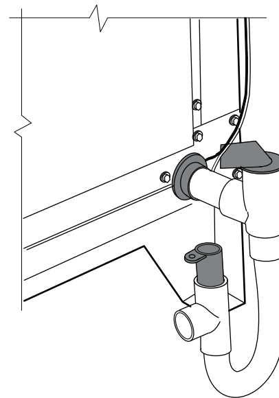
40RF/40RU with Condensate Trap
