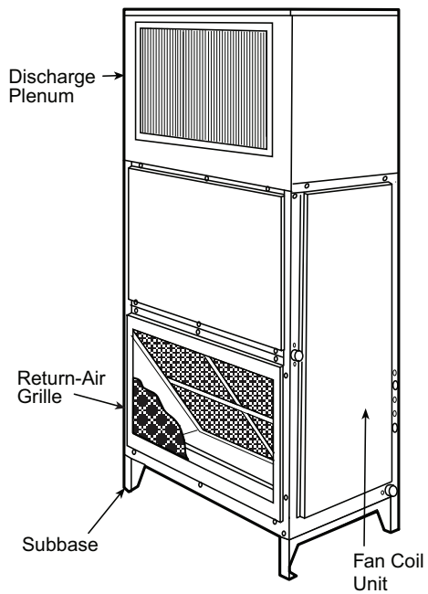
40RF/40RU with Discharge Plenum Return-Air Grille and Subbase
