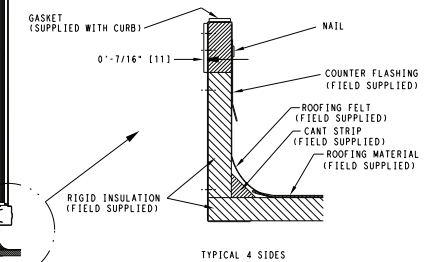
TYPICAL 4 SIDES
