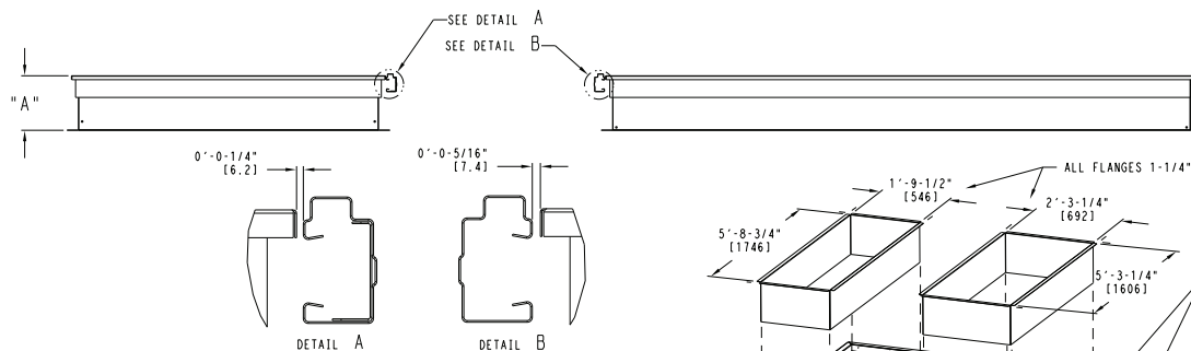
TYPICAL 4 SIDES
