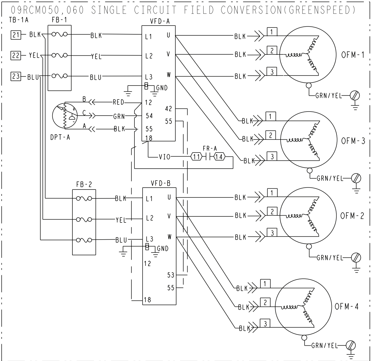
Fig. 36 — Greenspeed Controller Wiring (09RC060 Units Shown)
