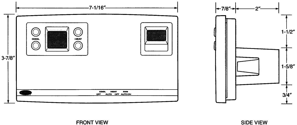
Fig. 1 — Monitor Thermostat or TEMP System Thermostat with Timeclock
