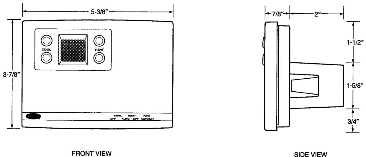
Fig. 2 — Monitor Thermostat or TEMP System Thermostat Without Timeclock, Zone Controller, and Bypass Controller
