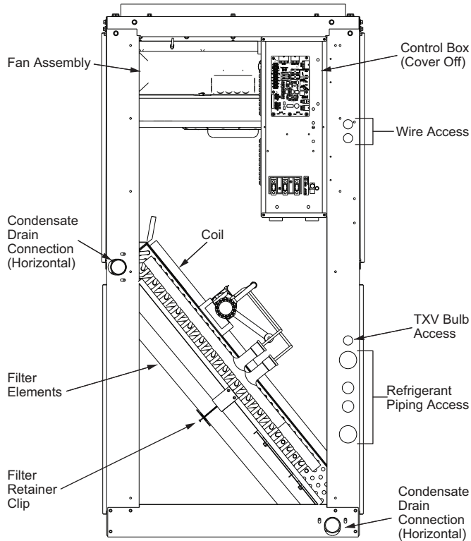
Fig. 14 — Wiring and Service Access (Side Panel Removed)
