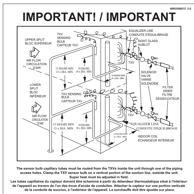
Fig. 19 — TXV Bulb Location Label
