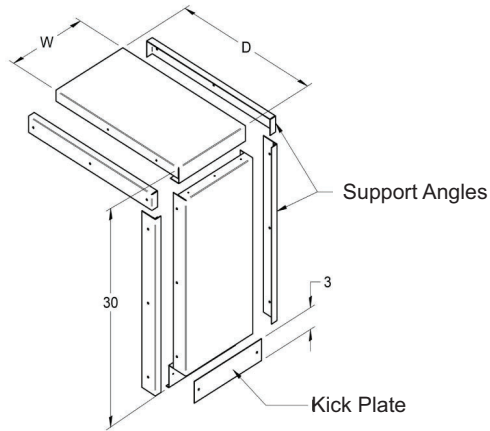
Flat Top Filler Section for Standard Height Units
