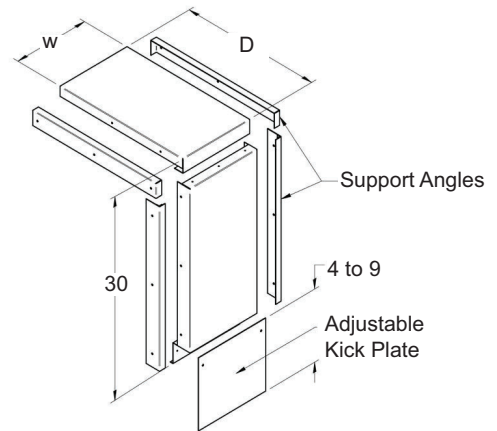
Flat Top Filler Section for Units With Sub-Base
