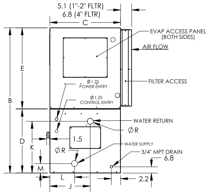
RIGHT VIEW
