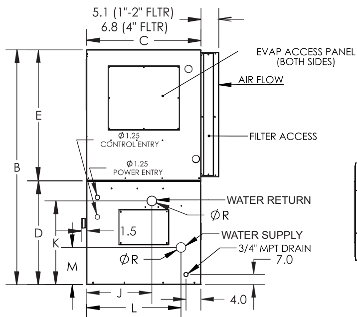
RIGHT VIEW
