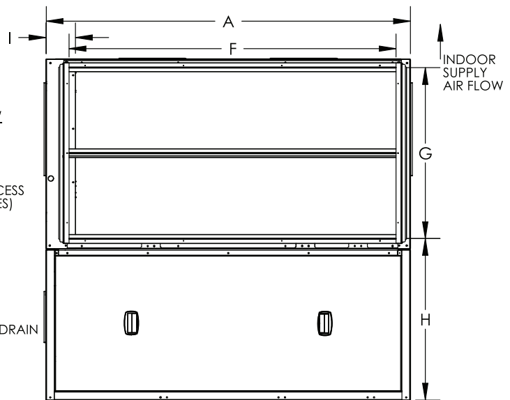
REAR VIEW
