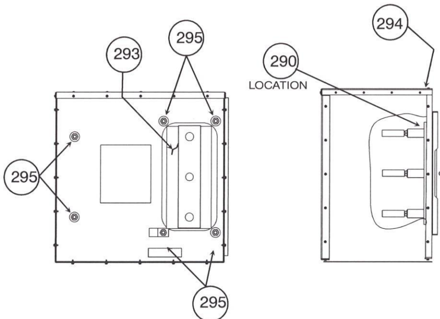
Compressor Terminal Box Assembly
