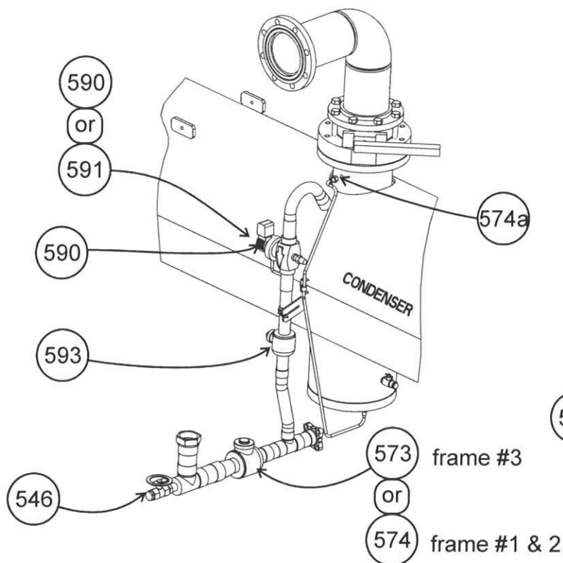
Machines w/Hot Gas Bypass
