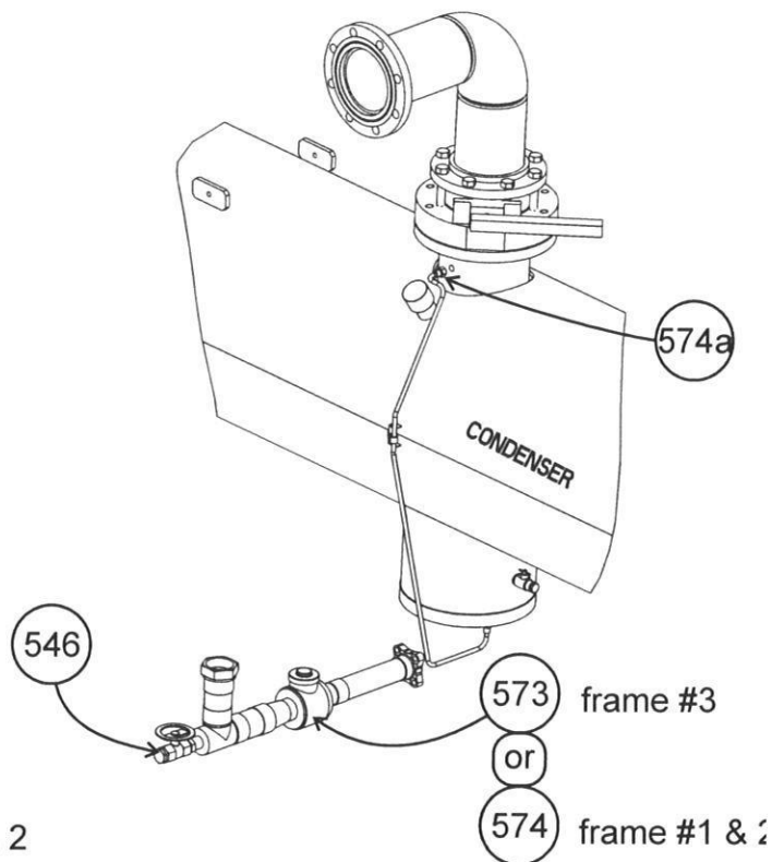
Machines w/out Hot Gas Bypass
