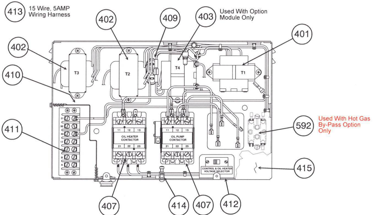
Power Panel For PIC I Machines
