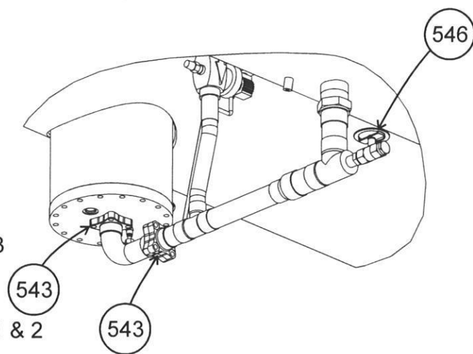
Machines w/out Cooler Isolation Valve
