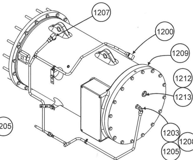
Motor Cooling Arrangement 02XR54016605
