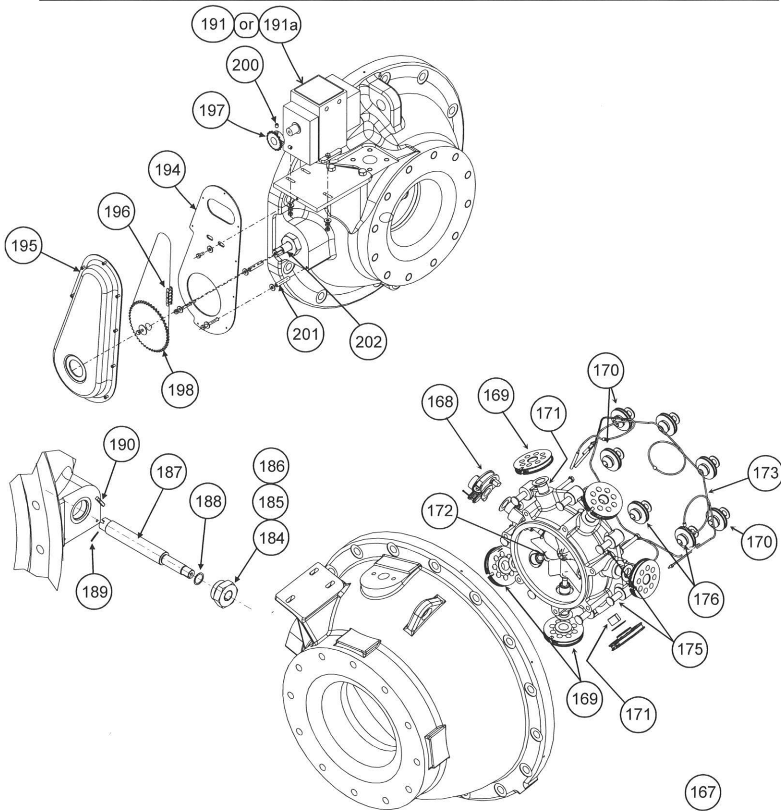
Blade Ring Assembly
