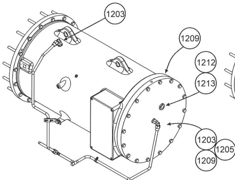
Motor Cooling Arrangement 02XR54016604 02XR54016606
