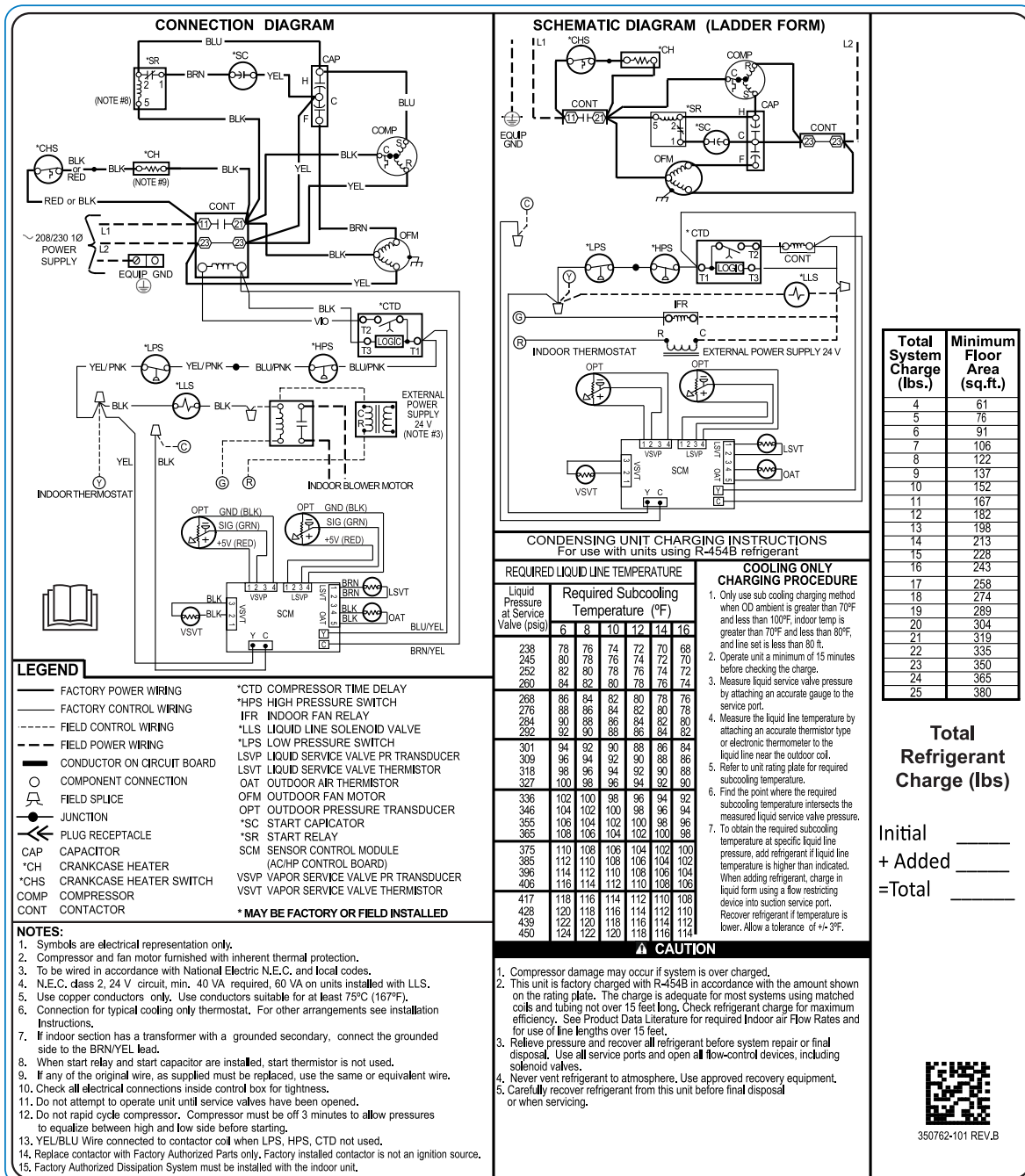
Fig. 1 – Size 1.5 - 5 Tons
