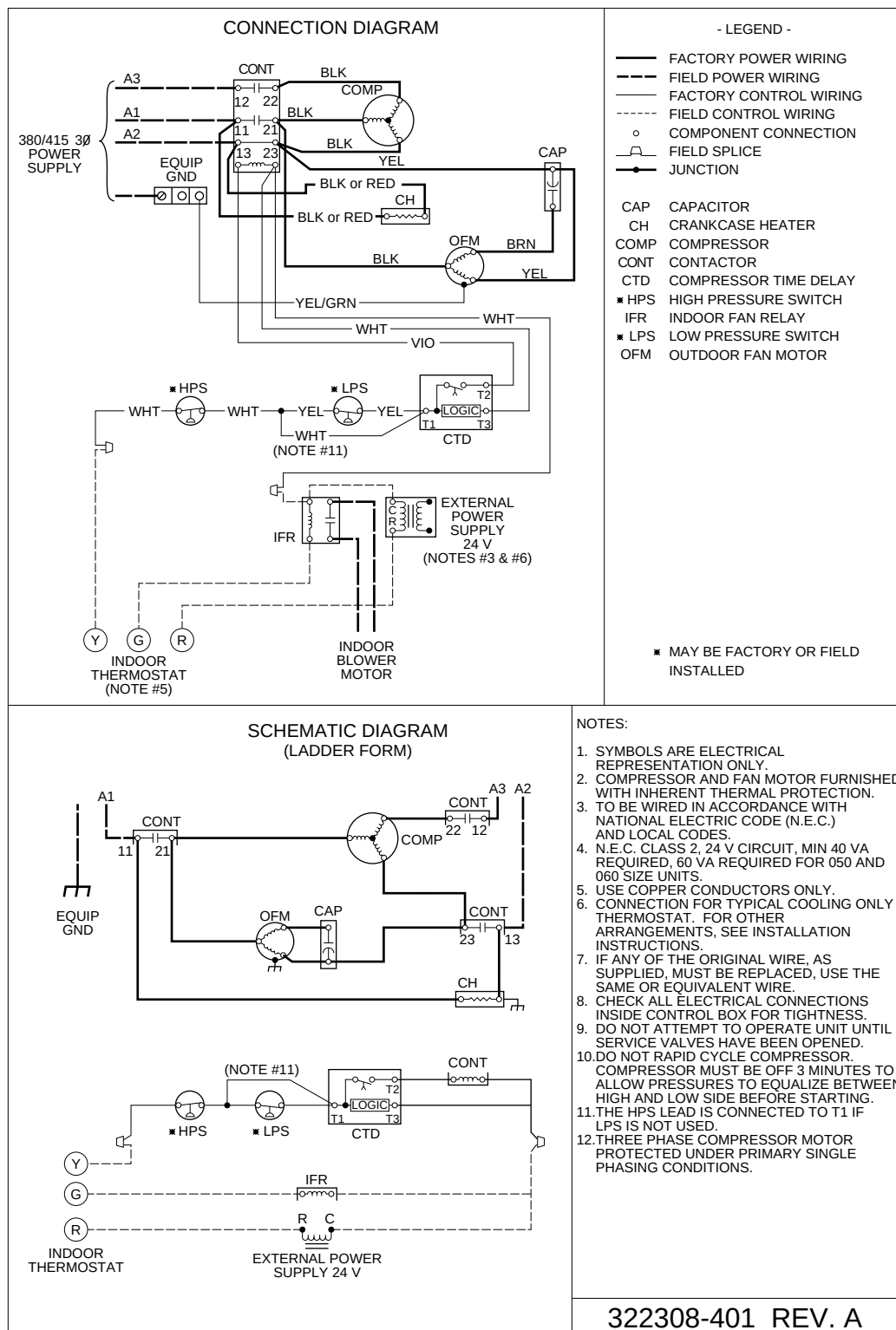
Fig. 2—38TUA036903/913, 048903/913, 060903 400v, 3 Phase, 50 Hertz
