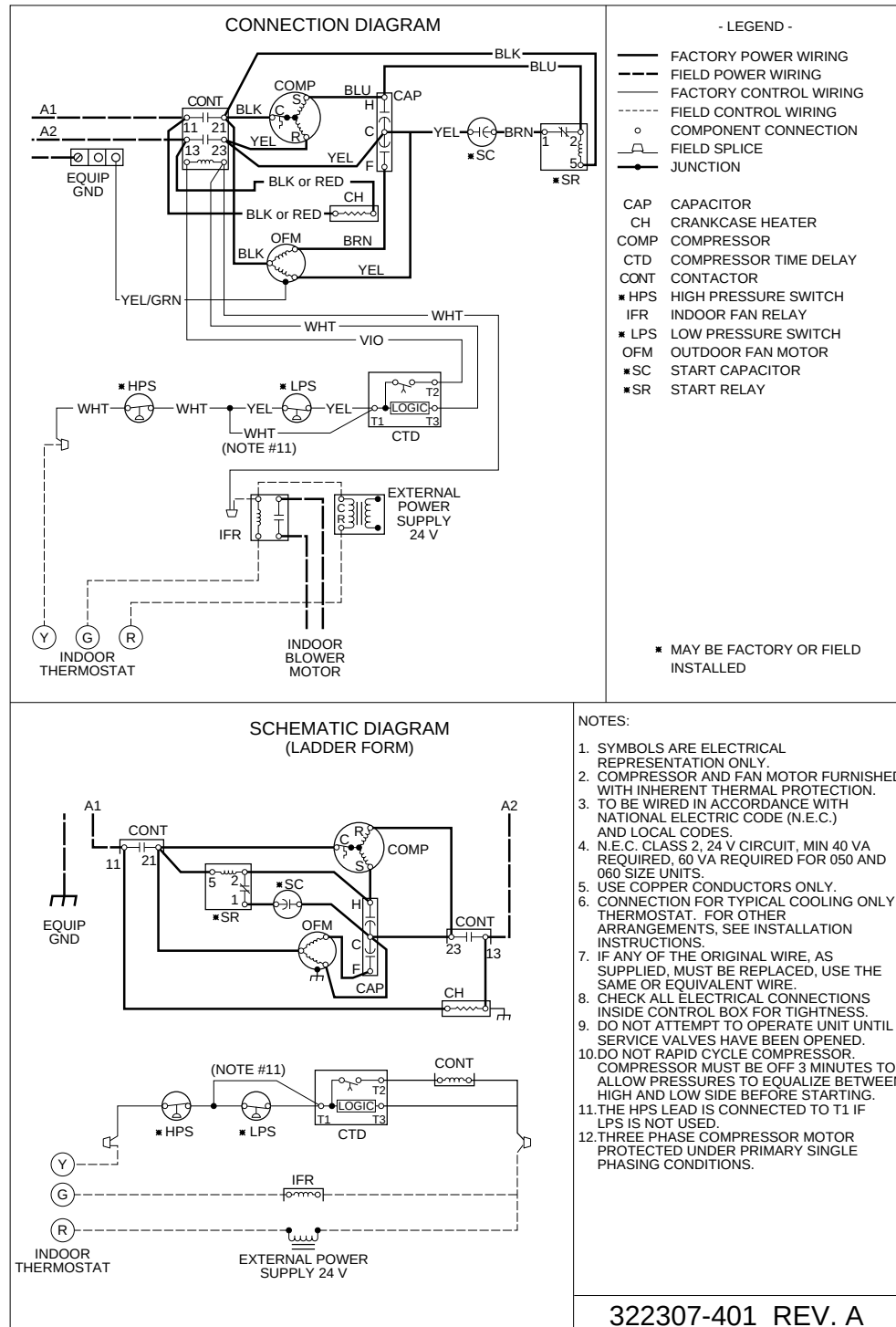
Fig. 1—38TUA024703, 036703/713, 048703/713 230v, 1 Phase, 50 Hertz
