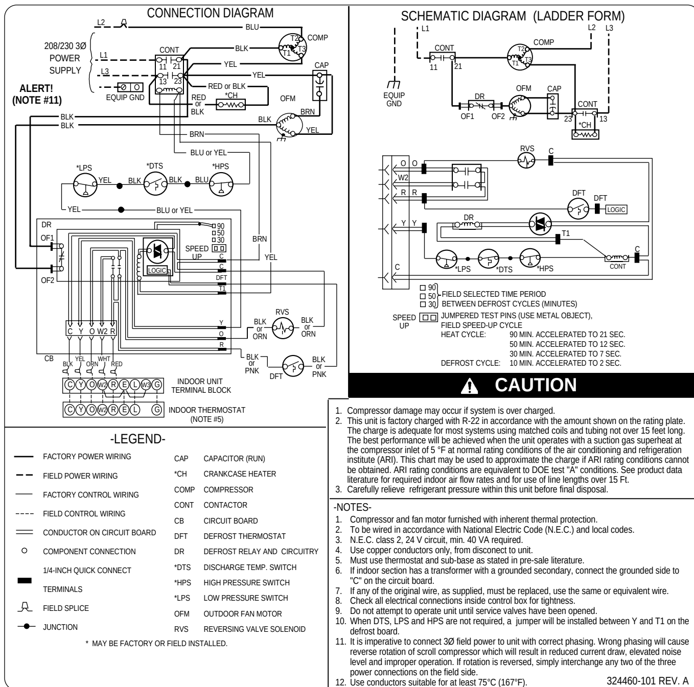
A97591 Fig. 4—38YC(C, W) 030 (50), 036 (50, 51, 52, 53), 042 (50, 51, 52, 53, 54), 048 (50, 51, 52), 060 (50, 51, 52) 208/230v, 3 Phase, 60 Hertz
