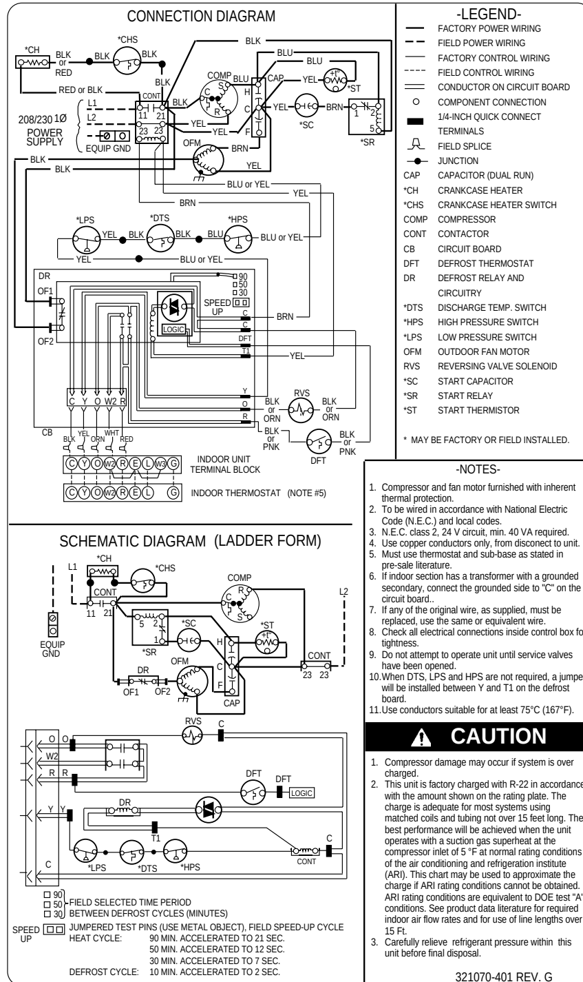
Fig. 1—38YC(C, G, S) 018 (30), 024 (30), 030 (30, 31), 036 (31, 32) 208-230v, 1 Phase, 60 Hertz
