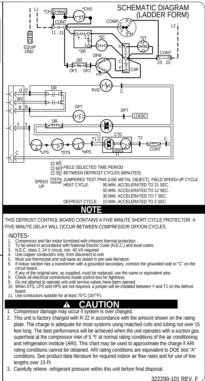
Fig. 2—38YC(C, G, S) 036 (30), 042 (30, 31, 32, 33), 048 (30, 31) and 38YCW018-048 208-230v, 1 Phase, 60 Hertz
