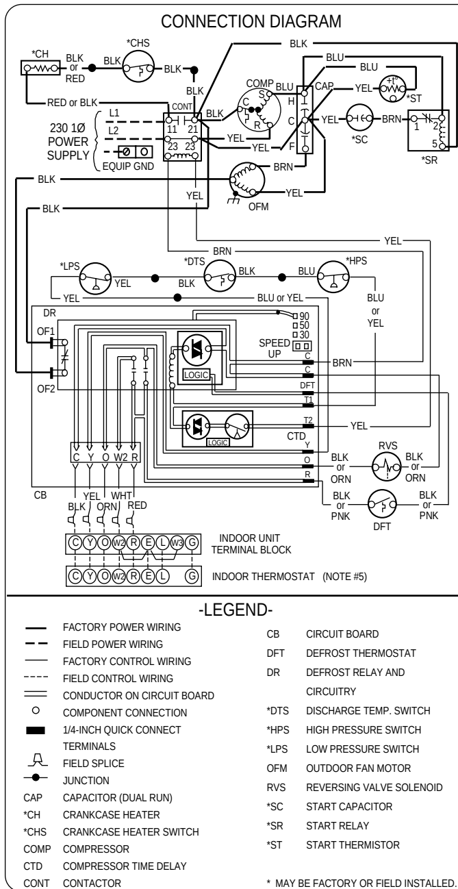
Fig. 2—38YC(C, G, S) 036 (30), 042 (30, 31, 32, 33), 048 (30, 31) and 38YCW018-048 208-230v, 1 Phase, 60 Hertz
