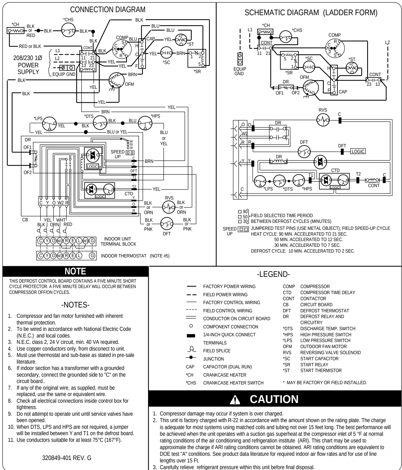
Fig. 3—38YC(C, G, S, W) 060 (30, 31) 208-230v, 1 Phase, 60 Hertz
