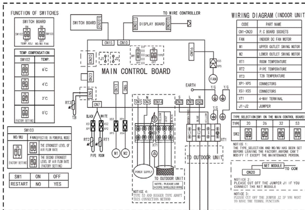
Fig. 6 – Wiring Diagram – Sizes 9 and 12
