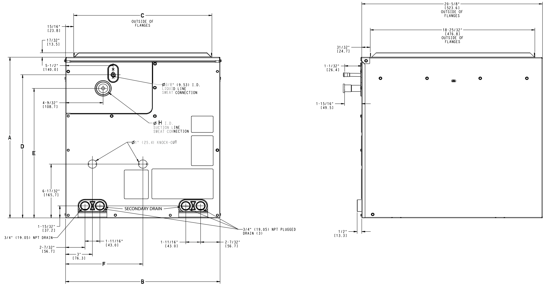
Fig. 8 – CVPVA (14" & 17" cabinet widths)
