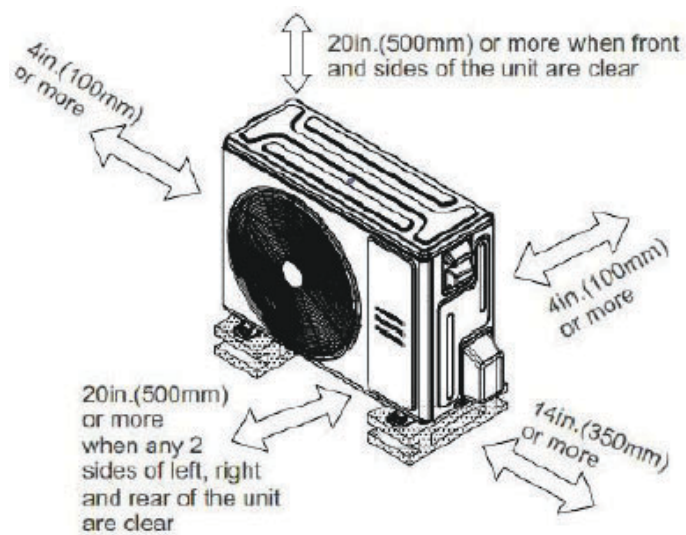
Fig. 6 – Clearances
