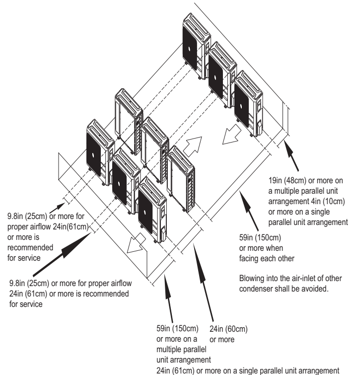
Fig. 7 – Multi-Unit Clearances
