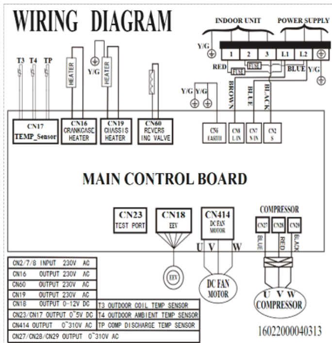
Fig. 10 – 18K/24K – 208/230V Wiring Diagram
