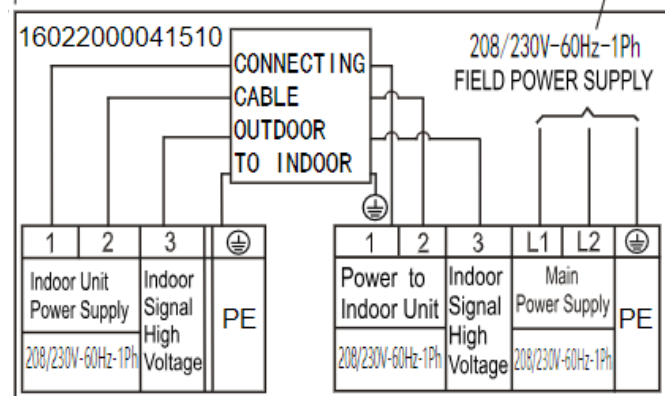
Fig. 7 – 9K/12K/18K/24K/30K/36K Connection Diagram
