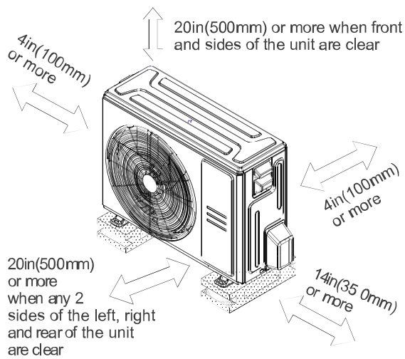
Fig. 5 – Clearances
