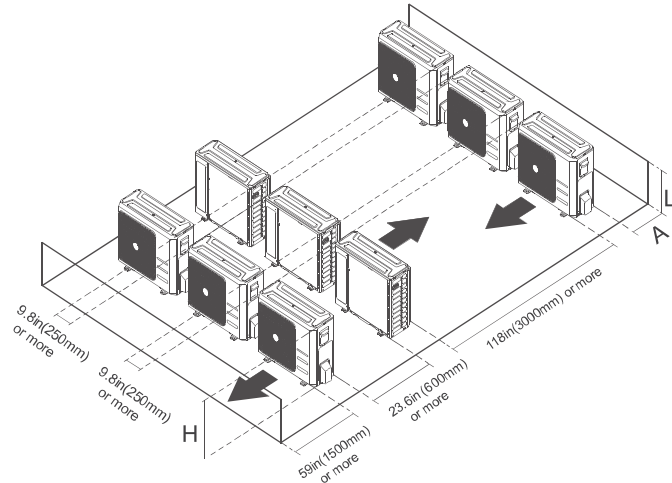
Fig. 6 – Clearances for multiple units
