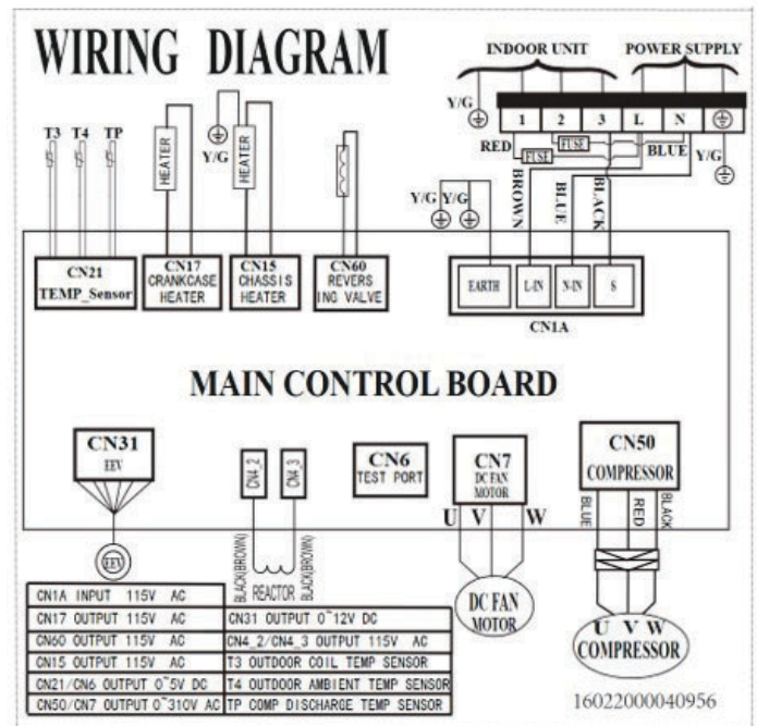
Fig. 8 – 12K – 115V Wiring Diagram
