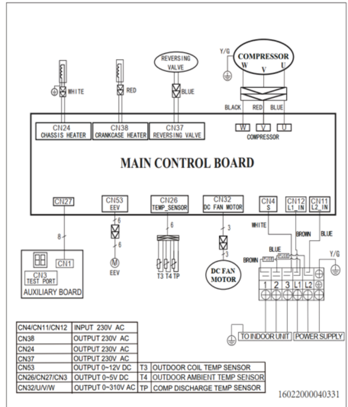
Fig. 11 – 30K – 208/230V Wiring Diagram
