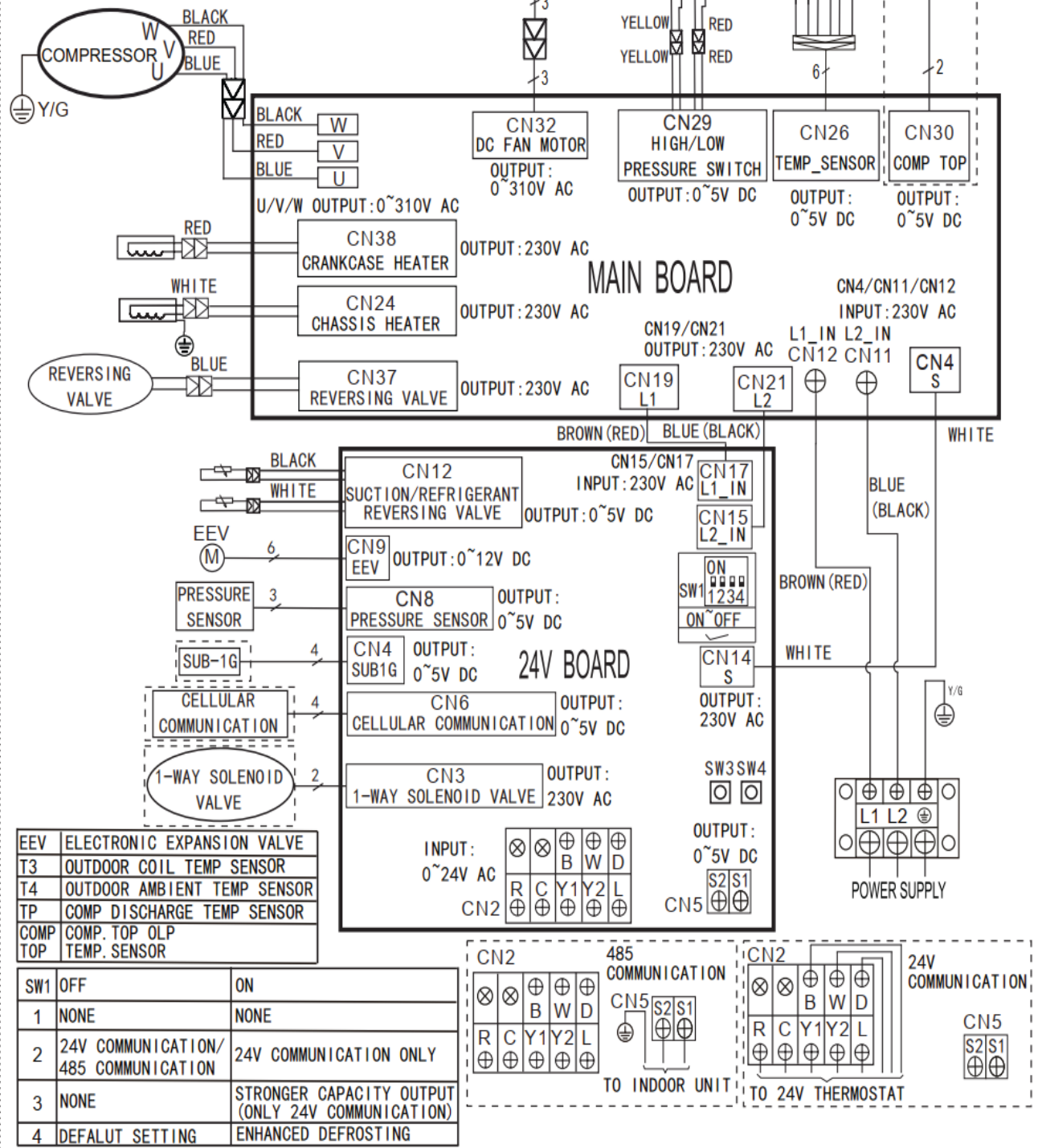
Fig. 38 — Wiring Diagram Size 30K
